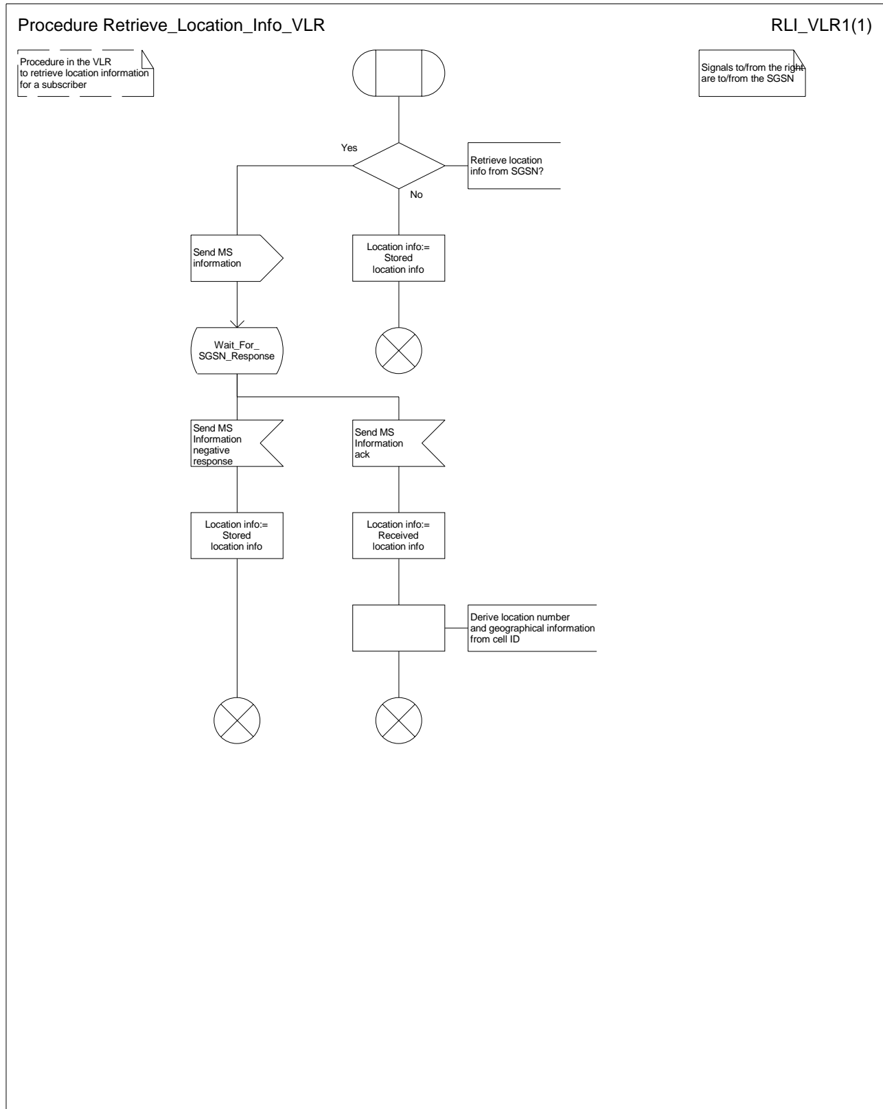
Figure 56c: Procedure Retrieve_Location_Info_VLR
