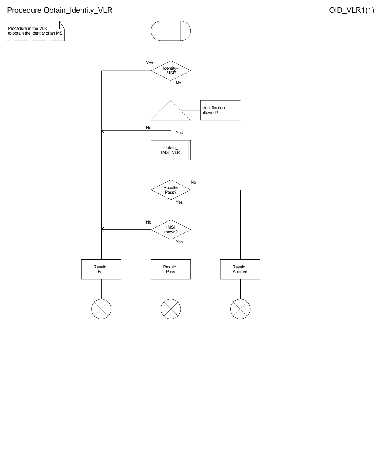
Figure 22: Procedure Obtain_Identity_VLR
