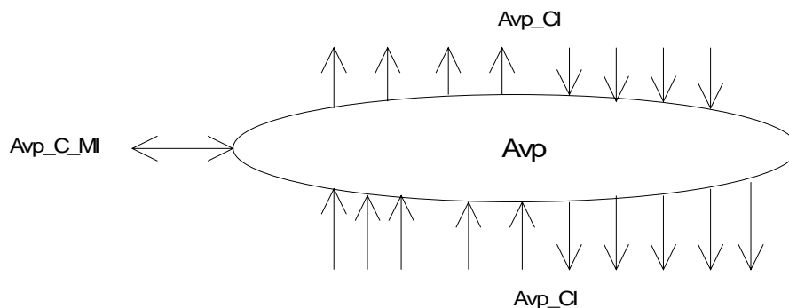
Figure 15: Avp_C symbol
