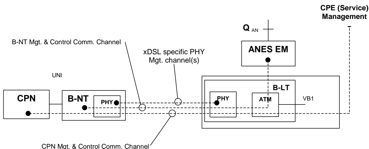
Figure 10: Extension and relevant termination functions of the B-NT and CPN Management & Control Communication Channels, and XDSL specific Physical Layer management channel(s)
