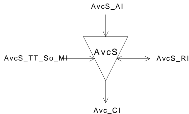
Figure 33: AvcS_TT_So symbol
