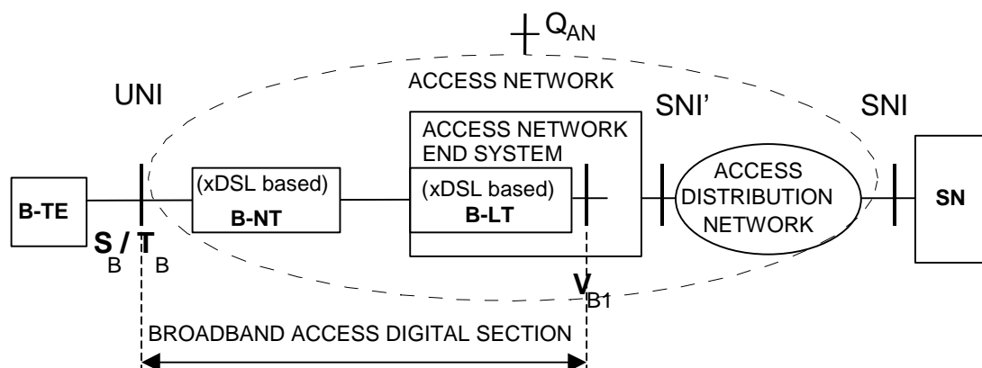
Figure 1: xDSL based ATM Access Digital Section supporting a single ATM interface at UNI
