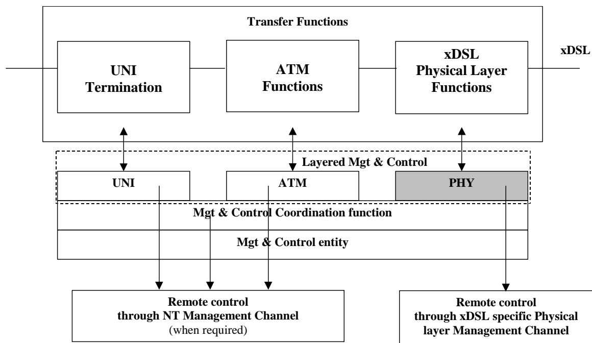
Figure 9: B-NT Management & Control Architecture
