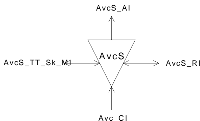
Figure 34: AvcS_TT_Sk symbol
