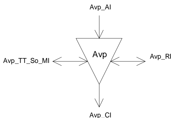
Figure 16: Avp_TT_So symbol
