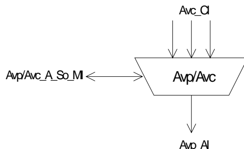
Figure 26: Avp/Avc_A_So symbol
