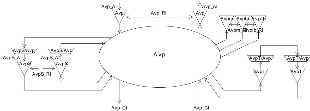
Figure 14: ATM Virtual Path layer network atomic functions
