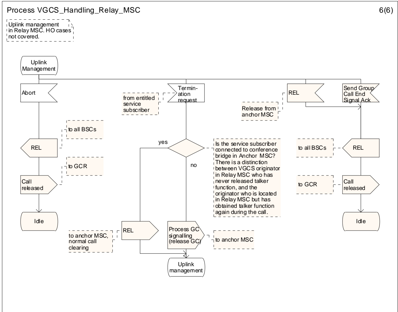
Figure 10: The VGCS handling process in the relay MSC (sheet 6 of 6)
