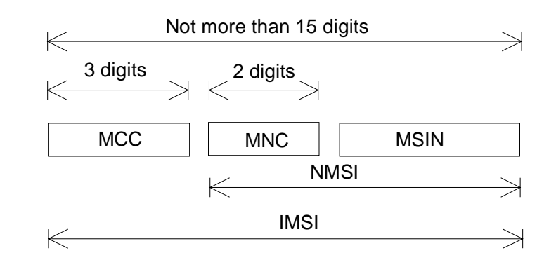
Figure 1: Structure of IMSI
