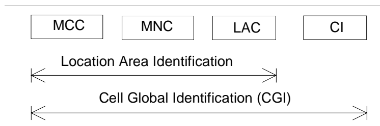
Figure 5: Structure of Cell Global Identification
