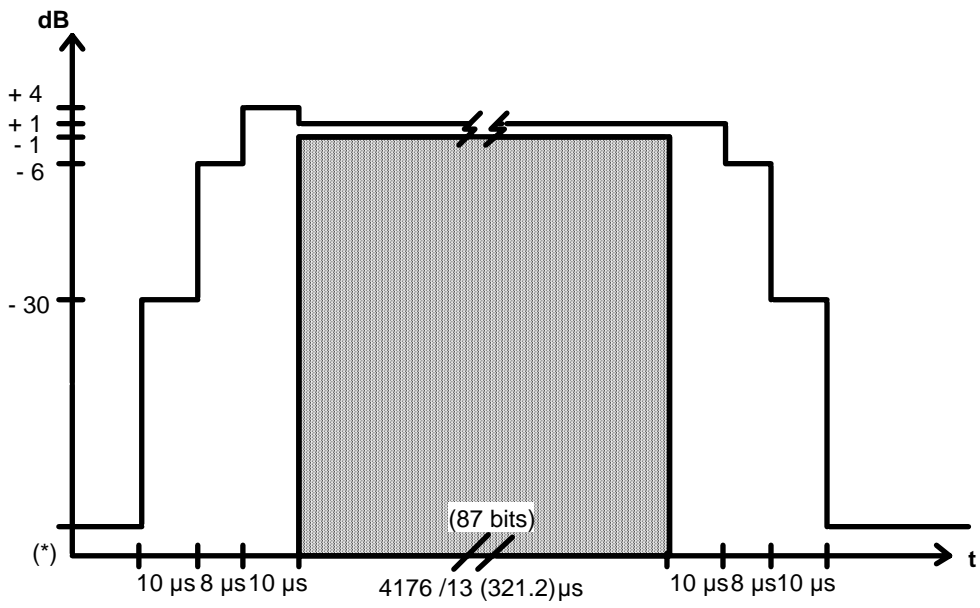
PCS 1 900 MS Access Burst Time Mask
