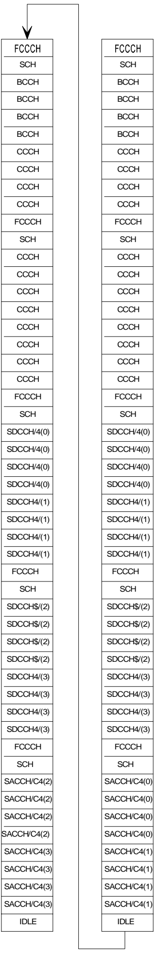
Figure 8b: TDMA frame mapping for FCCH + SCH + BCCH + CCCH + SDCCH/4(0...3) + SACCH/4(0...3)
