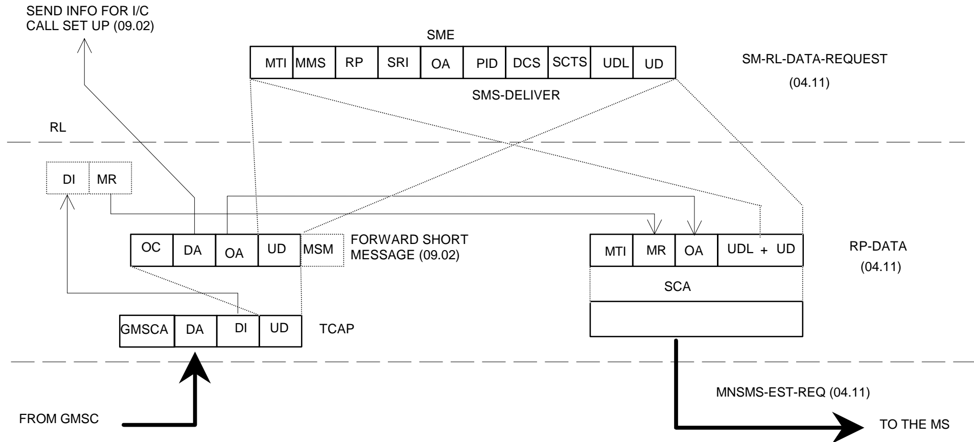
Figure 1.3: Mobile terminated short message
