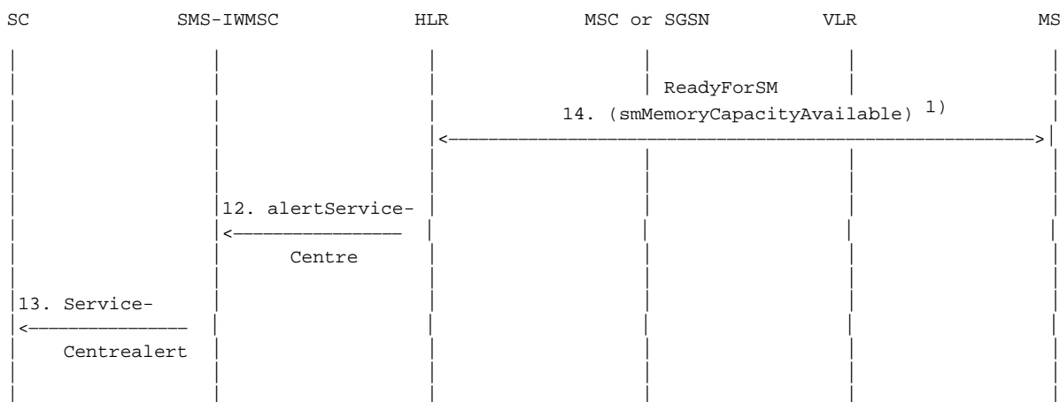
Figure 03.40/20b: The alert procedure when the MS becomes reachable, MNR, MNRG or both are set and MCEF is set
