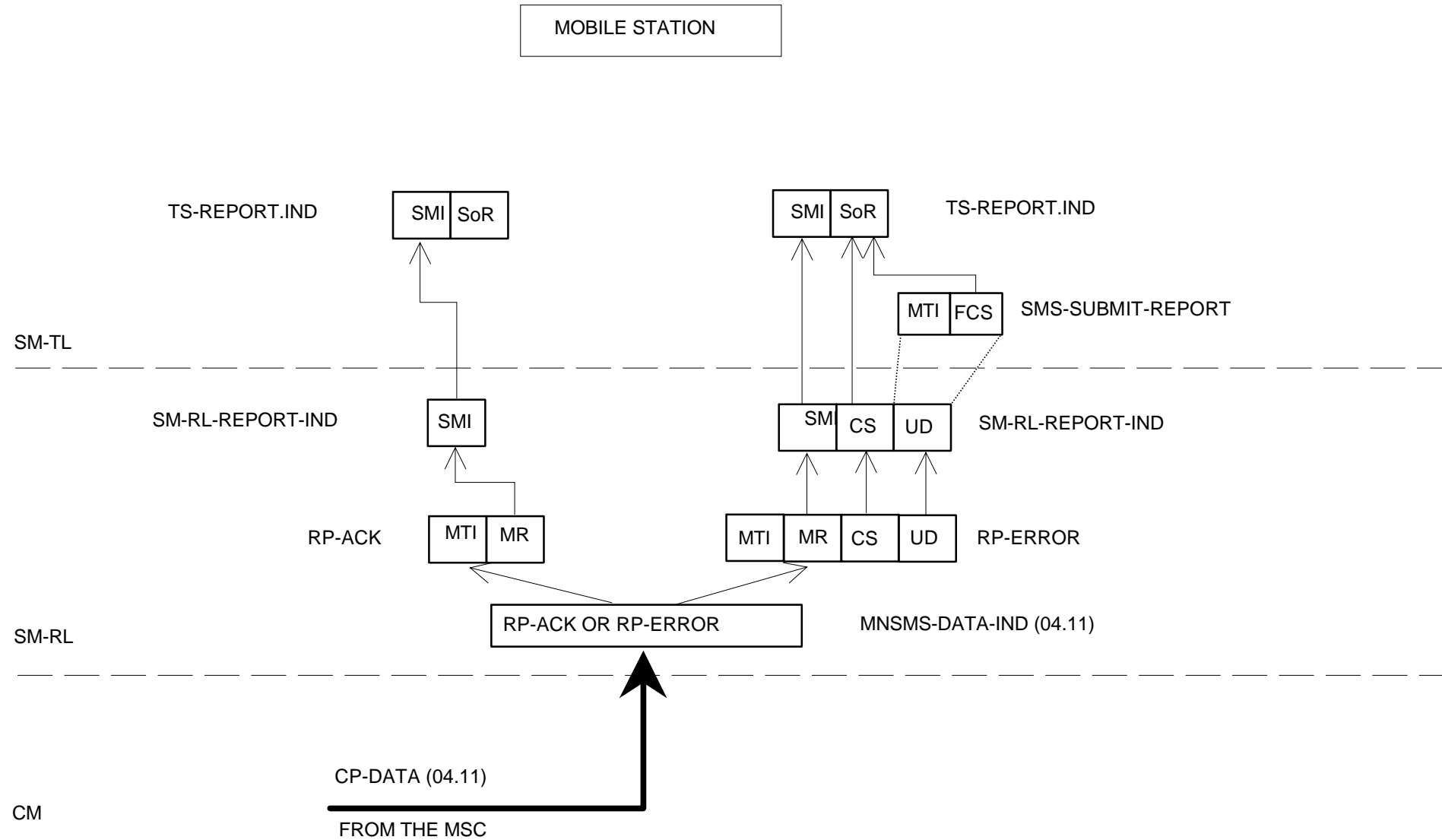
Figure 4.3: Acknowledgement in the MO case
