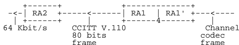
Figure 4.2: Rate adaption when performed at the BTS
