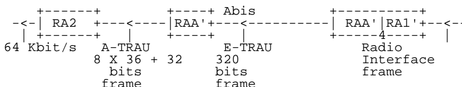
Figure 4.3.1: Rate adaption when 16 kbit/s traffic channels are used
