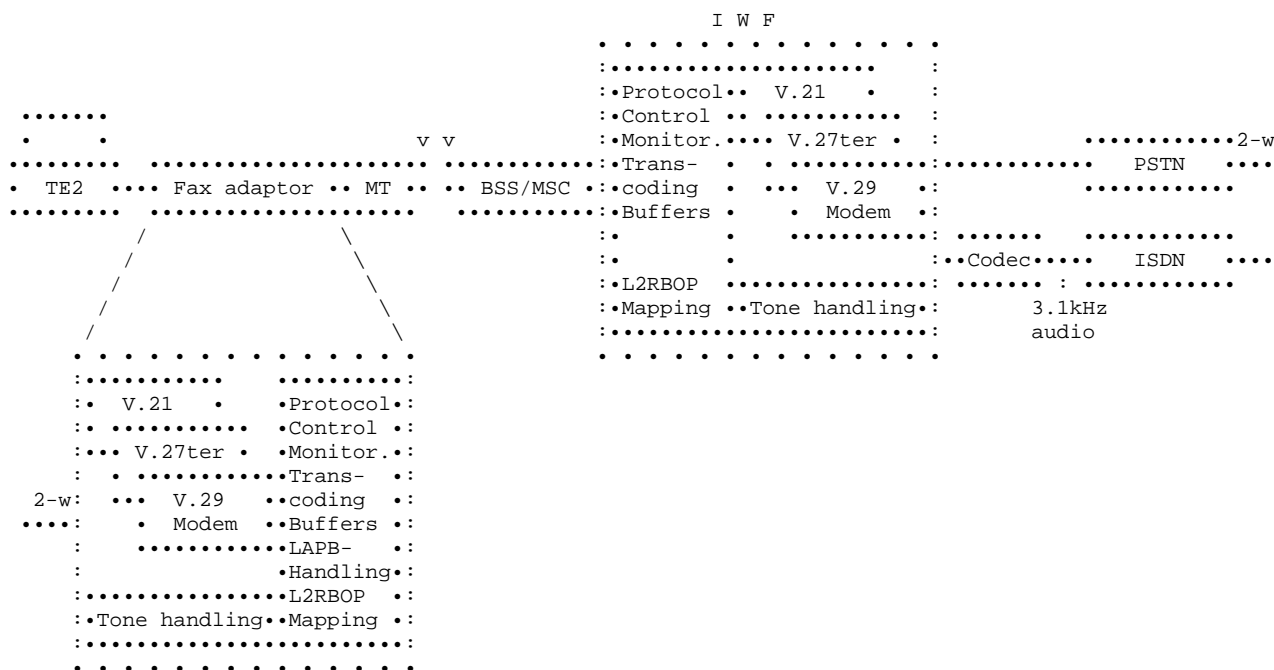
Figure 7/03.46: Network interworking
