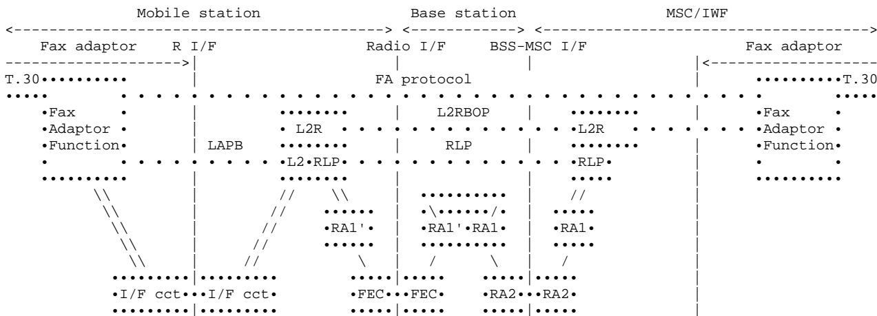
Figure 5/03.46: Protocol model for non-transparent support
