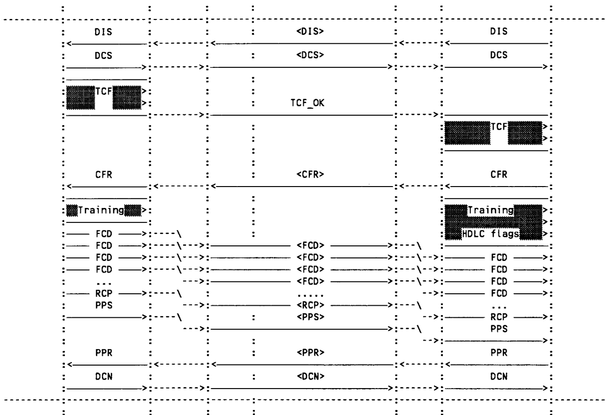
Figure II.8/03.46: Mobile originated facsimile transmission (error correction mode)
