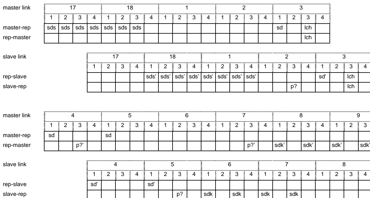
Figure 7: Call sequence for SDS (for acknowledgement without data) through type 1 DM-REP
