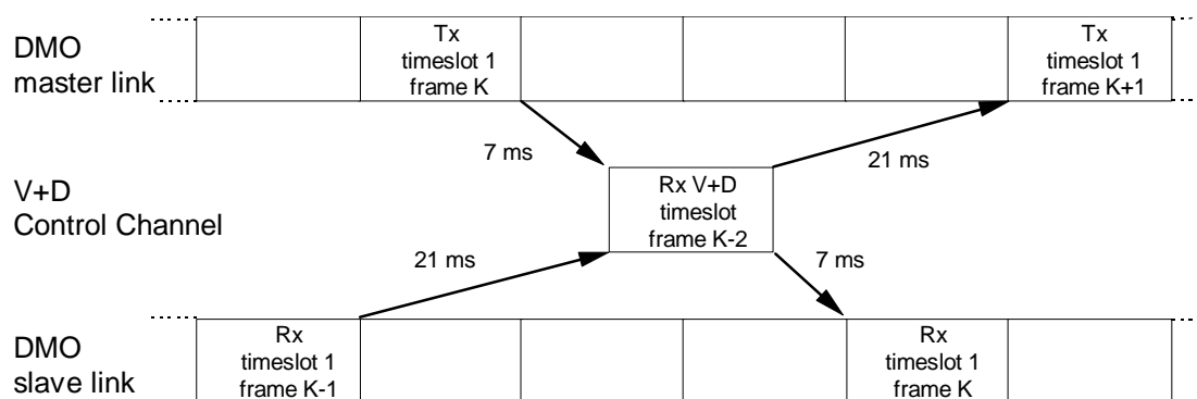
Figure 8: Dual watch timing on type 1 DM-REP
