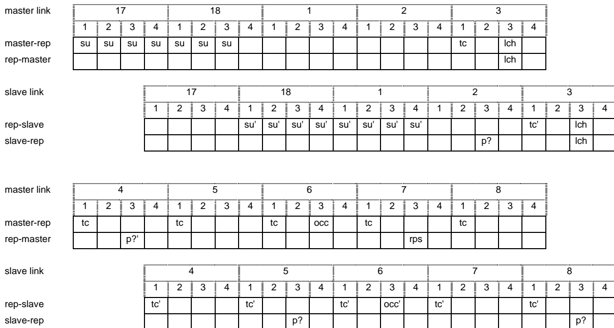
Figure 2: Call sequence for set-up without presence check through type 1 DM-REP
