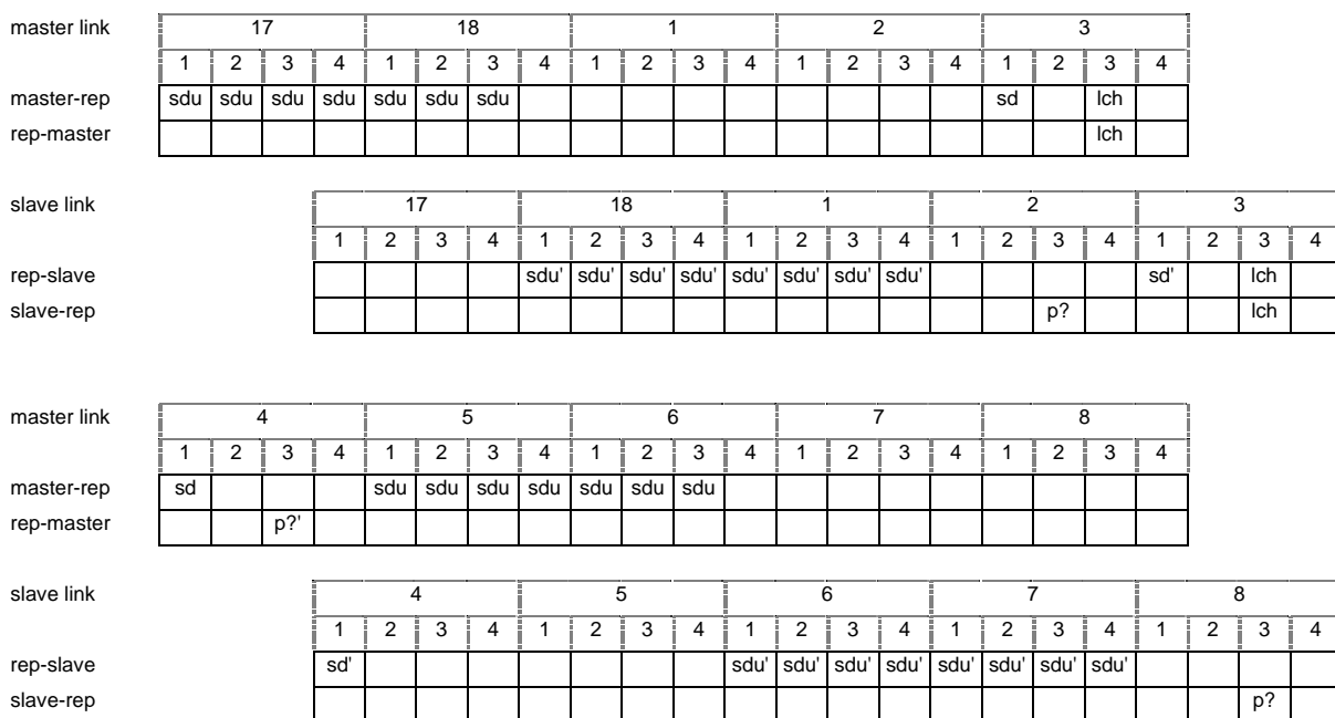
Figure 6: Call sequence for SDS (for unacknowledged data) through type 1 DM-REP
