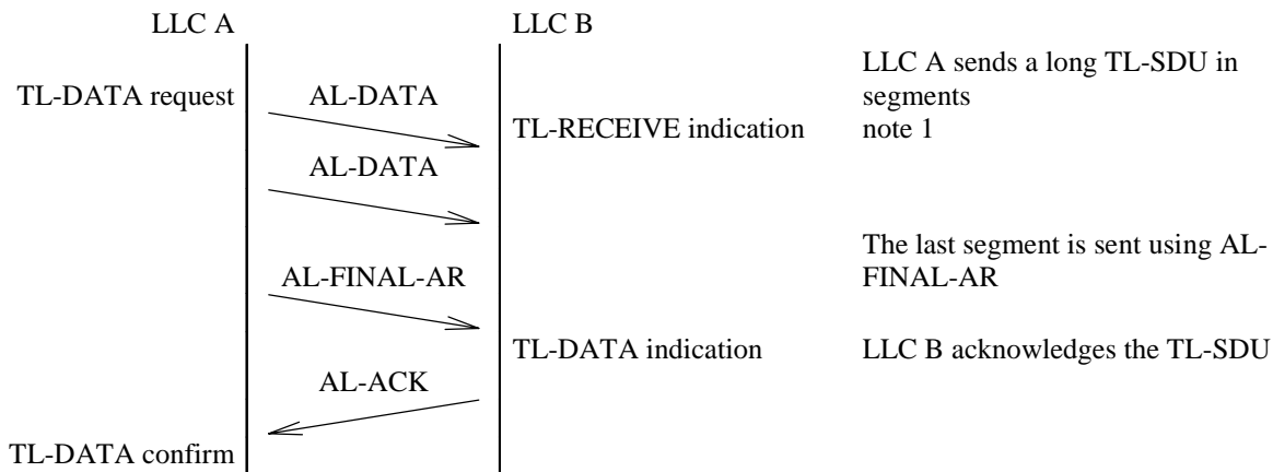
Figure 122: PDU exchange in a unidirectional transfer
