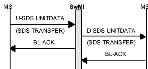
Figure 218: Layer 2 Acknowledgement
