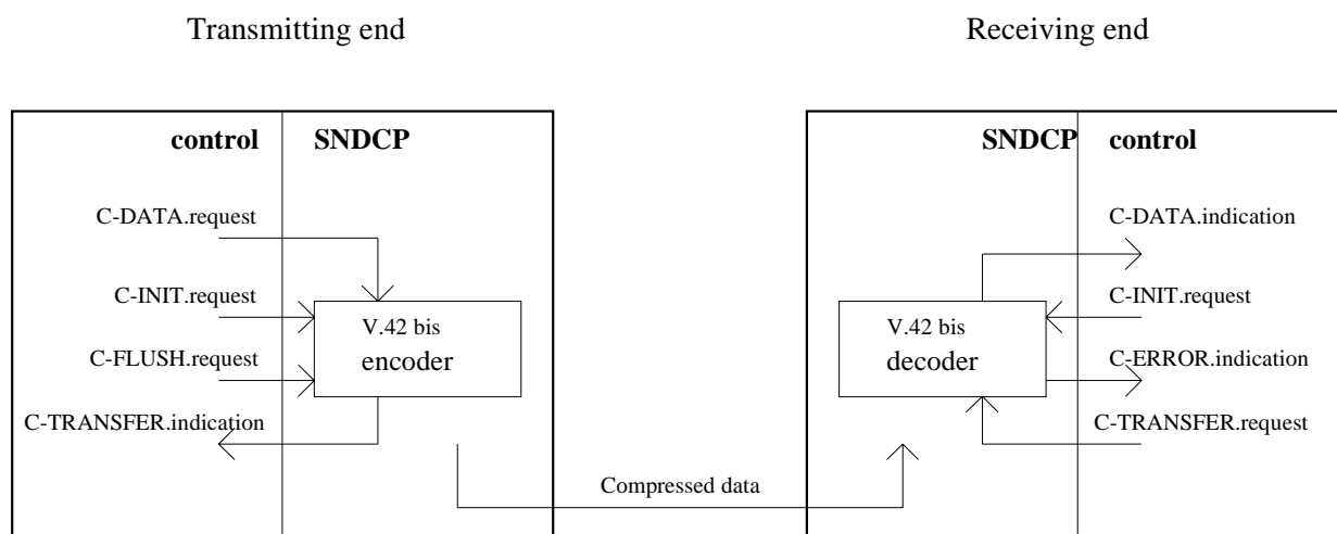
Figure 212: ITU-T Recommendation V.42bis data compression function
