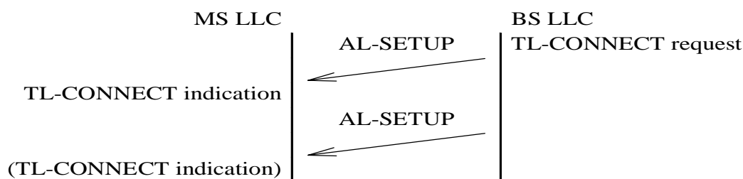
Figure 120: Unacknowledged transfer mode set-up of the advanced link
