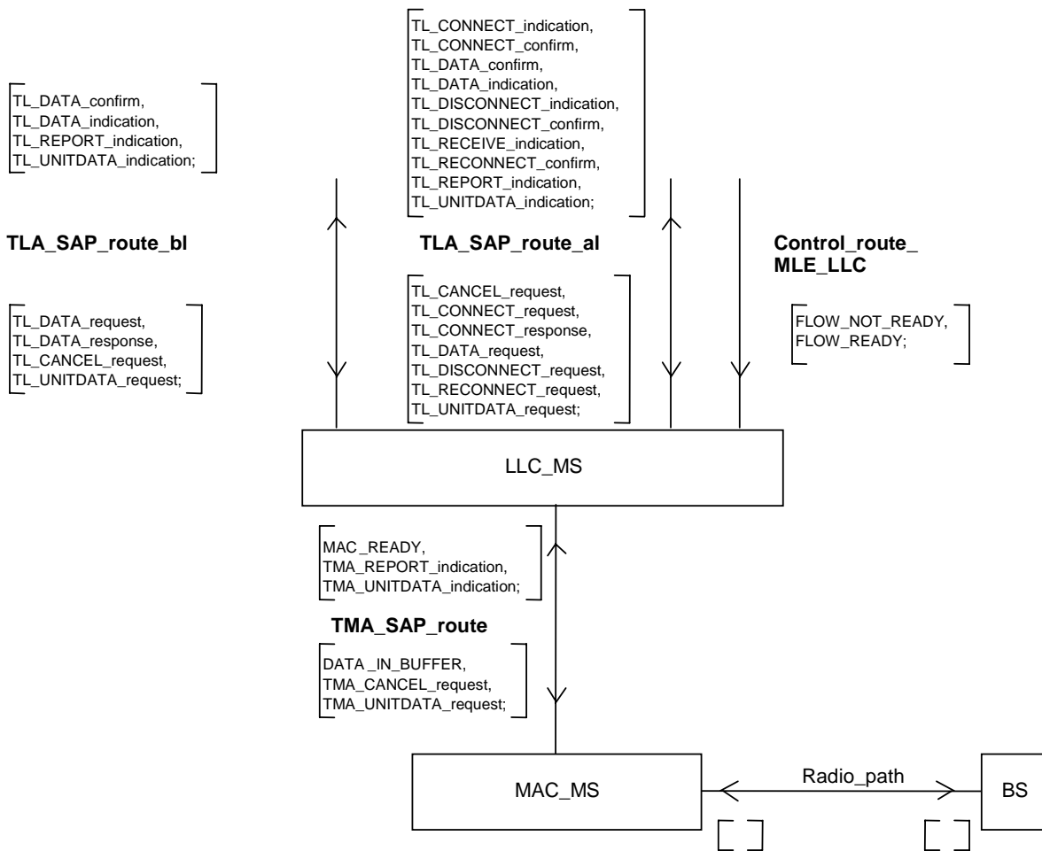
Figure 101: LLC relations
