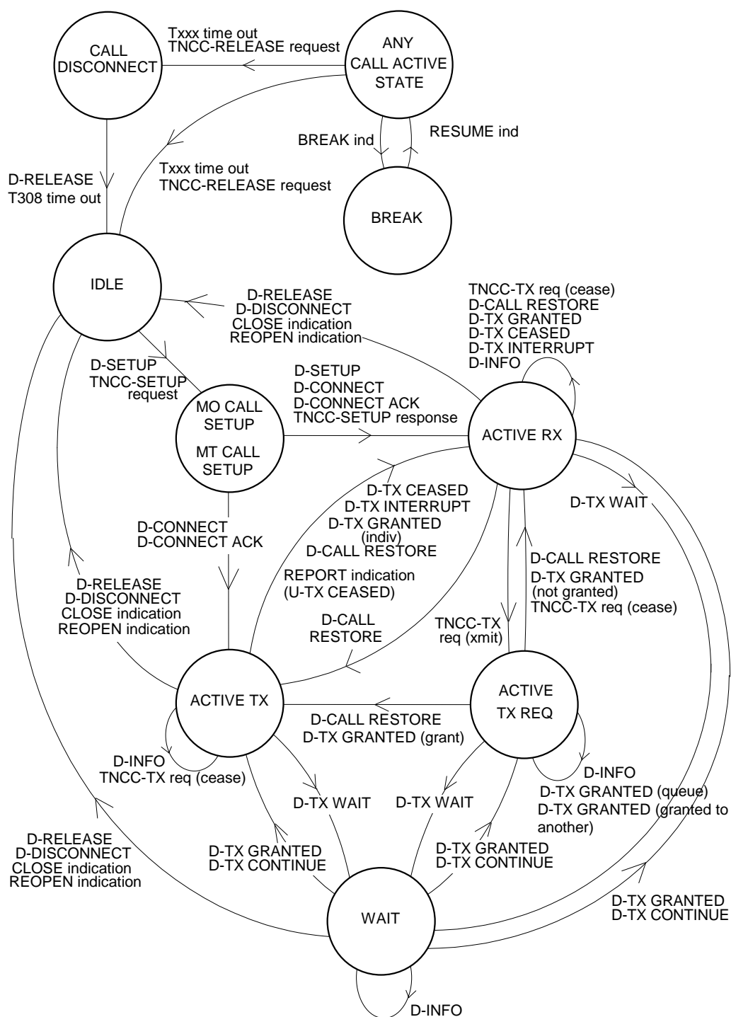
Figure 22: Sub state transition diagram for the CALL-ACTIVE state
