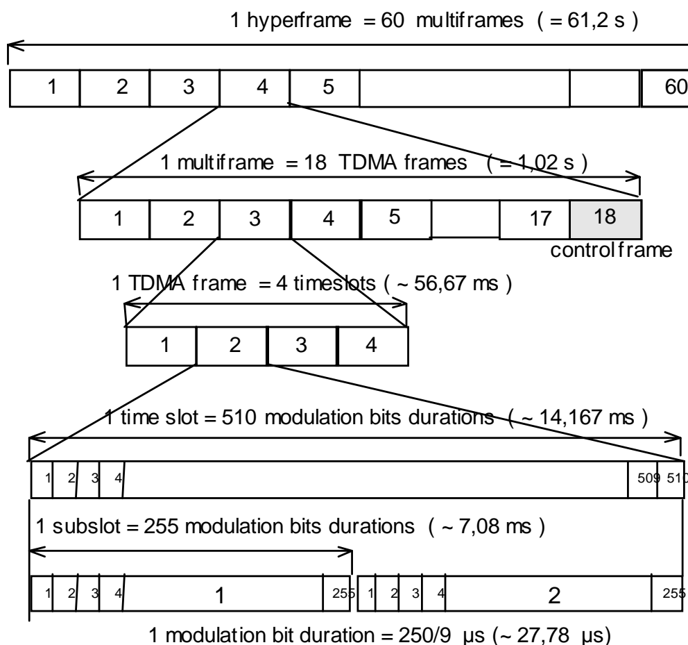
Figure 11: TDMA structure
