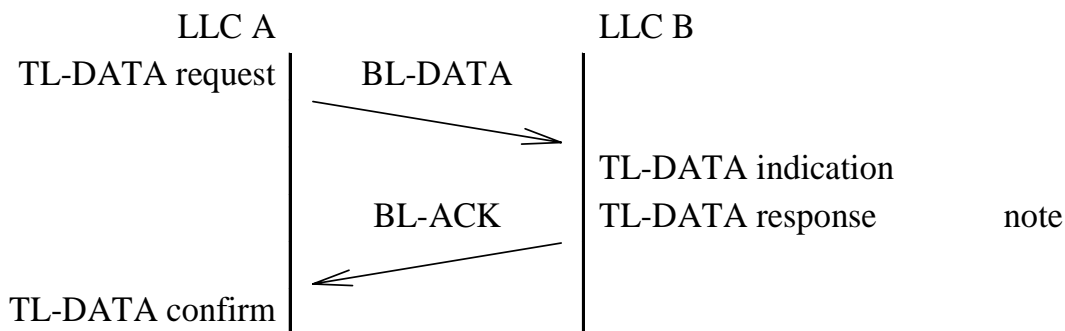
Figure 103: Basic link PDU exchange with acknowledgement carrying a layer 3 message
