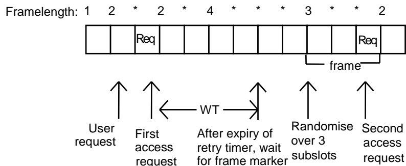
Figure 144: Example of random access procedure (BS using rolling access frames)
