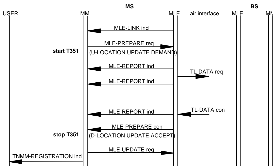
Figure 49: MLE initiated forward registration
