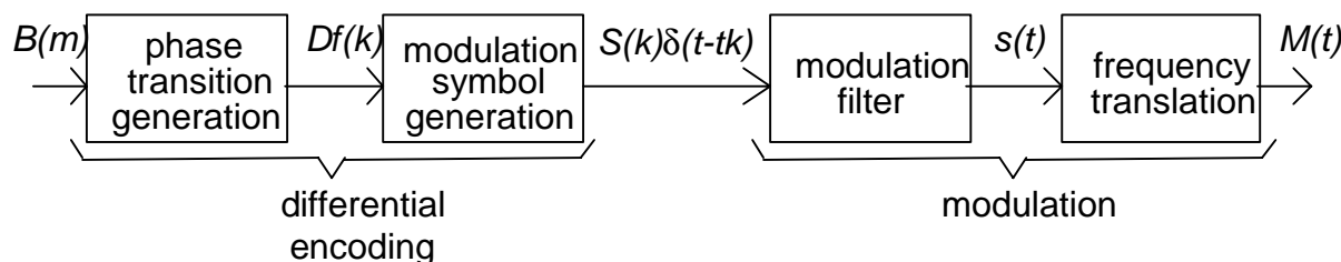
Figure 4: Block diagram of the modulation process
