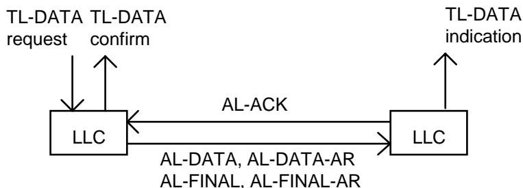
Figure 122: PDU exchange in a unidirectional transfer
