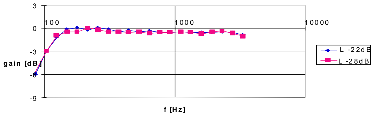
Figure 13: GSM EFR codec frequency response at different input levels
