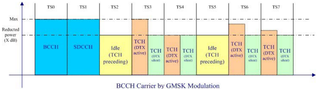
Figure 7.2-2: BCCH Carrier Power Reduction Method; Variant 2
