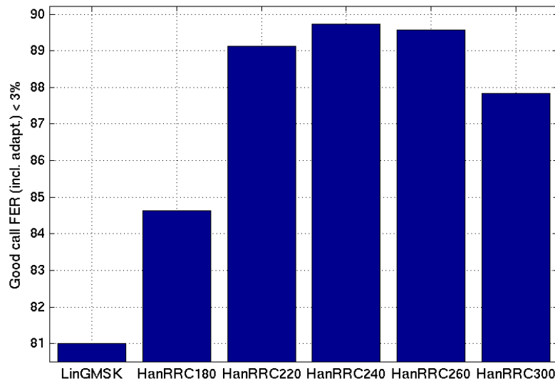
Figure 8-69e. Impact on performance from different TX pulse shapes on users in VAMOS mode, MS penetration scenario I.
