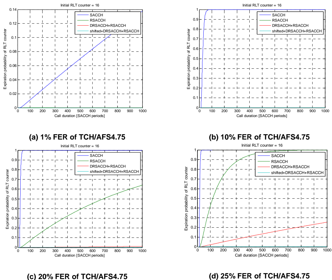
Fig. 11.3-22: Expiration probability of RLT counter vs call duration with initial RLT counter being 16 (TCH/AFS4.75).
