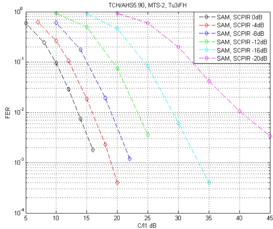
Figure 8-60f - Performance of SAM in MTS-2, AHS5.90 for varying SCPIR
