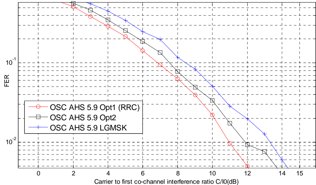
Figure 7-16a: Link Performance for investigated TX pulse shapes for OSC channels, CCI, DIR=7dB, TU3iFH GSM900.
