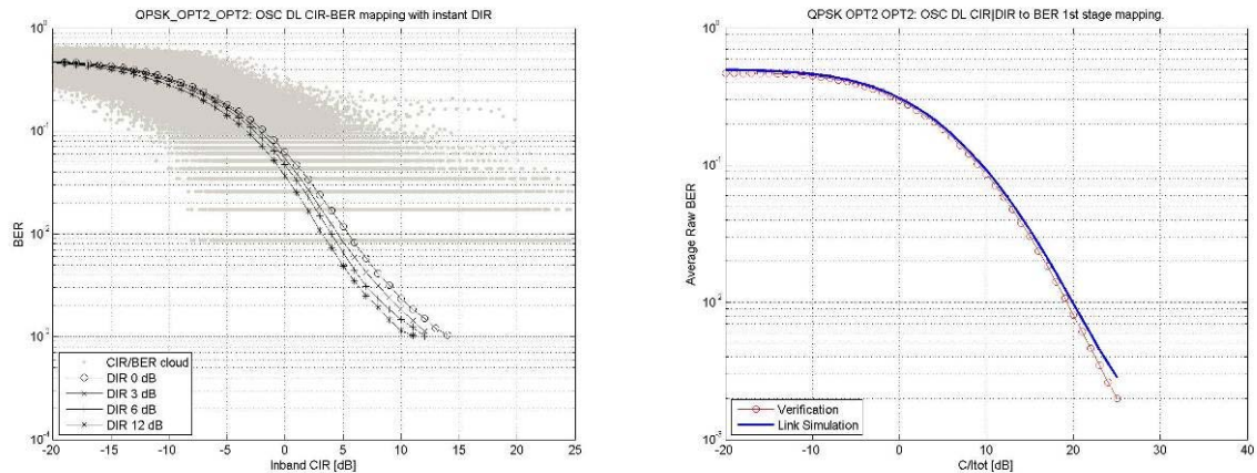
Figure 39-I. Mapping and verification for a QPSK modulated carrier
