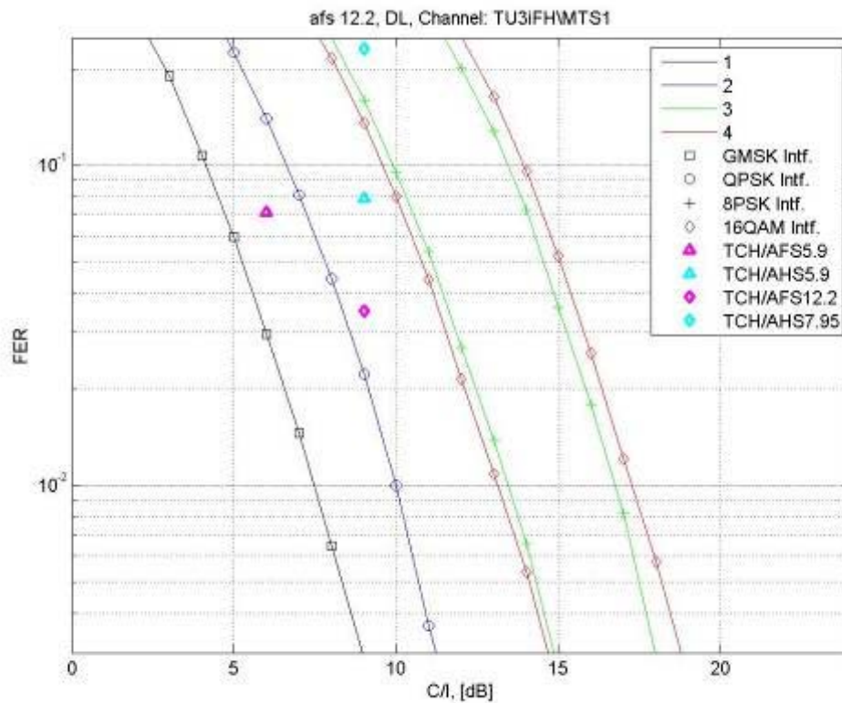
Figure 9-26: AMR 12.2 multiplexed users in DL, MTS-1/TU3iFH
