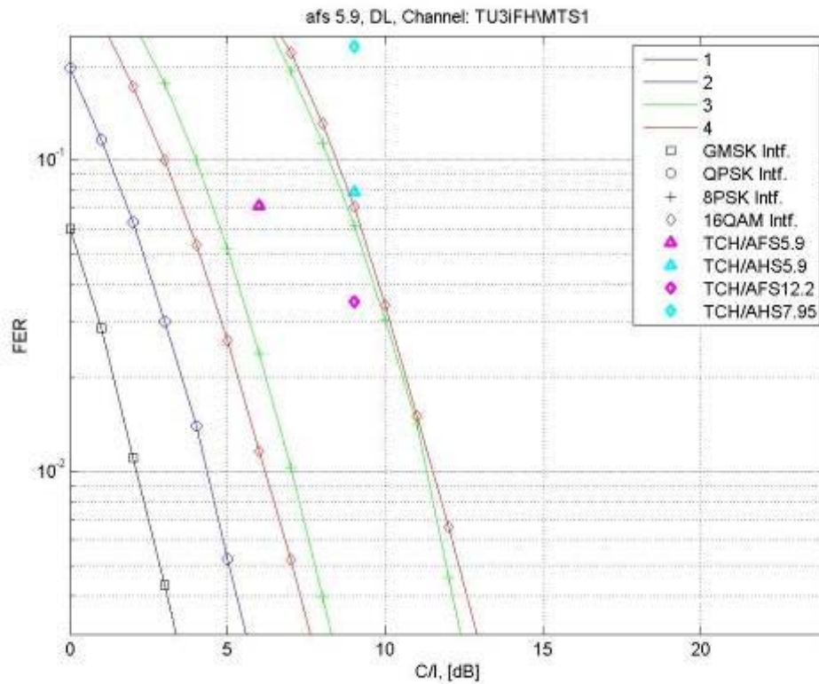
Figure 9-25: AMR 5.9 multiplexed users in DL, MTS-1/TU3iFH
