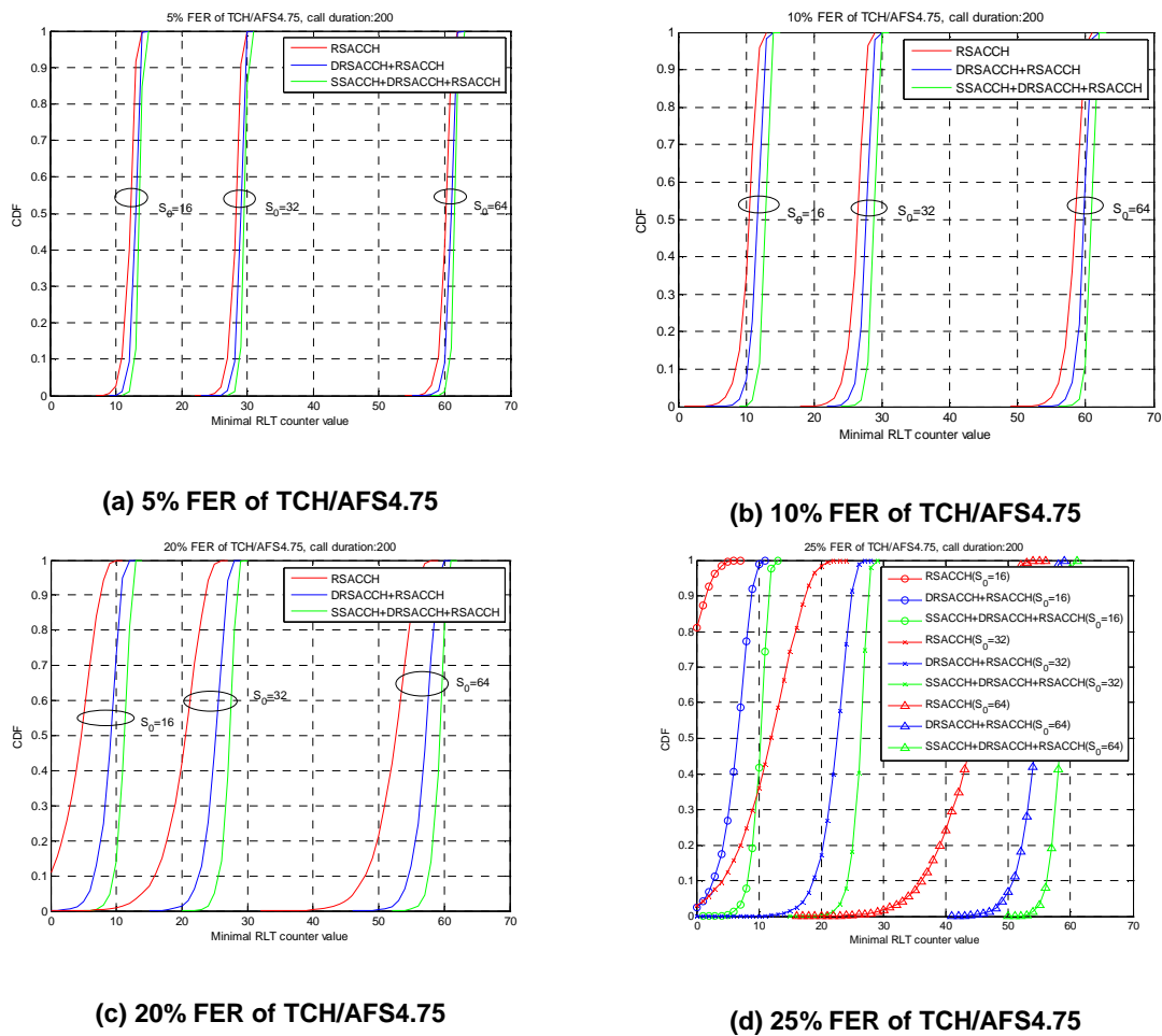
Fig. 11.3-28: CDF of minimal RLT counter values (TCH/AFS4.75, call duration: 200 SACCH periods).
