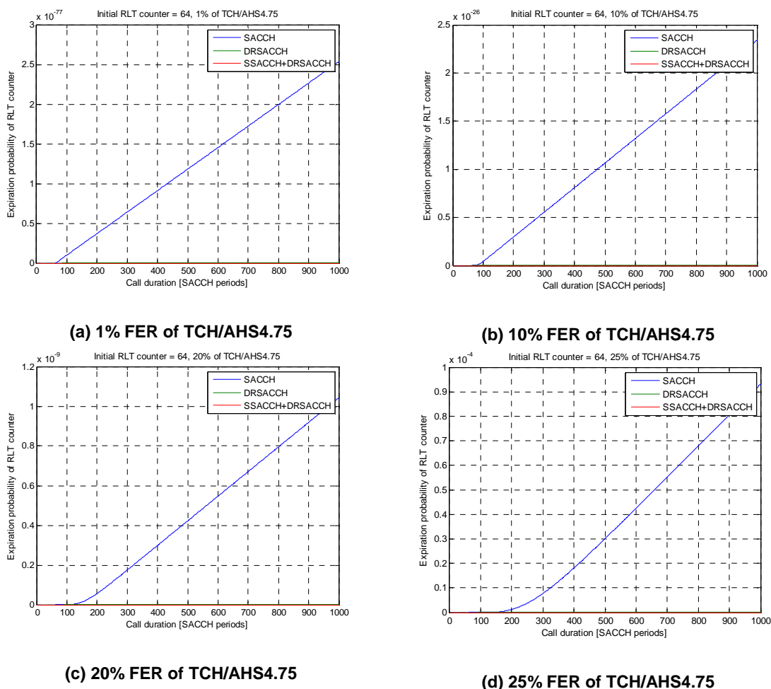
Fig. 11.3-27 Expiration probability of RLT counter vs call duration with initial RLT counter being 64 (TCH/AHS4.75).
