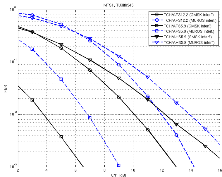
Figure 7-27: DL Co-channel interference performance (MTS1) of a legacy DARP MS receiving a MUROS sub channel using AMR half rate 5.9, AMR full rate 12.2 and AMR full rate 5.9
