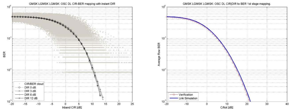
Figure 39-m. Mapping and verification for a GMSK modulated carrier
