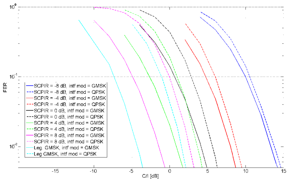
Figure 8-31: MTS-3, TU3iFH
