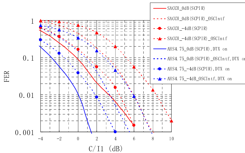
Figure 11-21: SACCH and TCH performance without shifted SACCH, DTX on
