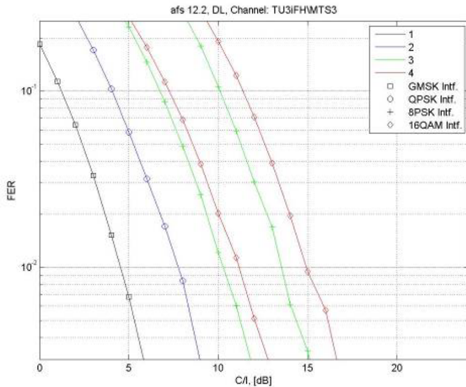
Figure 9-30: AMR 12.2 multiplexed users in DL, MTS-3/TU3iFH
