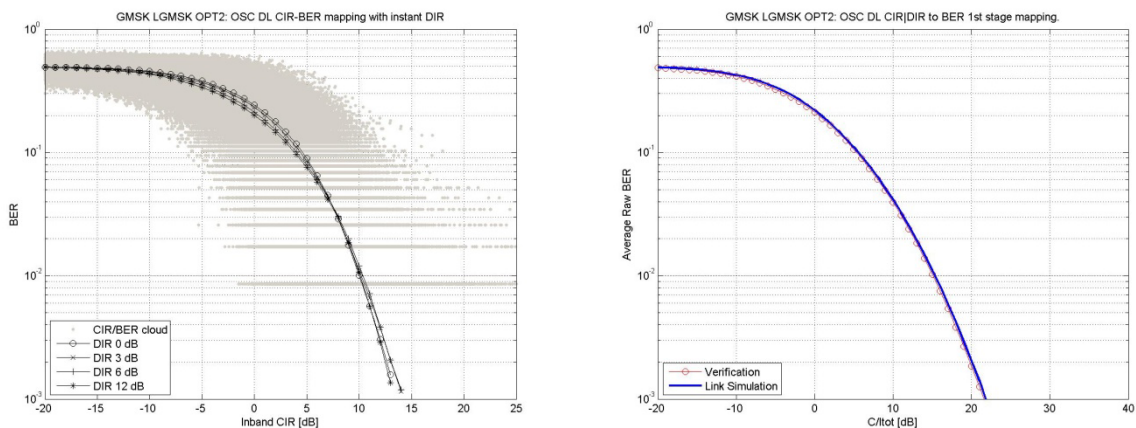
Figure 39-o. Mapping and verification for a GMSK modulated carrier
