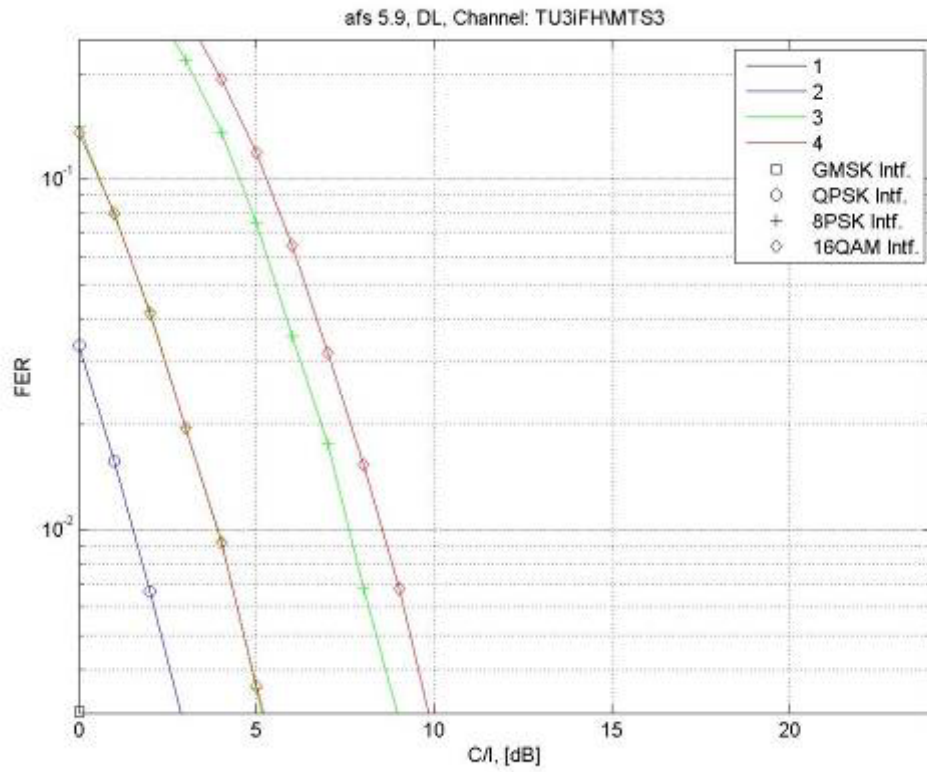
Figure 9-29: AMR 5.9 multiplexed users in DL, MTS-3/TU3iFH
