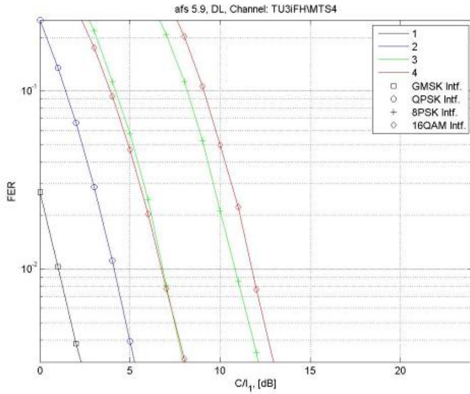
Figure 9-31: AMR 5.9 multiplexed users in DL, MTS-4/TU3iFH
