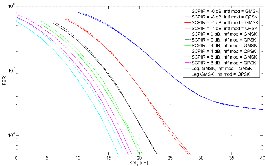
Figure 8-40: MTS-4, TU3nFH
