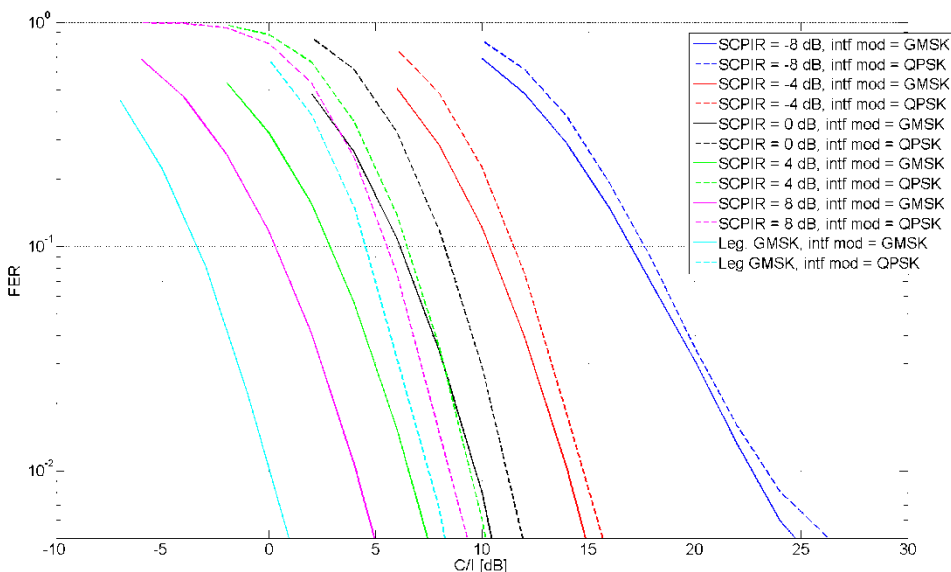
Figure 8-25: MTS-1, TU3iFH
