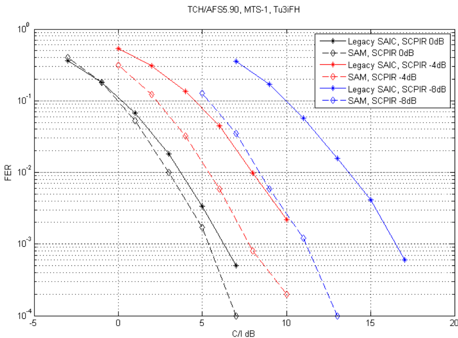
Figure 8-60a - MTS-1, AFS5.90
