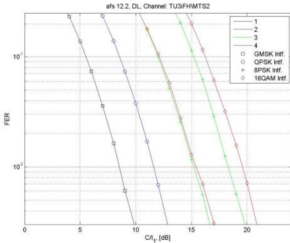
Figure 9-28: AMR 12.2 multiplexed users in DL, MTS-2/TU3iFH
