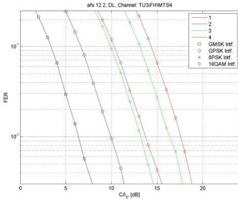
Figure 9-32: AMR 12.2 multiplexed users in DL, MTS-4/TU3iFH
