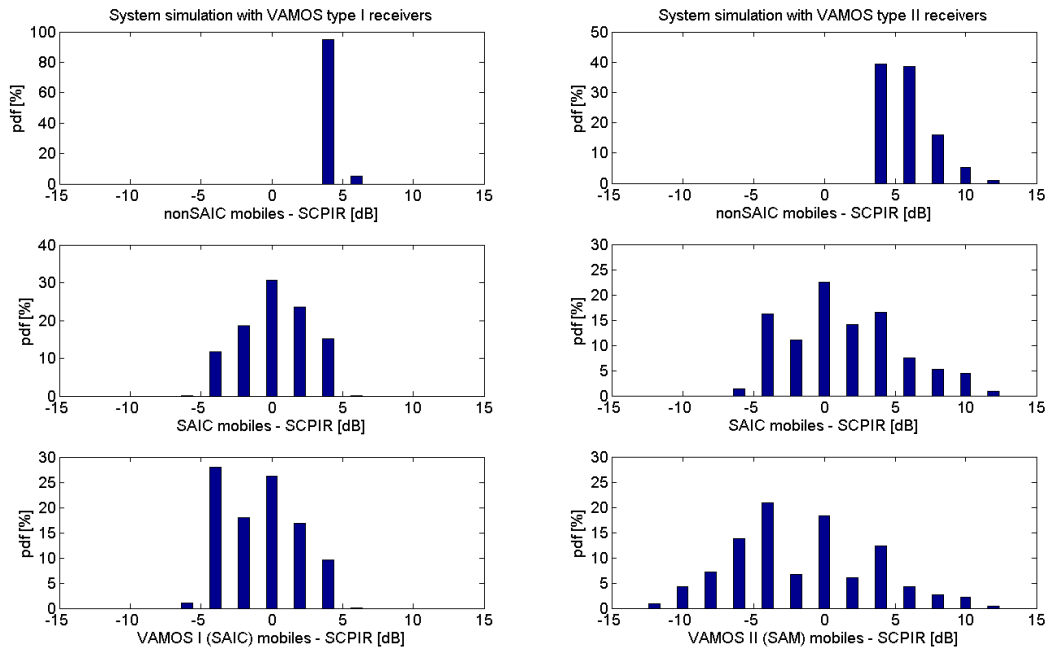
Figure 8-69: SCPIR distributions when using VAMOS I (left) and VAMOS II (right) receivers
