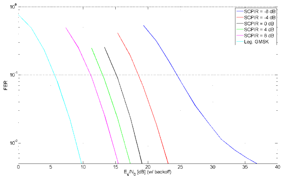
Figure 8-12: AHS/5.90 sensitivity
