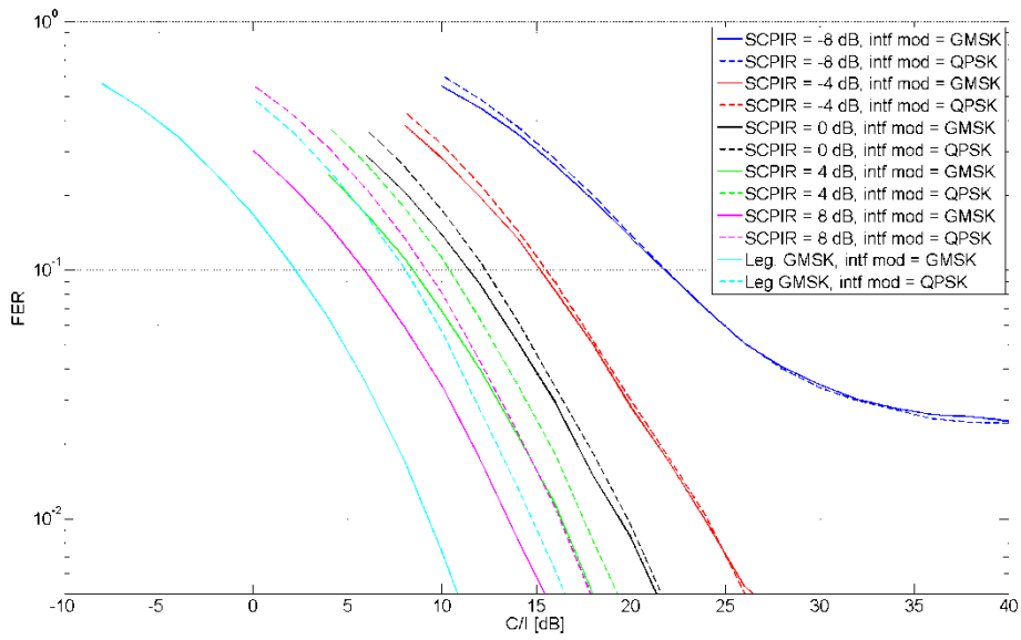
Figure 8-39: MTS-3, TU3nFH
