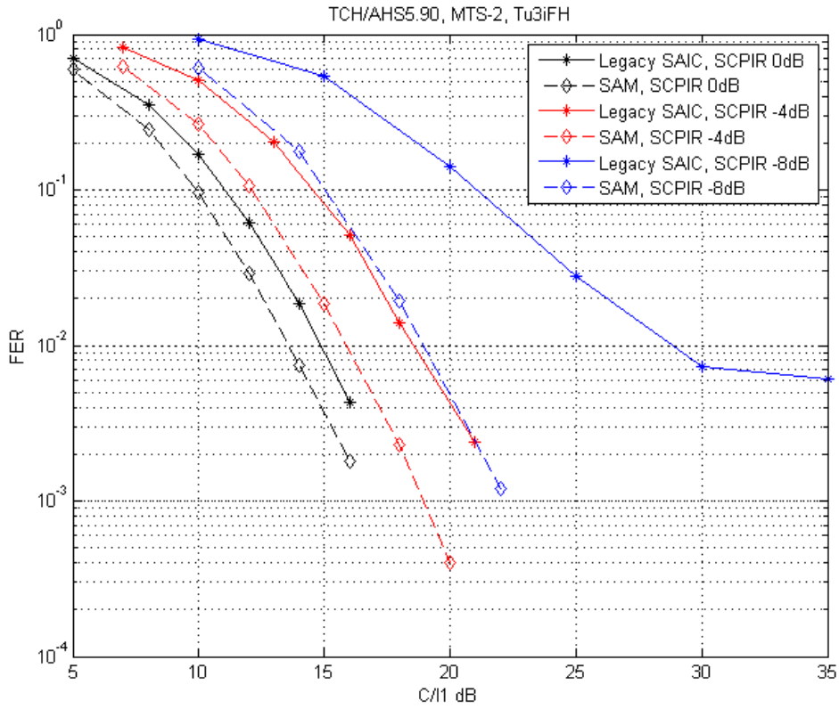
Figure 8-60d - MTS-2, AHS5.90
