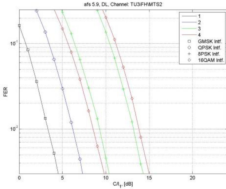
Figure 9-27: AMR 5.9 multiplexed users in DL, MTS-2/TU3iFH
