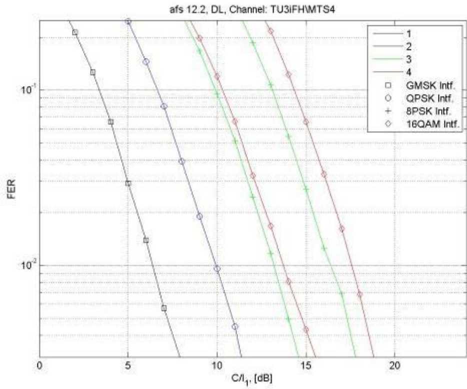
Figure 9-32: AMR 12.2 multiplexed users in DL, MTS-4/TU3iFHM4
