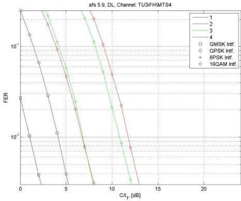
Figure 9-31: AMR 5.9 multiplexed users in DL, MTS-4/TU3iFHM4
