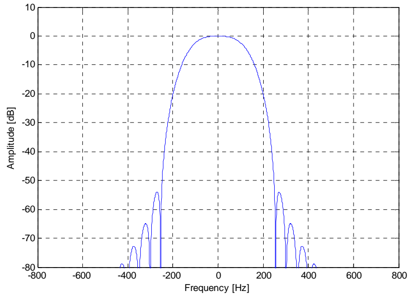
Figure 7-2a - Spectral power density of candidate pulse shape OPT 1.
