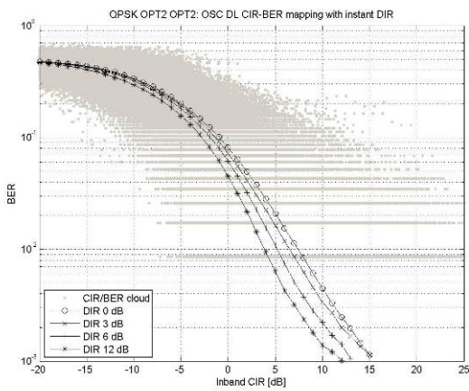
Figure 39-p. Mapping and verification for a QPSK modulated carrier
