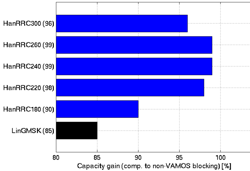
Figure 8-69a. Capacity gain MUROS-2, Scenario I.
