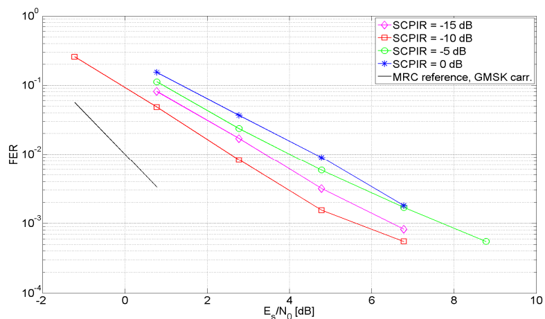
Figure 8-15 Sensitivity performance for TU3iFH, TCH/AFS5.90 (top left), TCH/AHS5.90 (top right) and TCH/AFS12.2 (bottom left).
