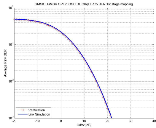
Figure 39-o. Mapping and verification for a GMSK modulated carrier
