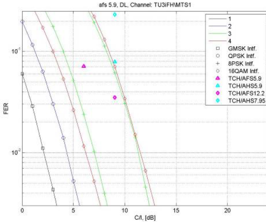
Figure 9-25: AMR 5.9 multiplexed users in DL, MTS-1/TU3iFH
