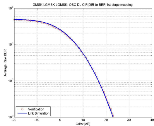
Figure 39-q. Mapping and verification for a GMSK modulated carrier
