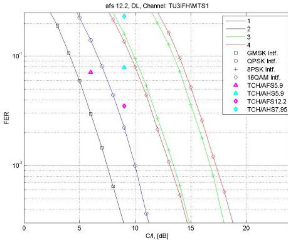
Figure 9-26: AMR 12.2 multiplexed users in DL, MTS-1/TU3iFH
