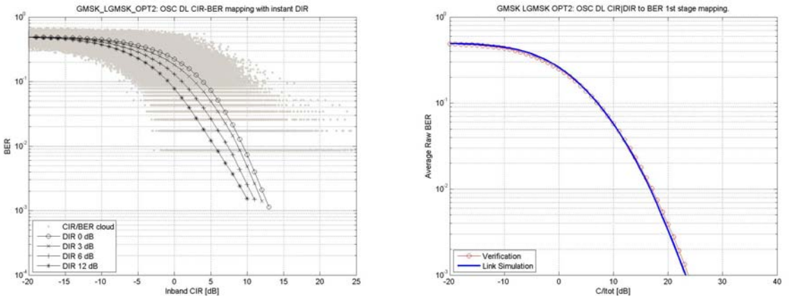
Figure 39-s. Mapping and verification for a GMSK modulated carrier
