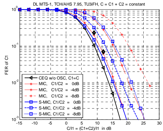
Figure 57b: MTS-1 for AHS 7.95, power C
