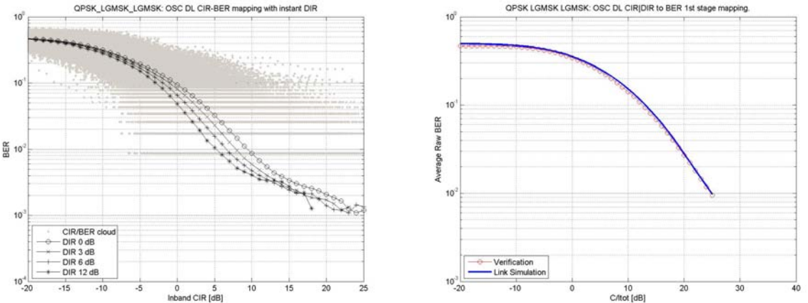
Figure 39-r. Mapping and verification for a QPSK modulated carrier
