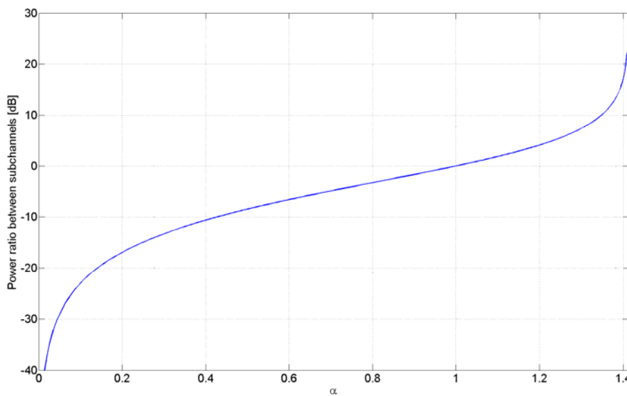
Figure 8-2: Cross power ratio
