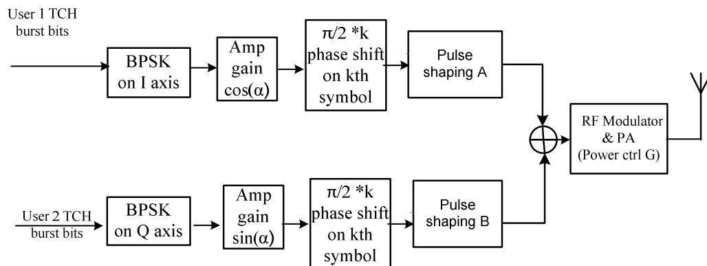
Figure 6-7a - Adaptive QPSK modulation with pulse shaping adaptation (A and B)
