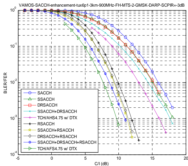
Fig. 11.3-10: Performance of MUROS AMR speech channels (with DTX), SACCH and SACCH enhancements (MTS-2, GMSK modulated interference, SCPIR=-3dB).
