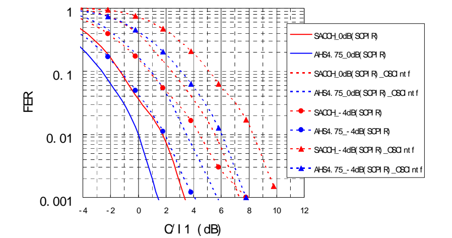
Figure 11-22: SACCH and TCH performance with shifted SACCH, DTX off
