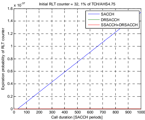
(a) 1% FER of TCH/AHS4.75
