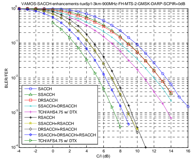
Fig. 11.3-8: Performance of MUROS AMR speech channels (with DTX), SACCH and SACCH enhancements (MTS-2, GMSK modulated interference, SCPIR=0dB).
