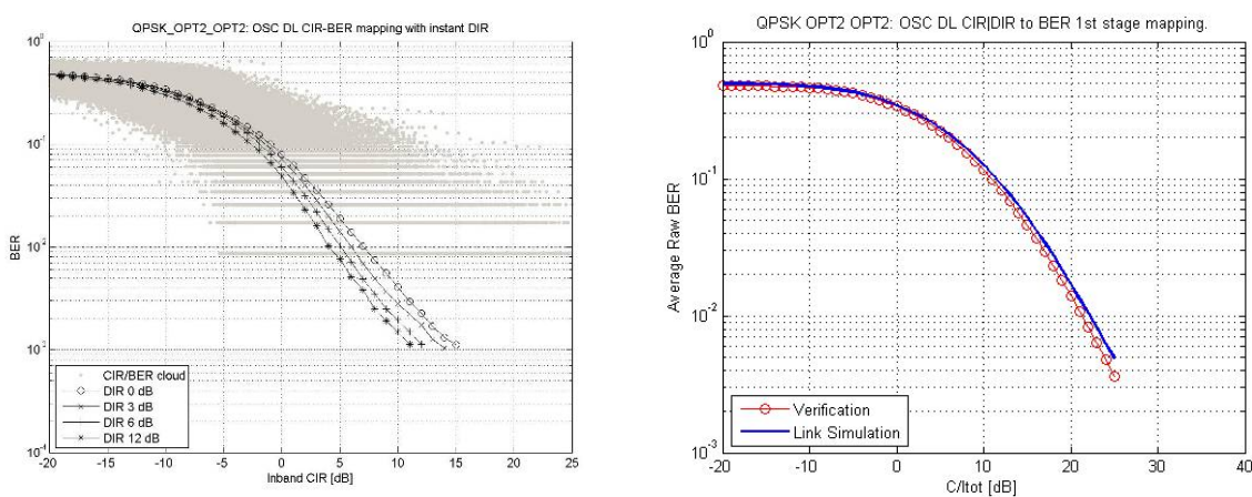
Figure 39-t. Mapping and verification for a QPSK modulated carrier
