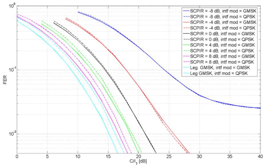
Figure 8-40: MTS-4, TU3nFH
