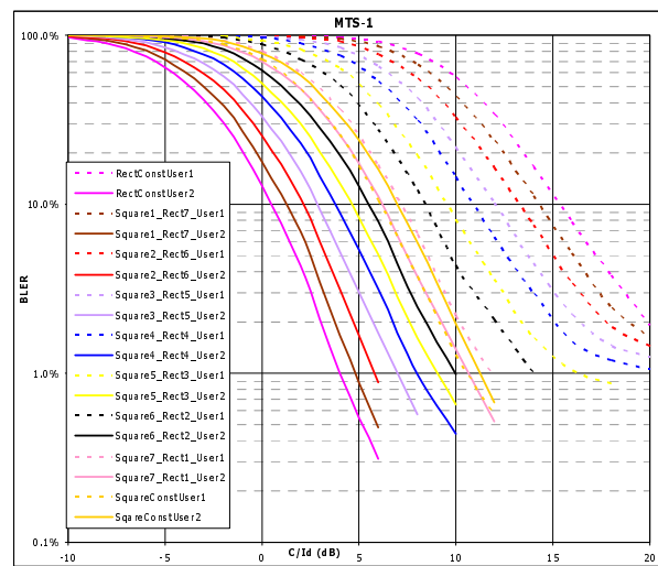
Figure 7-22: TCHAFS 12.2
