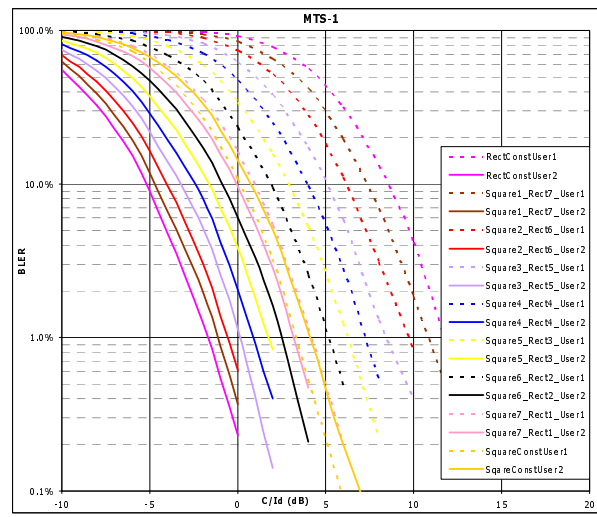
Figure 7-24: TCHAFS 5.9
