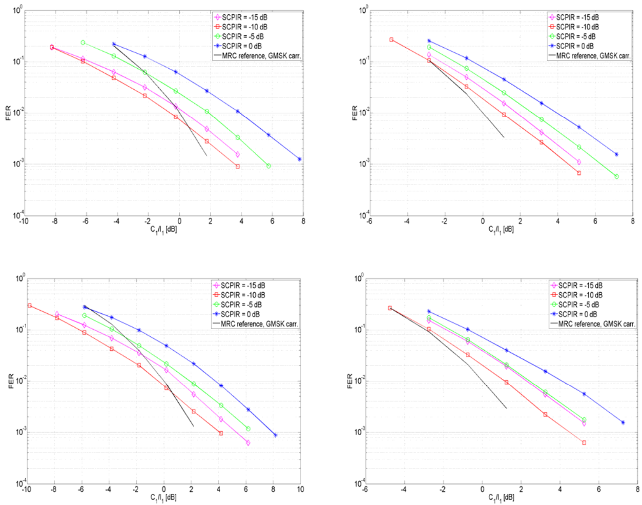
Figure 47 - TCH/AHS5.90, TU31FH. MTS-1 (top left), MTS-2 (top right), MTS-3 (bottom left), MTS-4 (bottom right)
