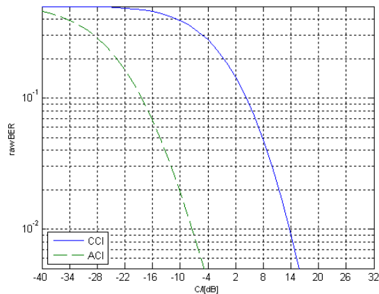
Figure 8-80. ACI to CCI mapping, Intf. Mod. = QPSK
