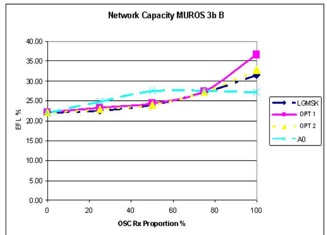
Figure 7-38D2: EFL for investigated TX pulse shapes (MUROS-3b, Channel type B) and different penetrations for OSC aware MS.
