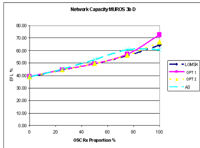
Figure 7-38D4: EFL for investigated TX pulse shapes (MUROS-3b, Channel type D) and different penetrations for OSC aware MS.
