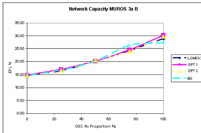
Figure 7-38C2: EFL for investigated TX pulse shapes (MUROS-3a, Channel type B) and different penetrations for OSC aware MS.
