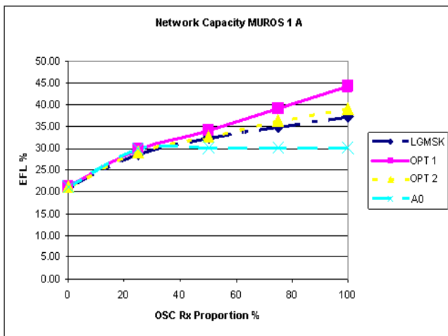
Figure 7-38A1: EFL for investigated TX pulse shapes (MUROS-1, Channel type A) and different penetrations for OSC aware MS.
