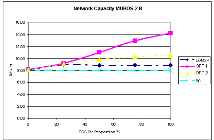
Figure 7-38B2: EFL for investigated TX pulse shapes (MUROS-2, Channel type B) and different penetrations for OSC aware MS.
