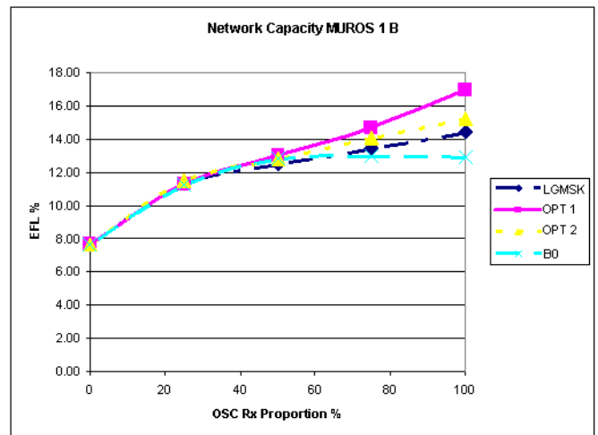
Figure 7-38A2: EFL for investigated TX pulse shapes (MUROS-1, Channel type B) and different penetrations for OSC aware MS.
