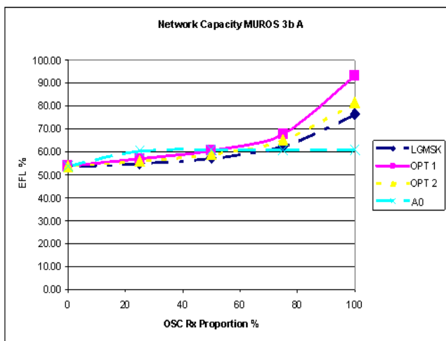
Figure 7-38D1: EFL for investigated TX pulse shapes (MUROS-3b, Channel type A) and different penetrations for OSC aware MS.
