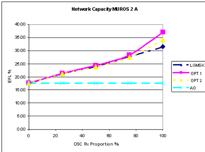
Figure 7-39B1: EFL for investigated TX pulse shapes (MUROS-2, Channel type A) and different penetrations for OSC aware MS
