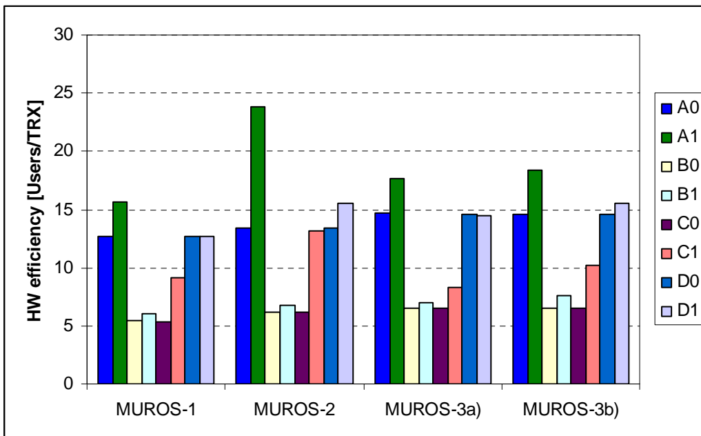
Figure 7-37: HW efficiency for OSC with LGMSK pulse shape in DL for agreed MUROS network configurations
