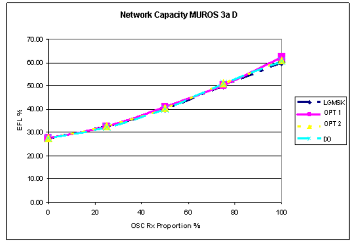
Figure 7-38C4: EFL for investigated TX pulse shapes (MUROS-3a, Channel type D) and different penetrations for OSC aware MS.
