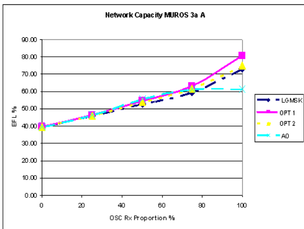
Figure 7-38C1: EFL for investigated TX pulse shapes (MUROS-3a, Channel type A) and different penetrations for OSC aware MS.
