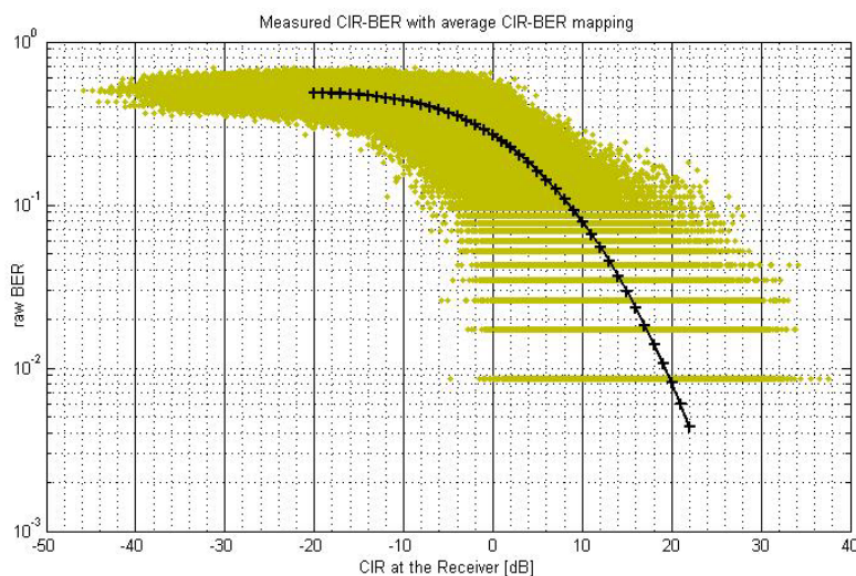
Figure 7-38E2 - Example relationship between the measured burst-wise CIR after the Rx front-end filter and the raw BER distribution for SAIC OSC, with average CIR-BER mapping.
