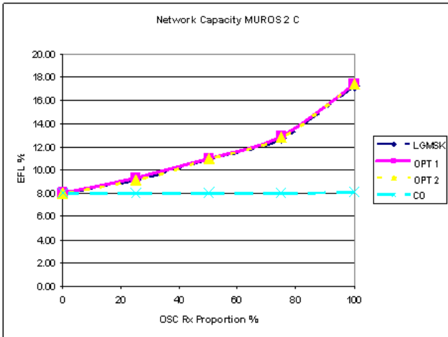
Figure 7-38B3: EFL for investigated TX pulse shapes (MUROS-2, Channel type C) and different penetrations for OSC aware MS.
