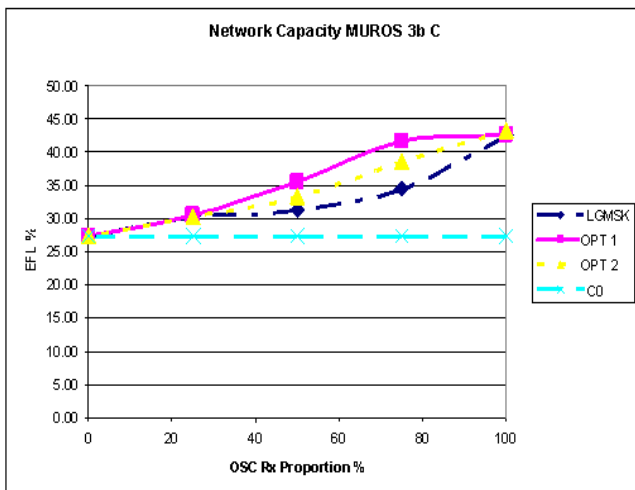
Figure 7-38D3: EFL for investigated TX pulse shapes (MUROS-3b, Channel type C) and different penetrations for OSC aware MS.
