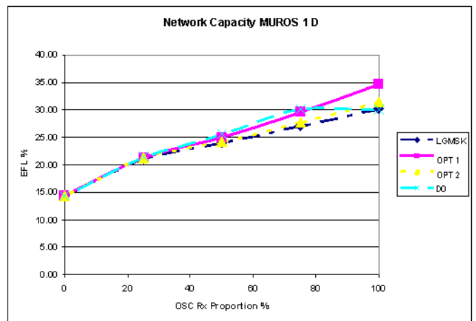
Figure 7-38A4: EFL for investigated TX pulse shapes (MUROS-1, Channel type D) and different penetrations for OSC aware MS.
