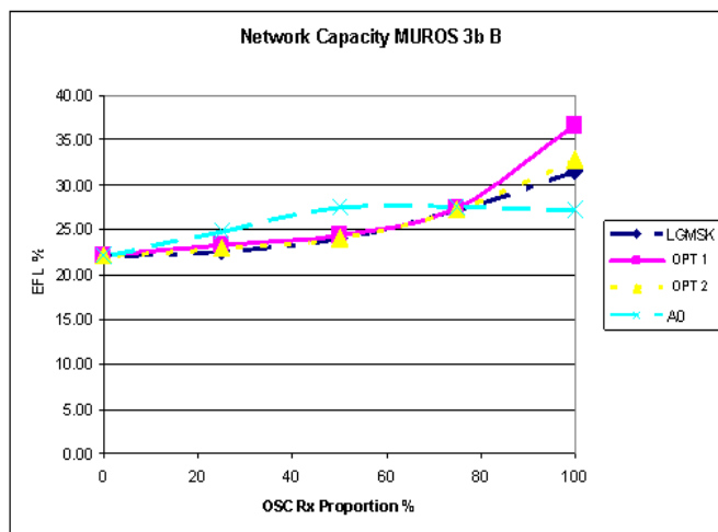
Figure 7-38D2: EFL for investigated TX pulse shapes (MUROS-3b, Channel type B) and different penetrations for OSC aware MS.
