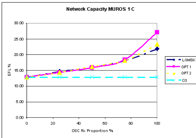
Figure 7-38A3: EFL for investigated TX pulse shapes (MUROS-1, Channel type C) and different penetrations for OSC aware MS.
