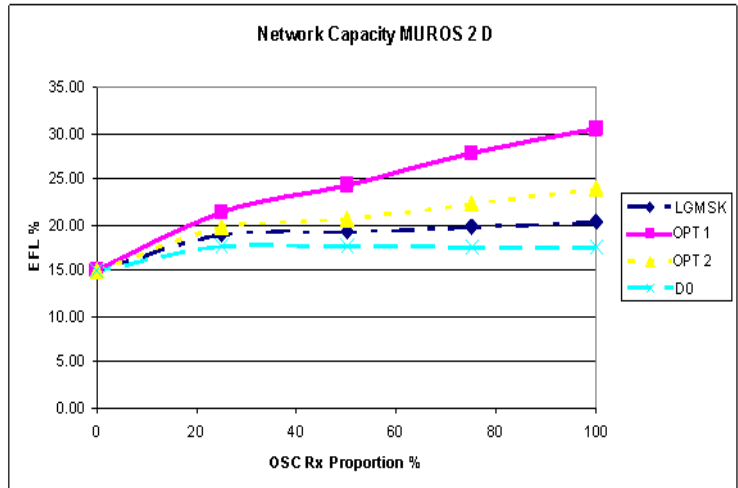
Figure 7-38B4: EFL for investigated TX pulse shapes (MUROS-2, Channel type D) and different penetrations for OSC aware MS.
