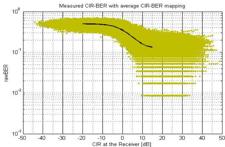
Figure 7-38E1- Example relationship between the measured burst-wise CIR after the Rx front-end filter and the raw BER distribution for non-SAIC OSC, with average CIR-BER mapping.
