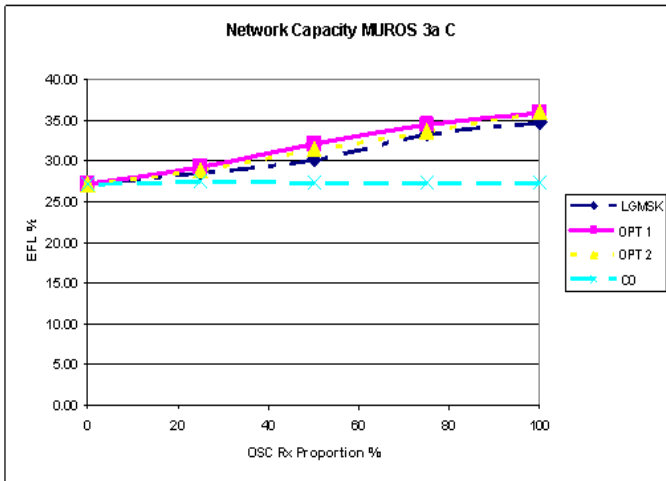
Figure 7-38C3: EFL for investigated TX pulse shapes (MUROS-3a, Channel type C) and different penetrations for OSC aware MS.
