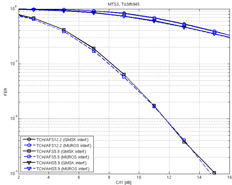
Figure 7-32: DL Asynchronous Co-channel interference performance (MTS3) of a non-legacy DARP MS receiving a MUROS sub channel using AMR half rate 5.9, AMR full rate 12.2 and AMR full rate 5.9
