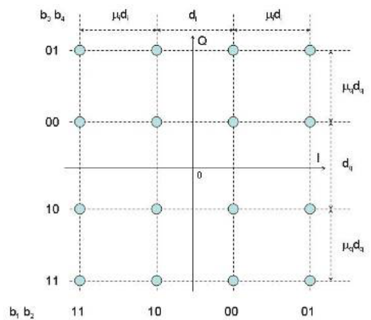
Figure 9-6: Downlink power control on HOM- 16QAM
