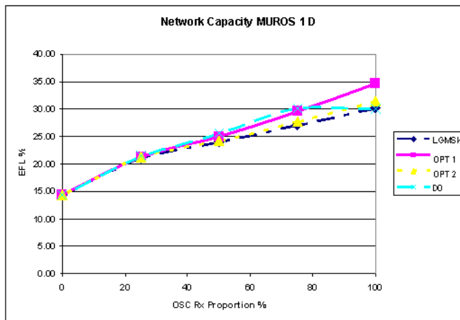
Figure 7-38A4: EFL for investigated TX pulse shapes (MUROS-1, Channel type D) and different penetrations for OSC aware MS.
