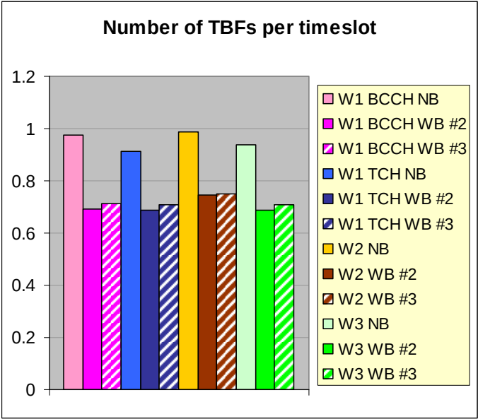
Figure 9.1: Average number of active TBFs per timeslot (at equal the PS load)
