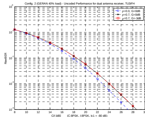
Figure 25: Uncoded BER of MS RX diversity for GMSK (left figure) and 8PSK (right figure), configuration 2 and different antenna gain imbalances and correlations [21]
