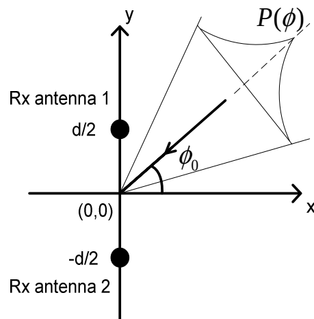
Figure 21: Antenna setup at MS side for evaluation of the impact on phase difference between antenna correlations [22]
