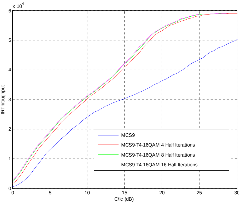
Figure 188: Throughput Performance for MCS9 and MCS9-T4-16QAM in TU3iFH Channel with Variable Number of Turbo Decoding Iterations
