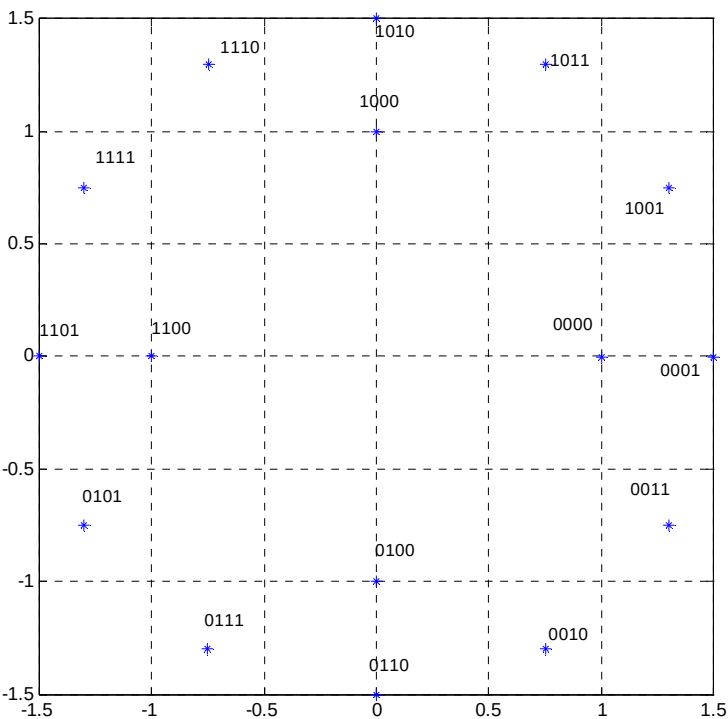
Figure 224: 16APK (12,4) Constellation
