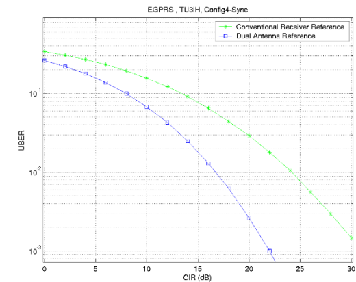
Figure 30: Uncoded BER performance comparison of the DAIC and conventional 8PSK receivers for Synchronized Network (a) Config3, and (b) Config4 [18]
