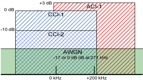
Figure 272: DTS-2 Link scenario with higher symbol rate interference
