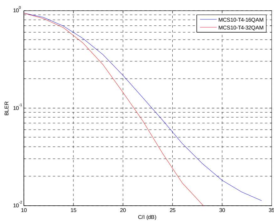
Figure 206: TU3iFH Co-Channel Performance (MCS-10)
