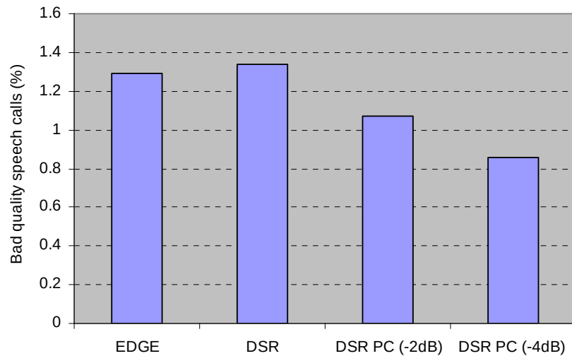
Figure 260: Percentage of bad quality voice calls for EGPRS and DSR with power offsets
