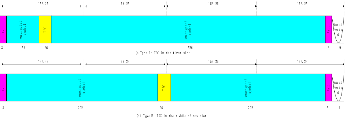
Figure 371: Aggregation of four slots
