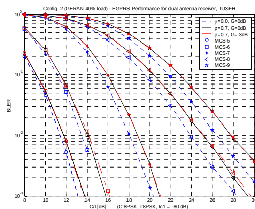
Figure 26: BLER of MS RX diversity for MCS-1 to MCS-4 (left figure) and MCS-5 to MCS-9 (right figure), configuration 2 and different antenna gain imbalances and correlations [21]
