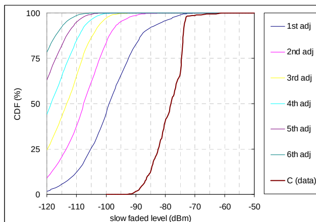
Figure 244: 1/3 adjacent channel I levels
