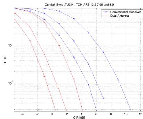
Figure 32: TCH/AFS FER Performance comparison of the DAIC and conventional receivers for Synchronized Network (a) Config3 and (b) Config4 [18]
