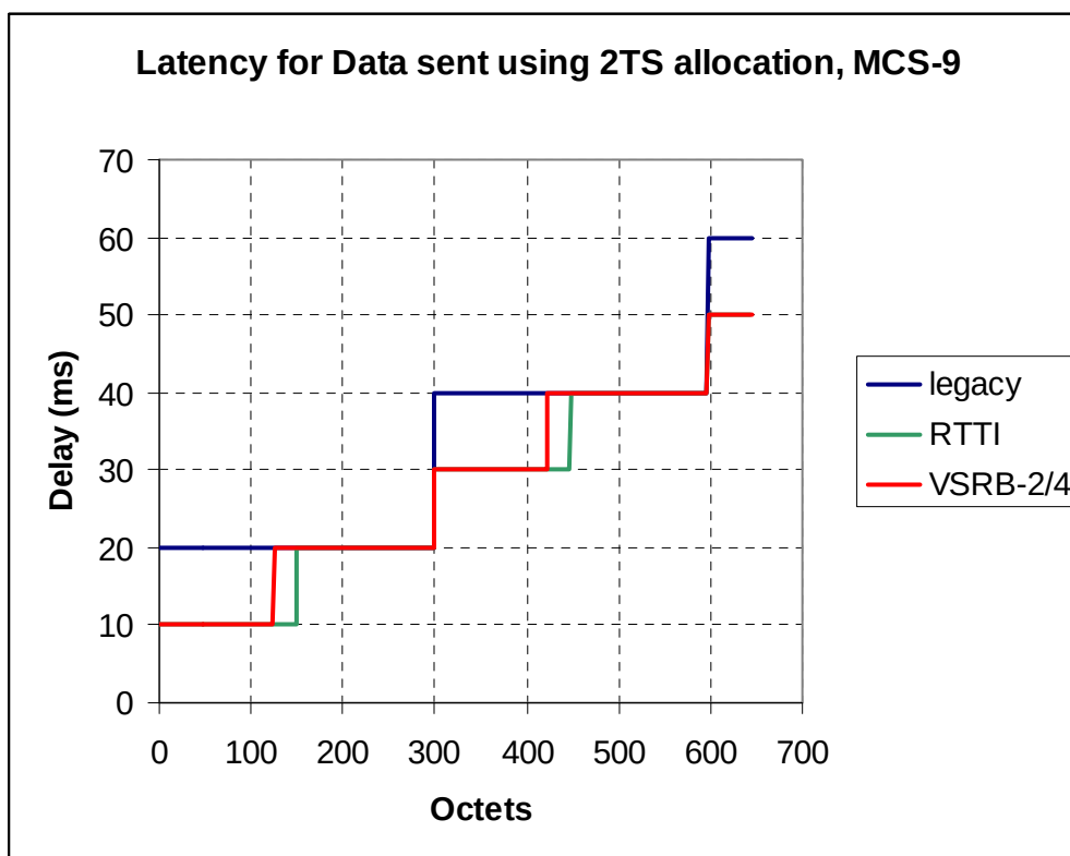
Figure 344: Delay over the radio interface / data sent (4-burst or 2-burst blocks)
