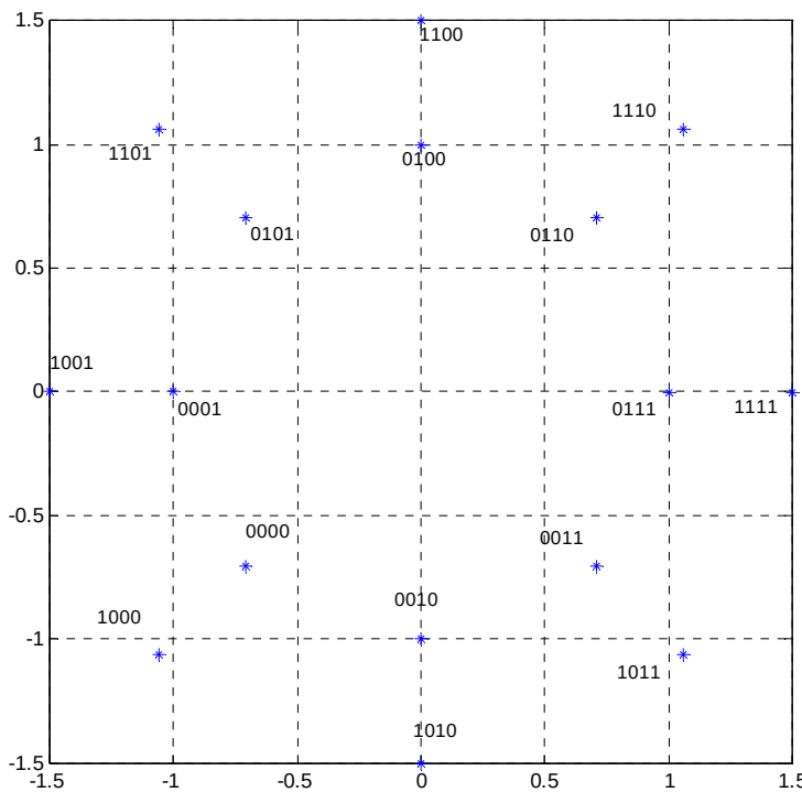
Figure 225: 16APK (8,8) Constellation
