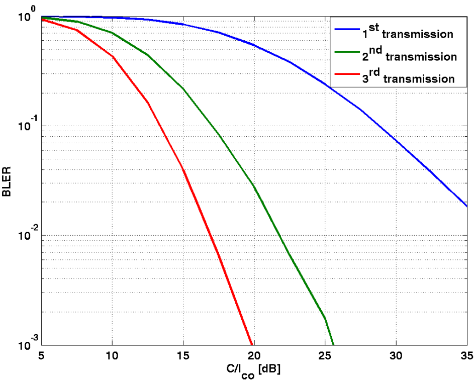
Figure B.8: Link performance with IR for MCS-11-16QAM on TU3iFH
