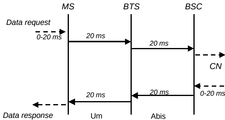
Figure 289: Indicative delays in GERAN network for a time slot Note that it is assumed that the Abis delay is the same as the TTI value
