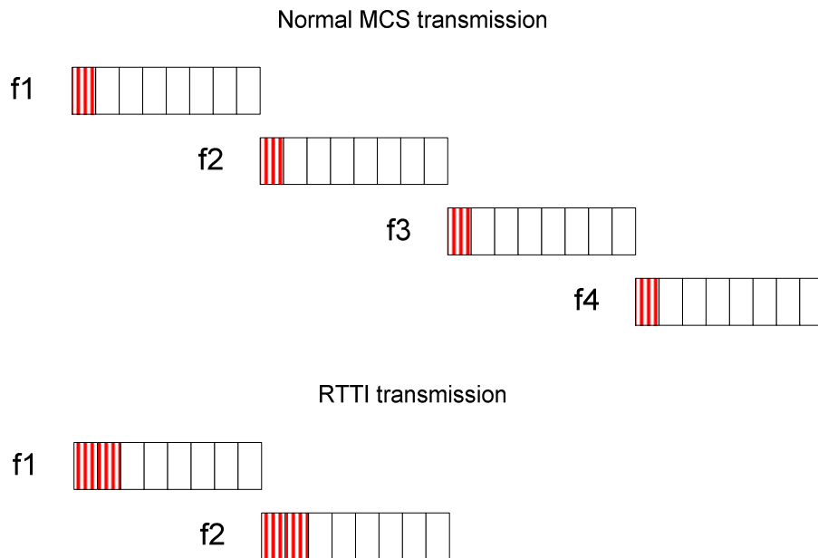
Figure 325: Reduced TTI burst mapping
