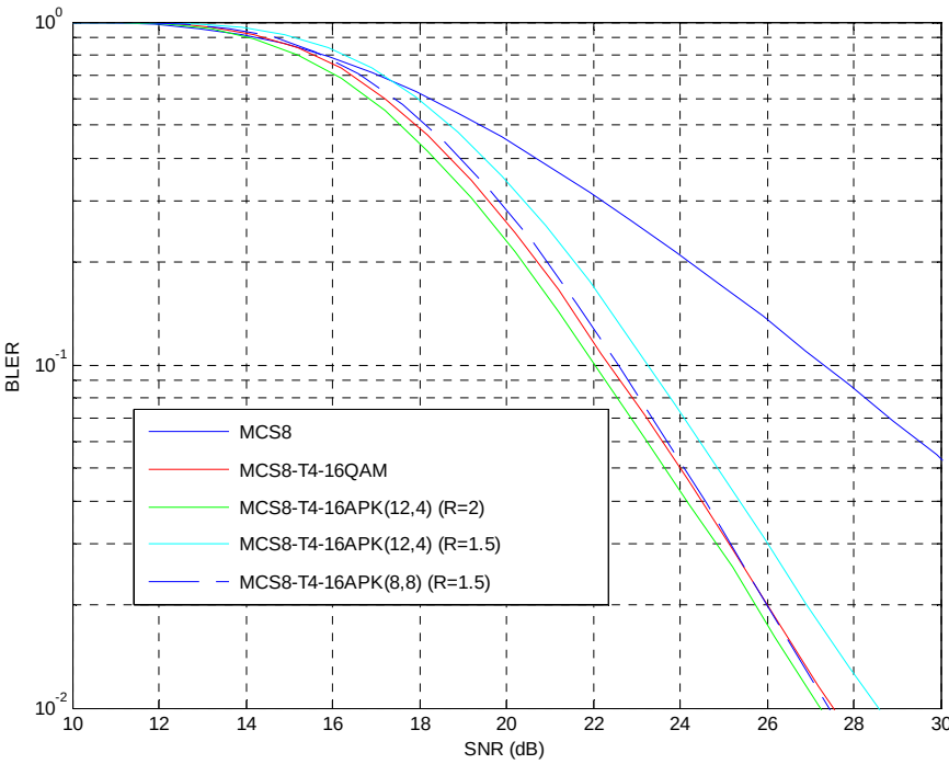
Figure 228: TU3iFH Sensitivity Performance (MCS-8)
