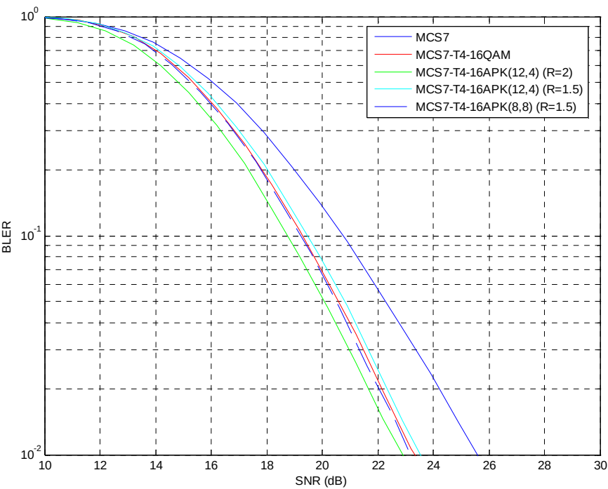
Figure 227: TU3iFH Sensitivity Performance (MCS-7)
