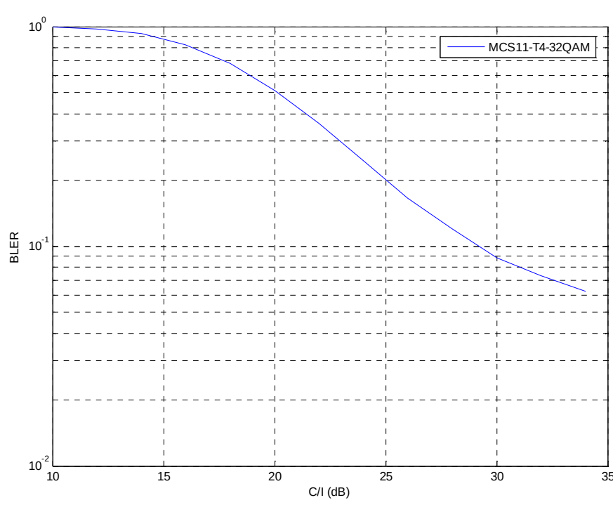
Figure 207: TU3iFH Co-Channel Performance (MCS-11)
