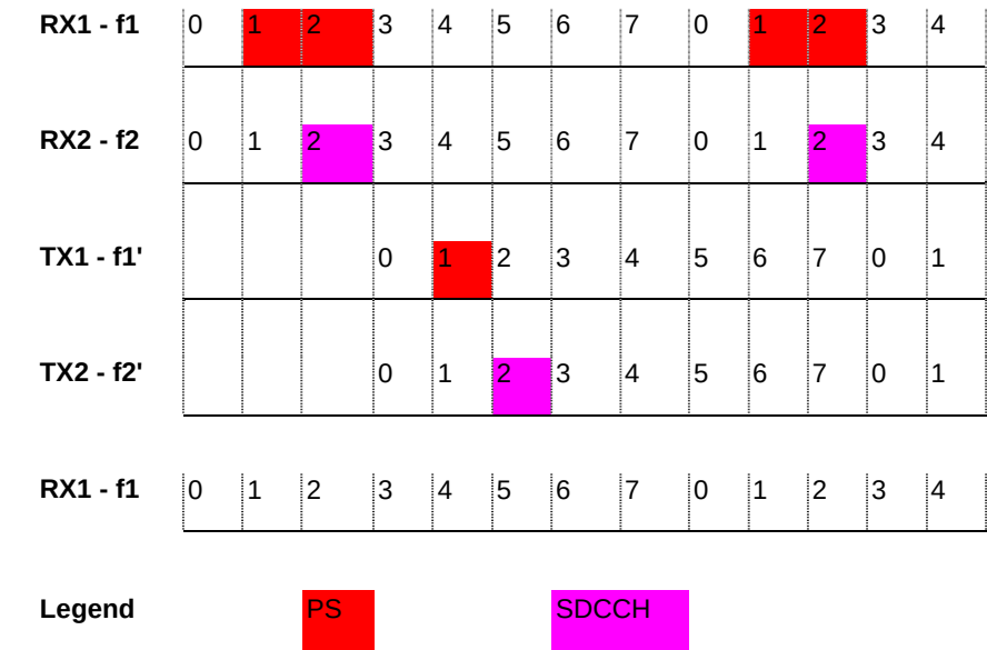
Figure 87: Allocation of SDCCH on Second Carrier Pair
