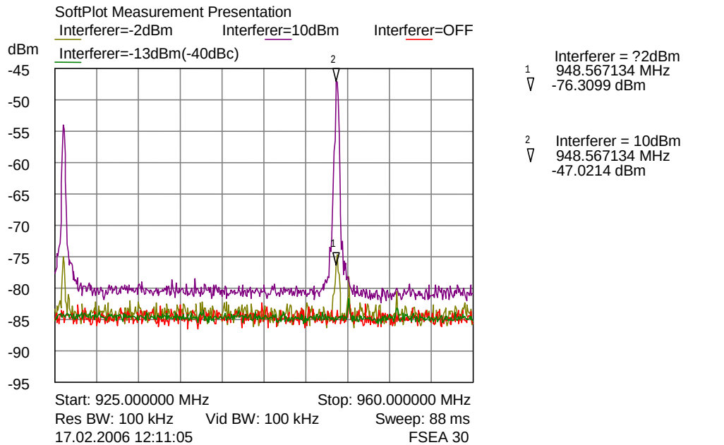
Figure 72: IM5 Measurements for 8-PSK 27 dBm mode - Setup 2
