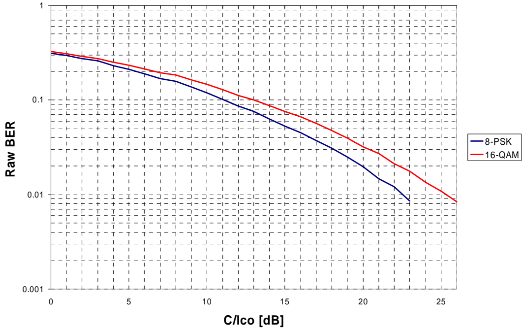
Figure 117: Raw BER (TU3nFH@900MHz, no impairments)
