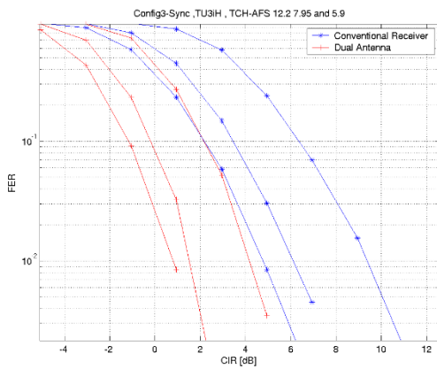
(a) (b) Figure 32: TCH/AFS FER Performance comparison of the DAIC and conventional receivers for Synchronized Network (a) Config3 and (b) Config4 [18]
