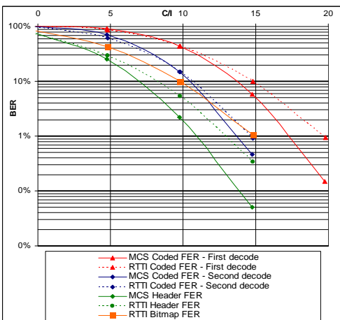
Figure 331: MCS 6 like coding scheme - TU 50 ideal FH
