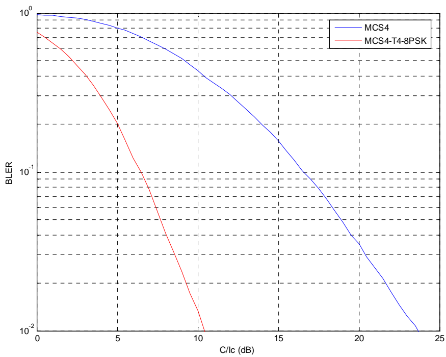
Figure 193: BLER Performance for MCS4 and MCS4-T4-8PSK in TU3iFH Channel
