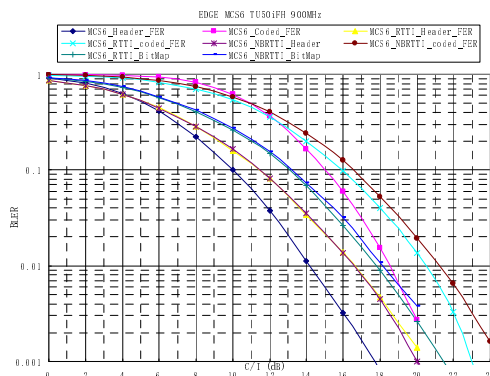
Figure 387: MCS 6 like coding scheme - TU 50 ideal FH
