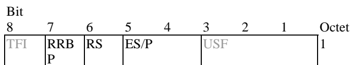
Figure 304: RRBP, RS and ES/P fields in modified EGPRS downlink RLC data block headers
