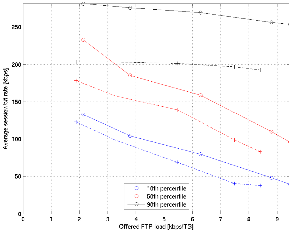
Figure 153b. Average session bit rate percentiles, 10th percentile (blue), 50th percentile (red), 90th percentile (black), as a function of offered FTP load, for EGPRS (dashed) and HQT level 2 (solid), in a 3-reuse.
