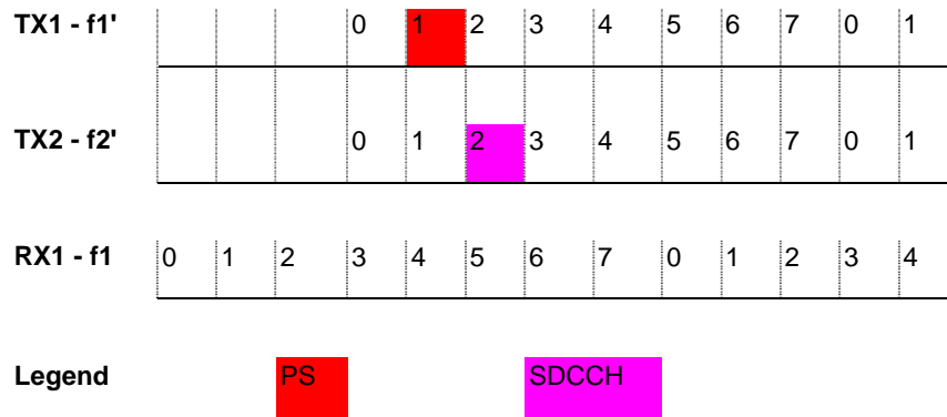
Figure 87: Allocation of SDCCH on Second Carrier Pair
