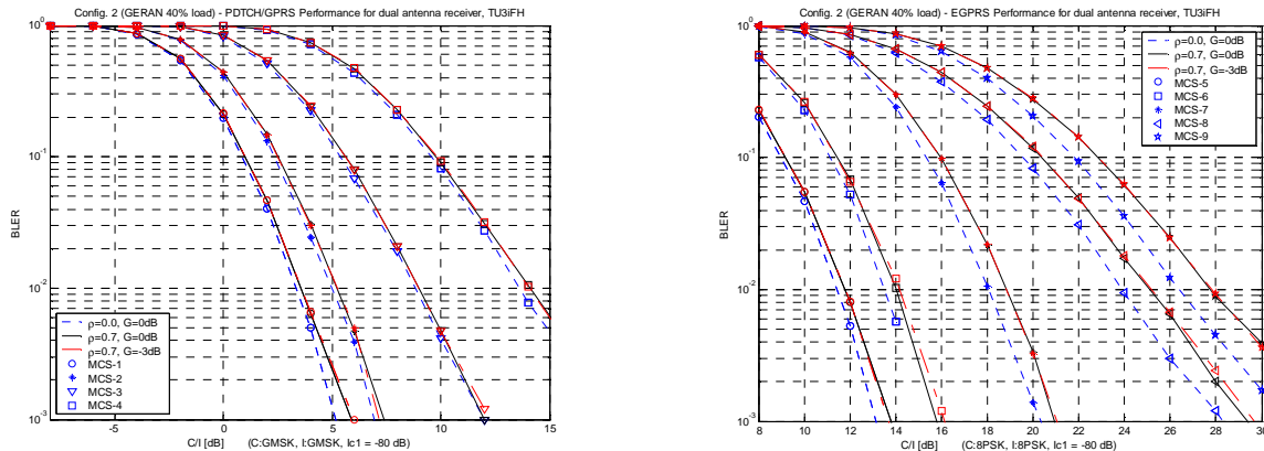
Figure 26: BLER of MS RX diversity for MCS-1 to MCS-4 (left figure) and MCS-5 to MCS-9 (right figure), configuration 2 and different antenna gain imbalances and correlations [21]
