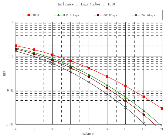
Figure 282: Influence of DSR receiver taps number in TU50 using single antenna
