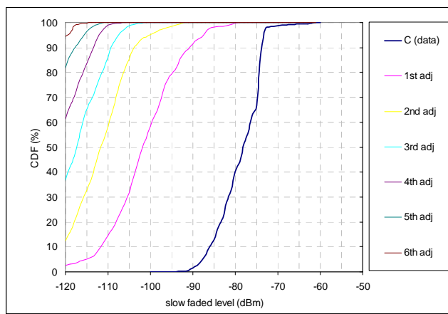
Figure 242: 4/12 adjacent channel I level cdf
