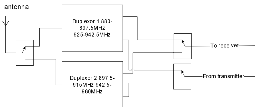
Figure 419a: Block diagram of new duplexer architecture
