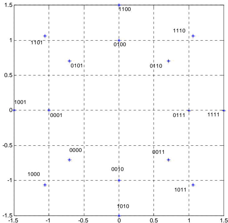
Figure 225: 16APK (8,8) Constellation
