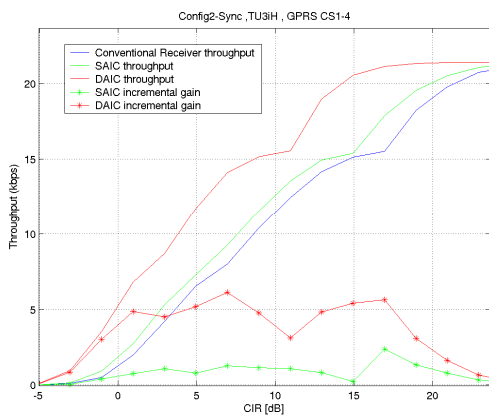
(a) (b) Figure 39: GPRS Hull-curve comparison of the DAIC, SAIC and conventional receivers for Synchronized Network (a) Config2 and (b) Config3 [18]
