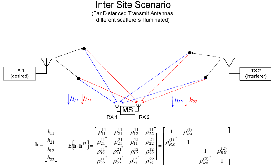
Figure 4: Inter-site interference scenario [13]
