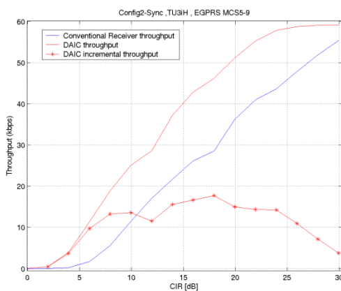
(a) (b) Figure 40: EGPRS Hull-curve comparison of the DAIC and conventional receivers for Synchronized Network (a) Config2 and (b) Config3 [18]
