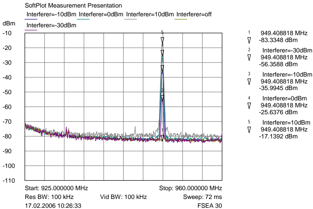
Figure 69: Measurements for IM3 in GSK mode - f1 at 32 dBm - Setup 1
