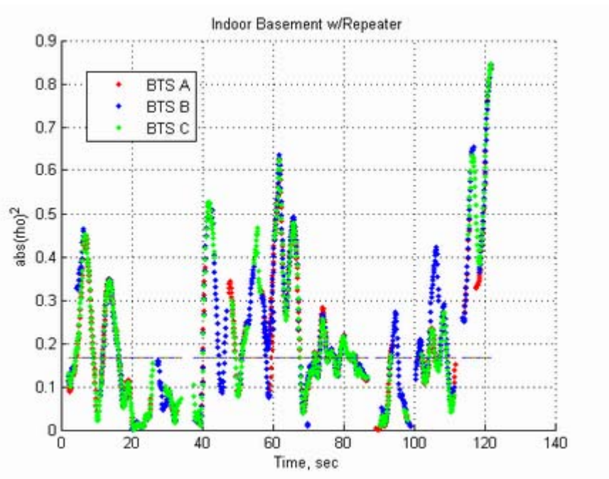
Figure 12: Indoor, Pedestrian Speed. With repeater - Full view [15]
