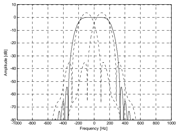
Figure 238: MDSR spectrum
