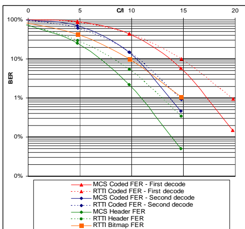
Figure 331: MCS 6 like coding scheme - TU 50 ideal FH
