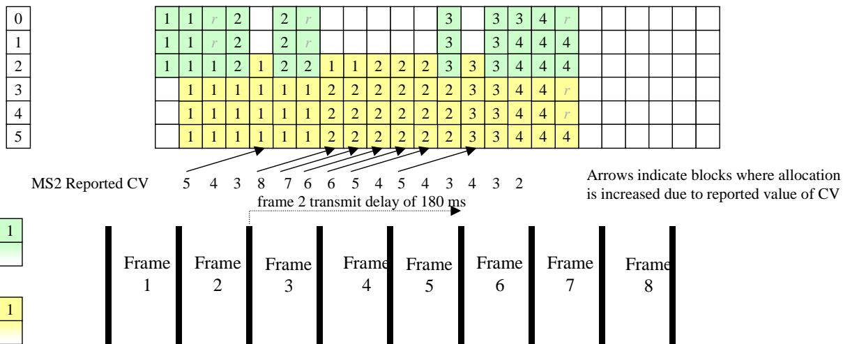
Figure 397: Scenario 3:EDA, sudden data rate peak for MS2
