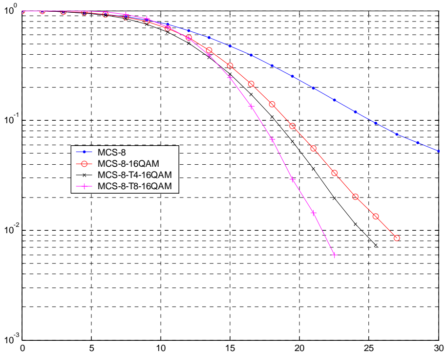
Figure C.4: TU50nH Co-Channel Performance (MCS-8)
