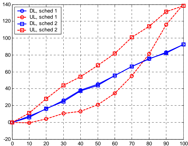
Figure 232i: CIR 35 dB, load factor: 80.0%, DL: 754.7 kbps/cell, UL: 754.7 kbps/cell.
