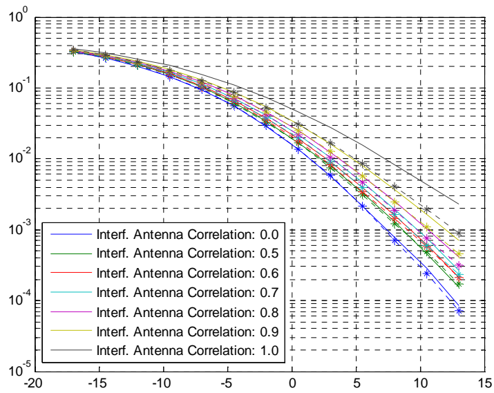
Figure 19: BER performance. TU50nFH1845. DTS-1 - With and without phase offset [26]
