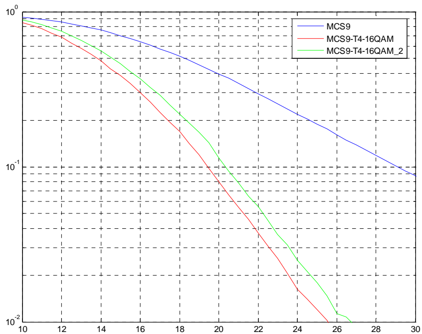
Figure 213: TU3iFH Co-Channel Performance (MCS-9)
