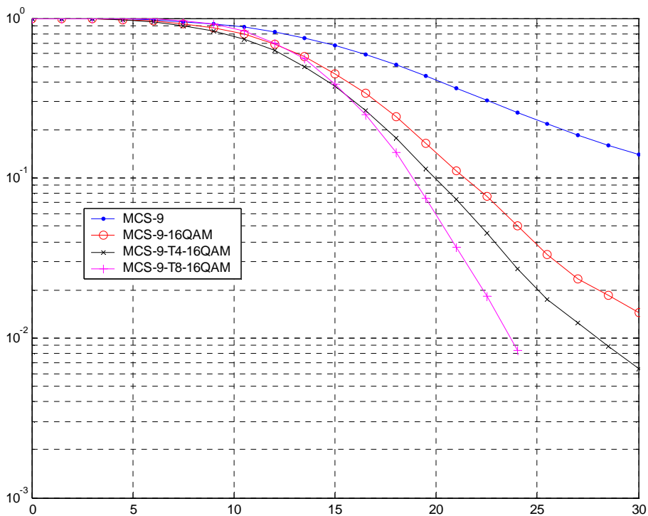
Figure C.5: TU50nH Co-Channel Performance (MCS-9)
