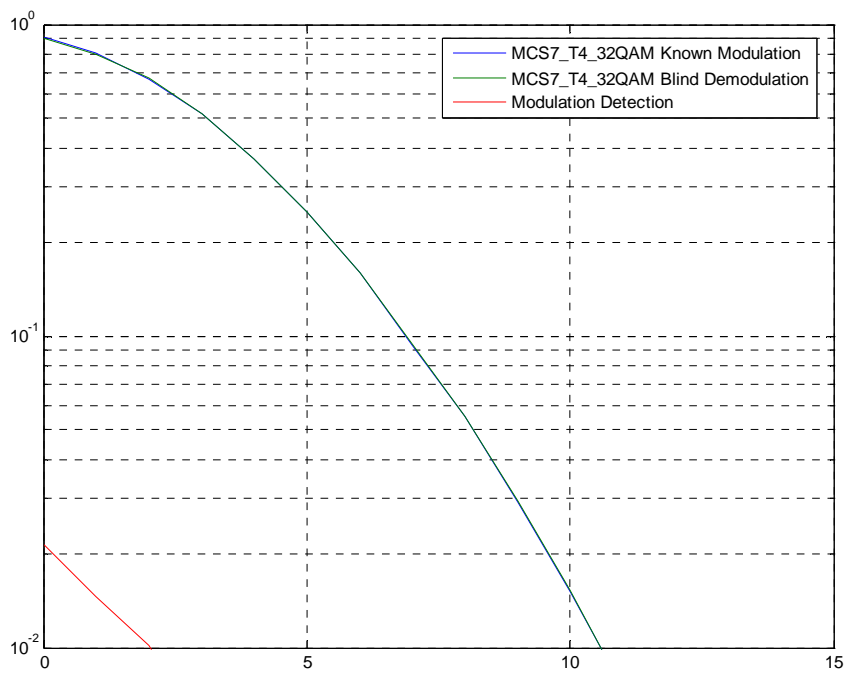
Figure C.19: MCS7-T4-32QAM, Sensitivity, TU50iFH
