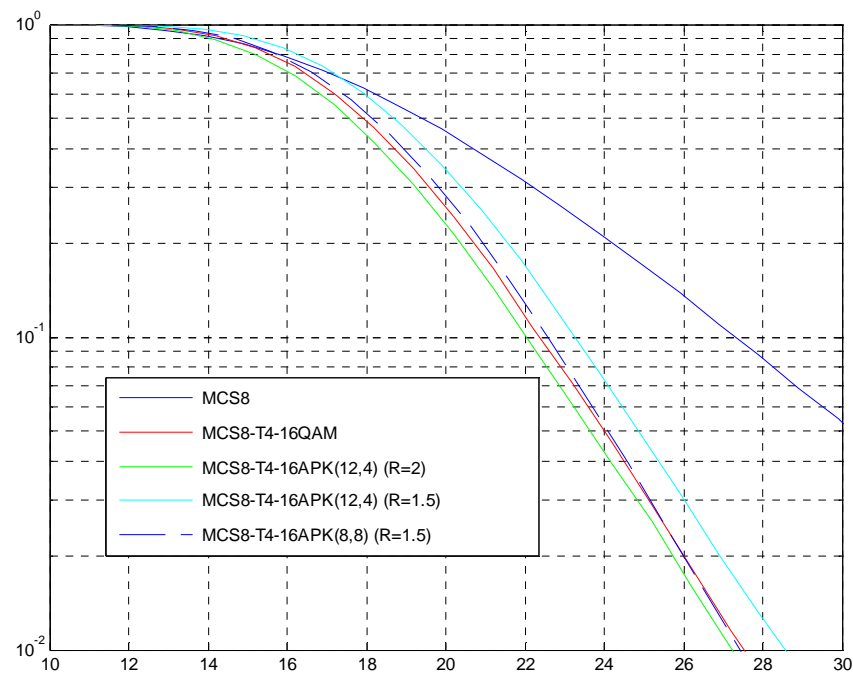
Figure 228: TU3iFH Sensitivity Performance (MCS-8)
