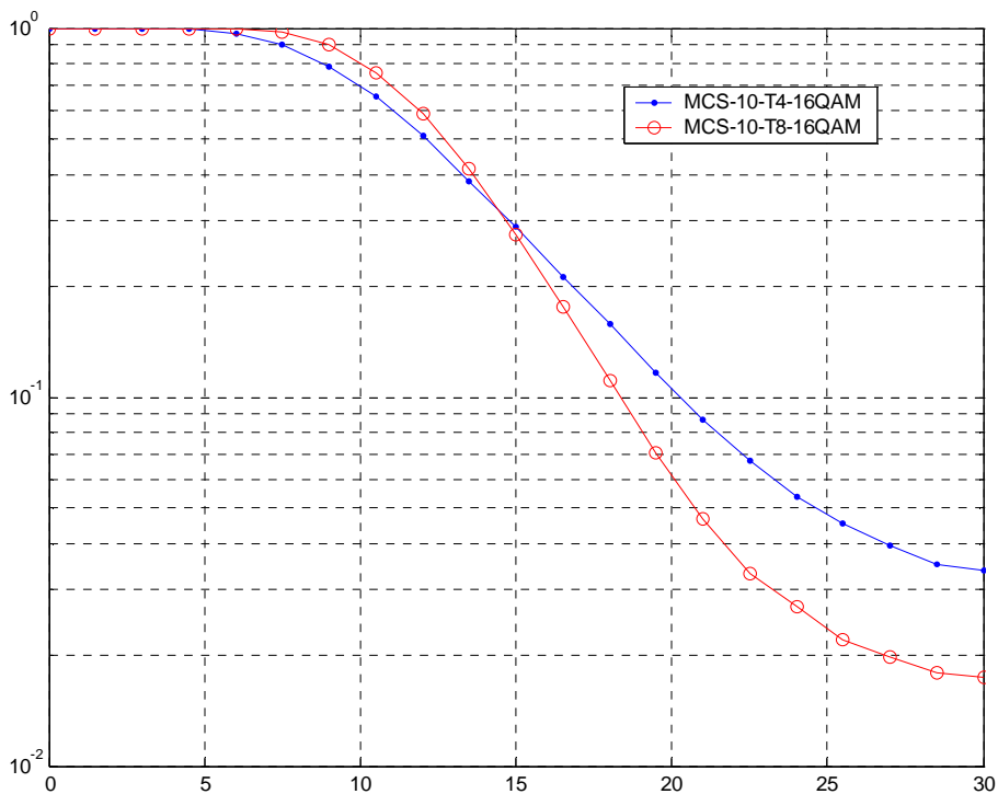
Figure 168: TU3iFH Sensitivity Performance (MCS-10 16-QAM)
