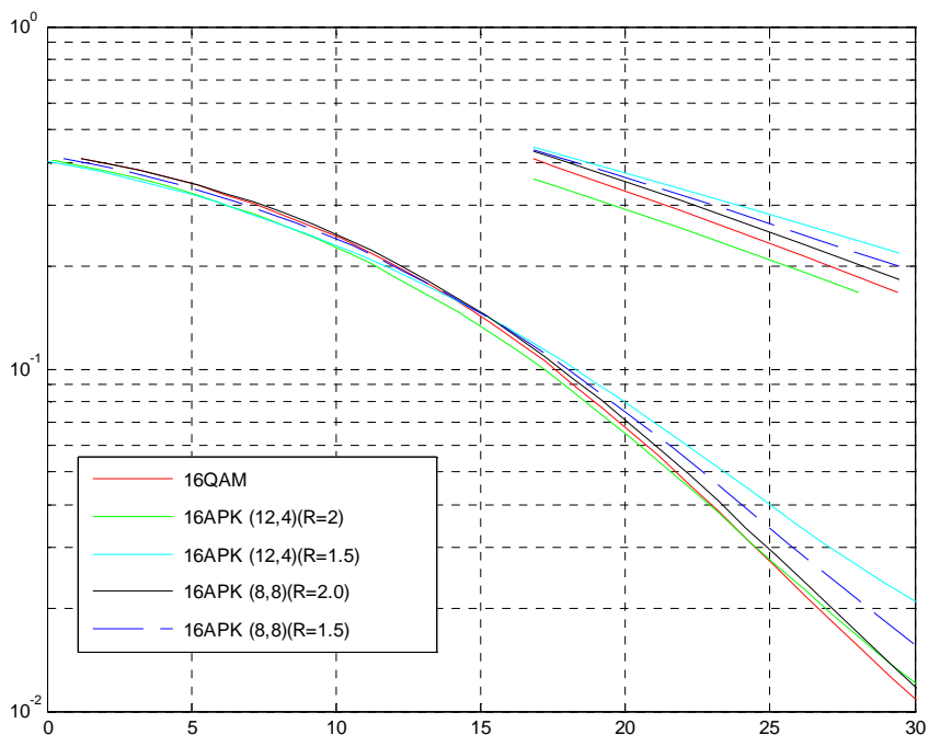
Figure 226: Uncoded BER of 16QAM, 16APK (12,4) & (8,8) Modulations
