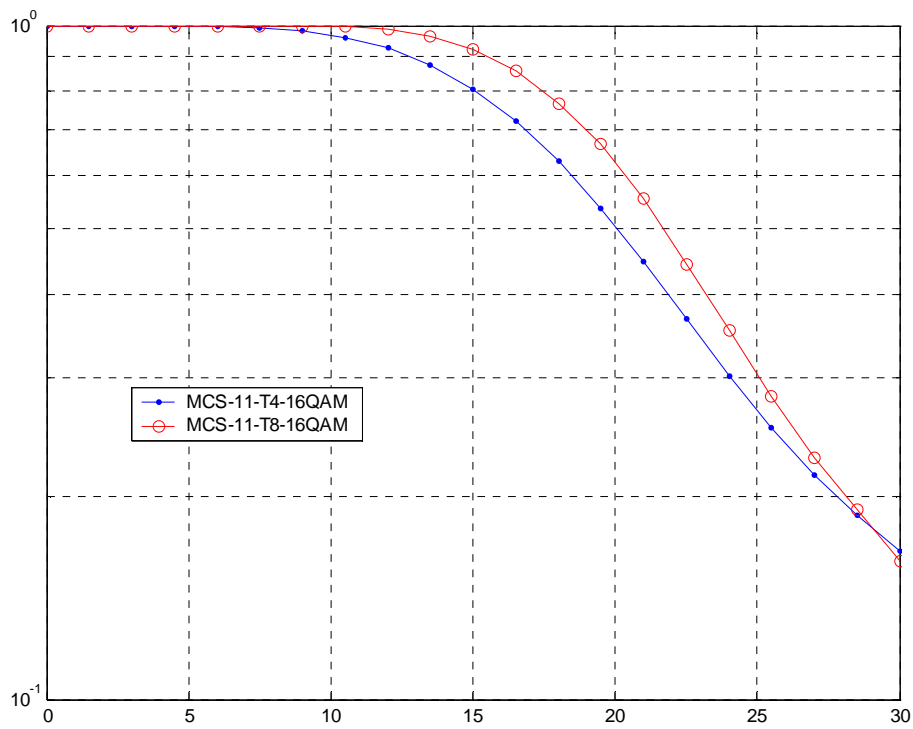
Figure C.7: TU50nH Co-Channel Performance (MCS-11 16-QAM)
