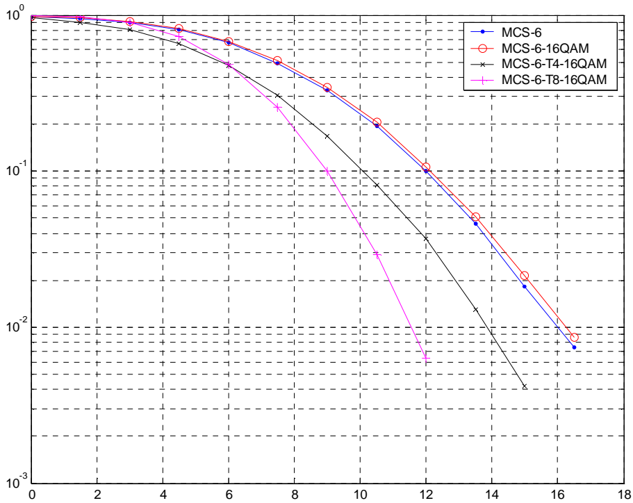
Figure 157: TU3iFH Co-Channel Performance (MCS-6)
