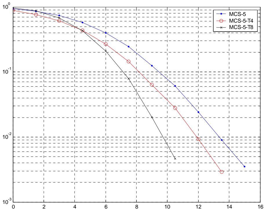
Figure 156: TU3iFH Co-Channel Performance (MCS-5)
