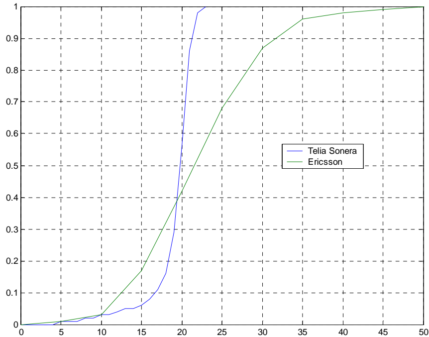
Figure 195: CDFs of C/Ico Distribution
