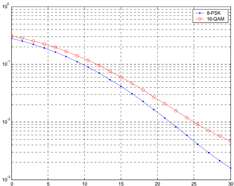
Figure 155: Uncoded BER for 8-PSK under TU3 Channel
