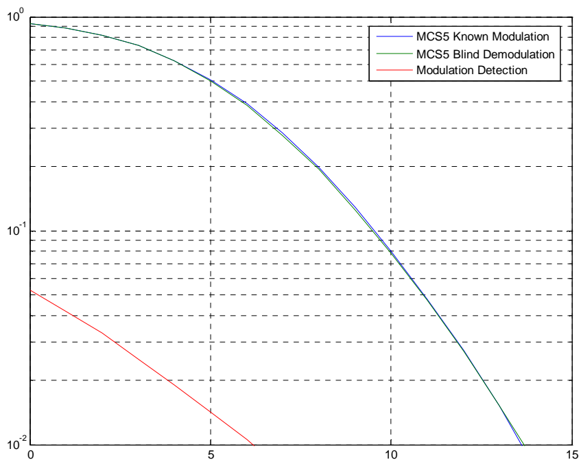
Figure C.13: MCS5, Co-channel, TU50iFH
