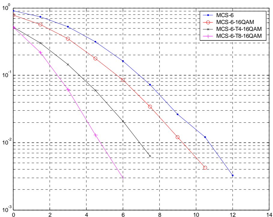
Figure 164: TU3iFH Sensitivity Performance (MCS-6)
