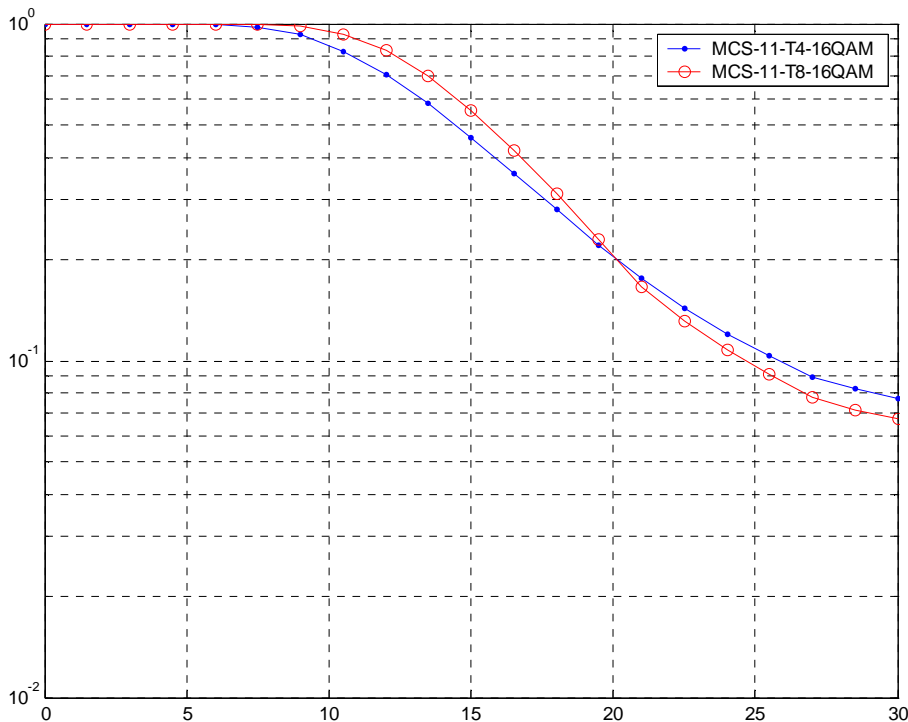
Figure 169: TU3iFH Sensitivity Performance (MCS-11 16-QAM)
