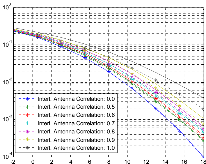
Figure 20: BER performance. TU50nFH1845. DTS-2 - With and without phase offset [26]
