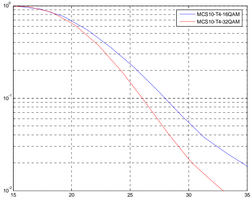
Figure 200: TU3iFH Sensitivity Performance (MCS-10)
