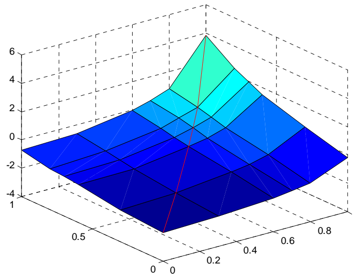
Figure 23: Impact of correlation in desired and interfere branch. DTS-1 - GMSK [26]
