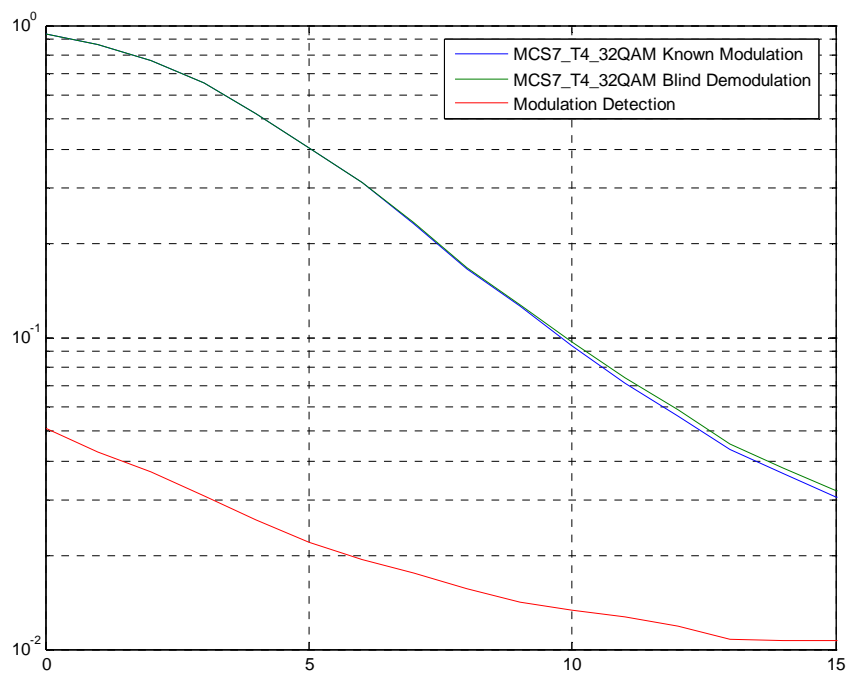
Figure C.23: MCS7-T4-32QAM, Sensitivity, HT100iFH
