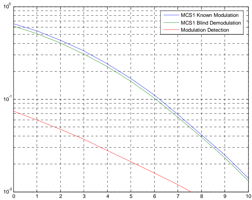
Figure C.8: MCS1, Co-channel, TU3iFH
