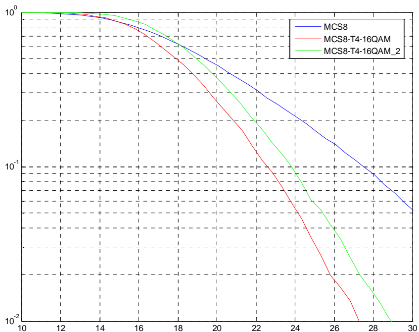
Figure 215: TU3iFH Sensitivity Performance (MCS-8)
