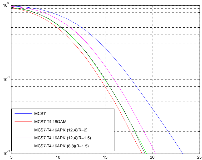
Figure 230: TU3iFH Co-Channel Performance (MCS-7)
