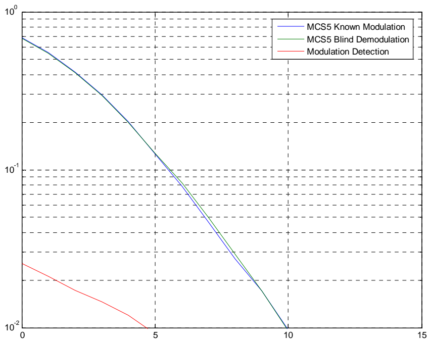
Figure C.21: MCS5, Sensitivity, HT100iFH
