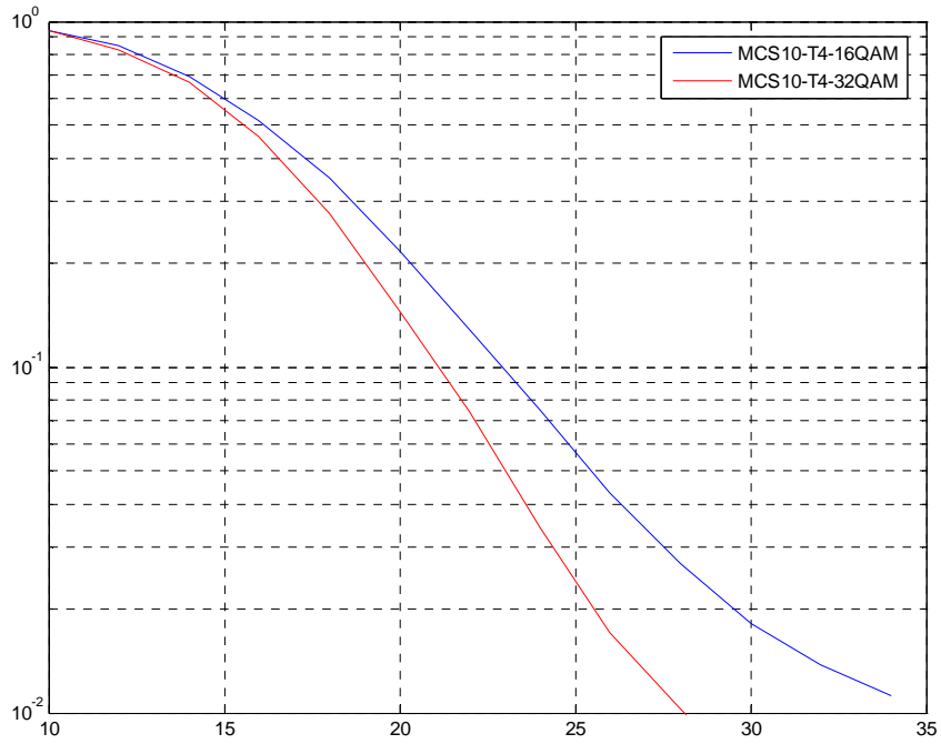
Figure 206: TU3iFH Co-Channel Performance (MCS-10)
