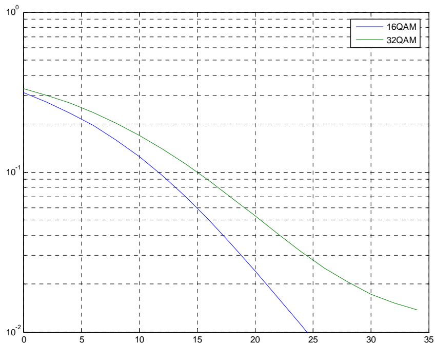
Figure 196: Uncoded BER of 16QAM and 32QAM Modulations
