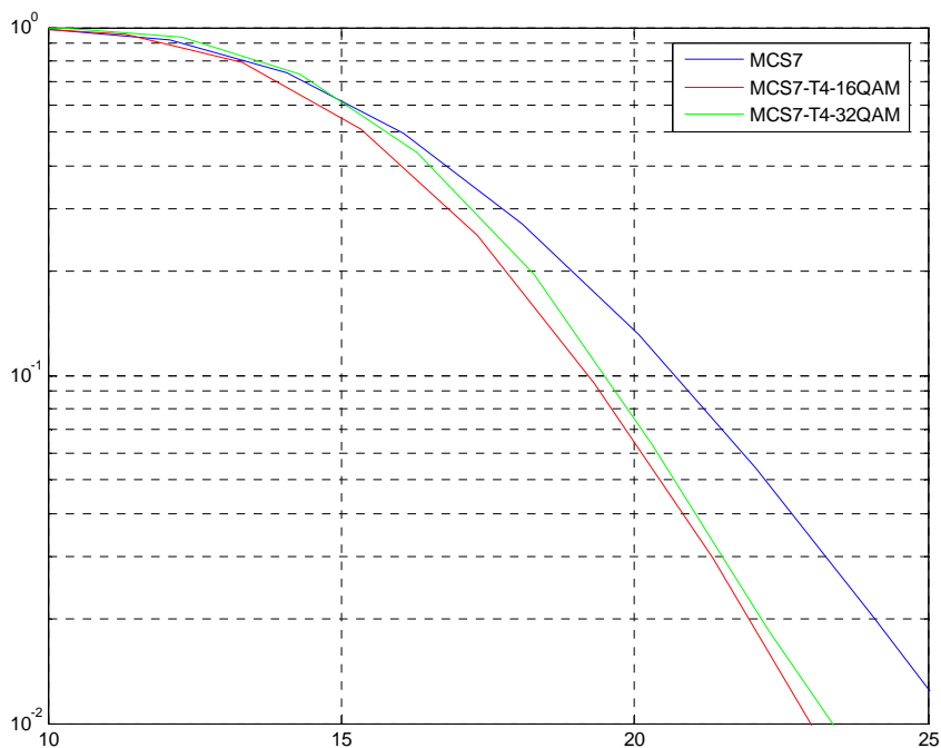
Figure 197: TU3iFH Sensitivity Performance (MCS-7)
