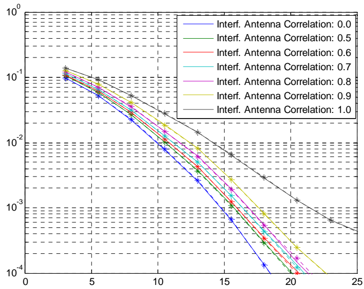
Figure 18: BER performance. TU50nFH1845. Sensitivity - With and without phase offset [26]
