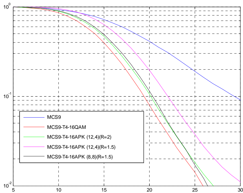
Figure 232: TU3iFH Co-Channel Performance (MCS-9)
