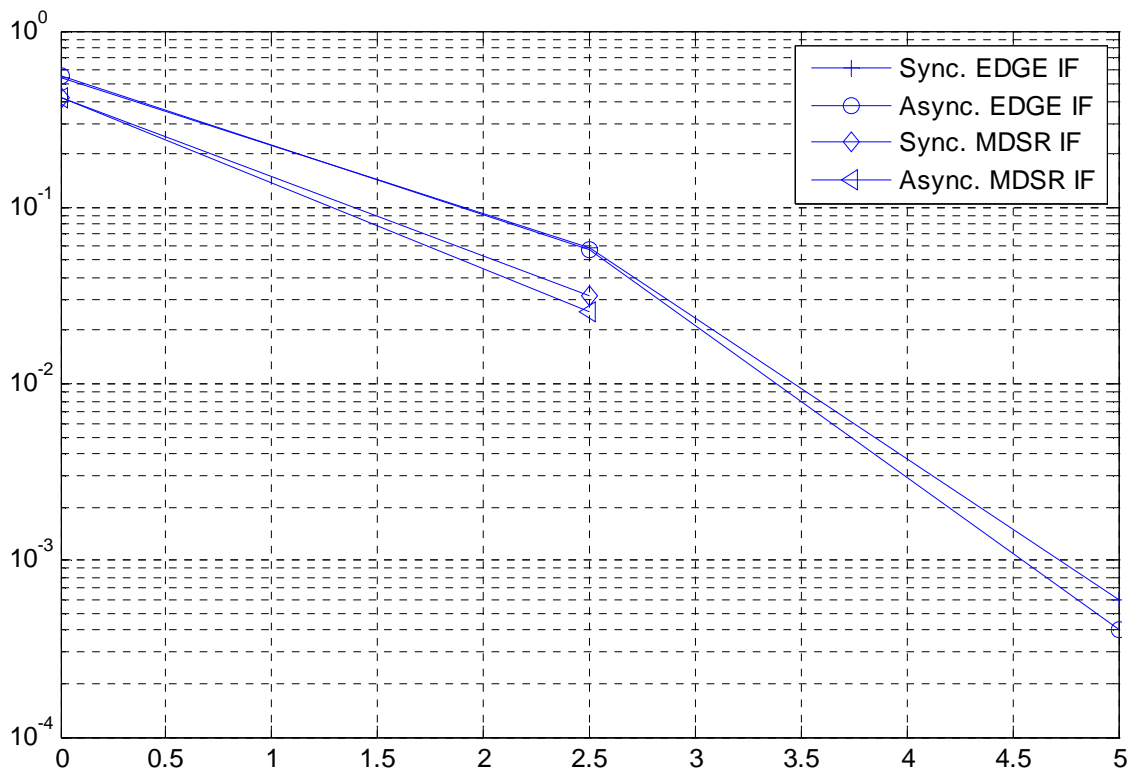
Figure 274: Voice performance at low SNR (noise power at 270 kHz equal to I_1 power)
