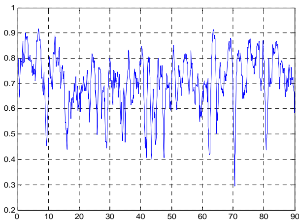
Figure 8: Antenna correlation values in steps of 100ms using a window width of 1s. C/I of 5 dB - TU3nFH945
