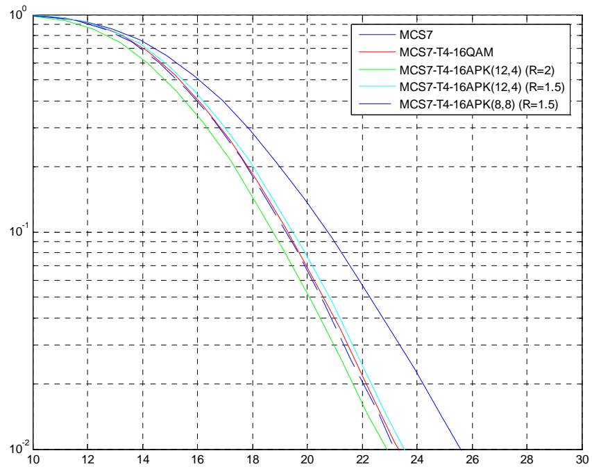
Figure 227: TU3iFH Sensitivity Performance (MCS-7)
