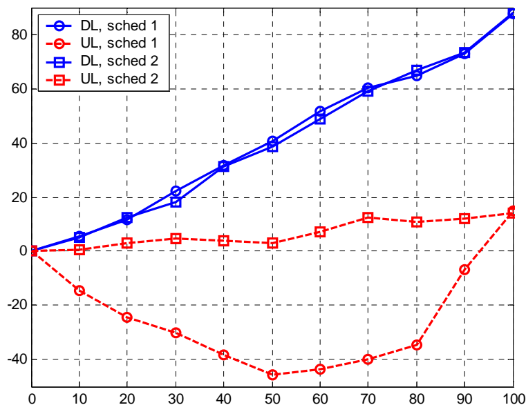
Figure 232h: CIR 35 dB, load factor: 80.0%, DL: 754.7 kbps/cell, UL: 754.7 kbps/cell.
