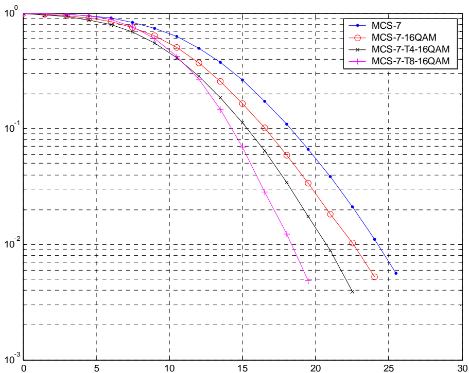
Figure C.3: TU50nH Co-Channel Performance (MCS-7)
