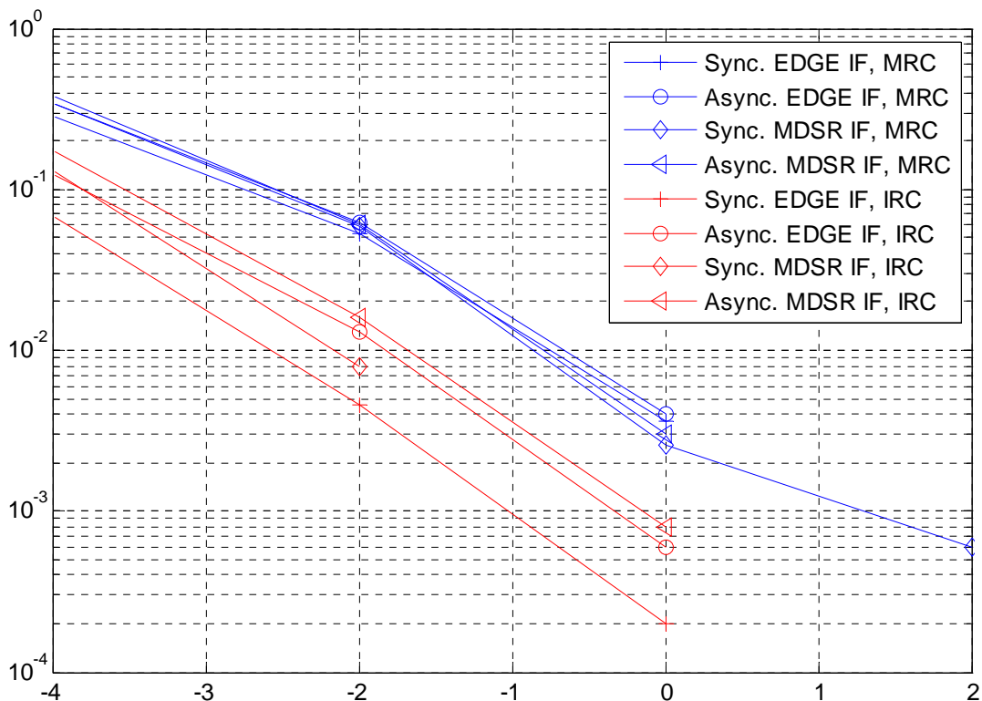
Figure 273: Voice impact with IRC and MRC
