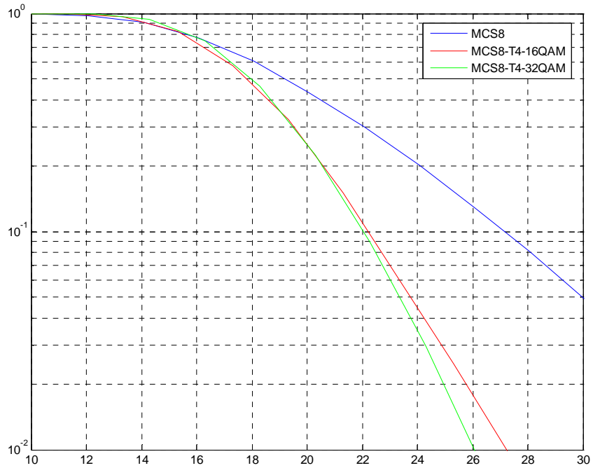
Figure 198: TU3iFH Sensitivity Performance (MCS-8)
