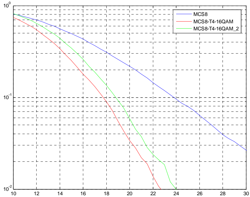
Figure 212: TU3iFH Co-Channel Performance (MCS-8)
