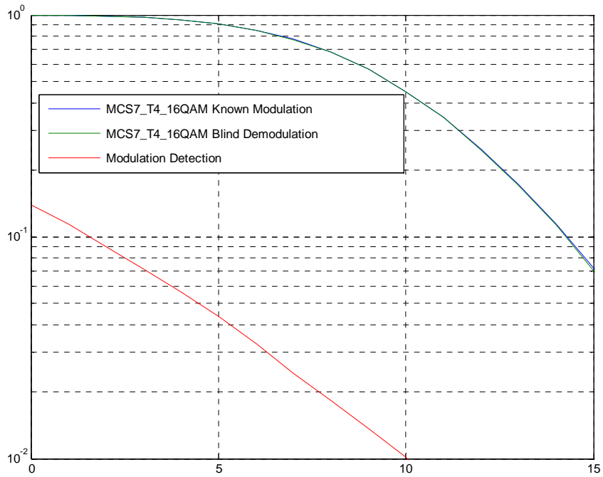
Figure C.14: MCS7-T4-16QAM, Co-channel, TU50iFH
