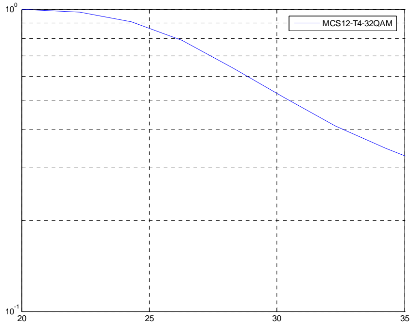
Figure 202: TU3iFH Sensitivity Performance (MCS-12)
