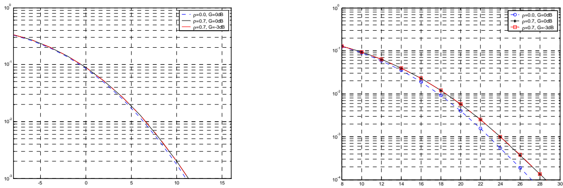
Figure 25: Uncoded BER of MS RX diversity for GMSK (left figure) and 8PSK (right figure), configuration 2 and different antenna gain imbalances and correlations [21]
