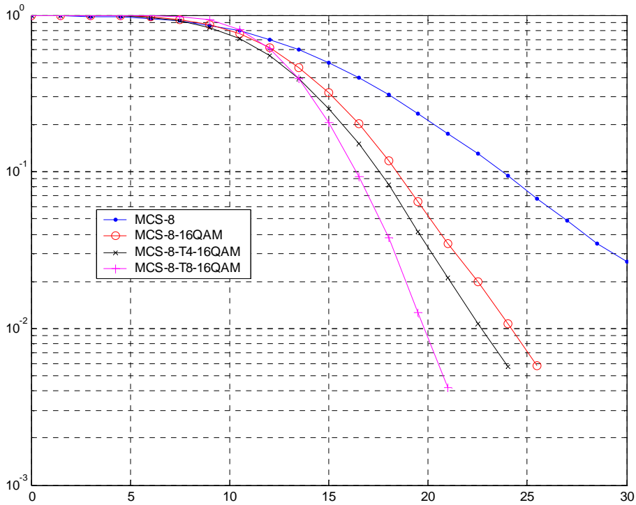
Figure 159: TU3iFH Co-Channel Performance (MCS-8)
