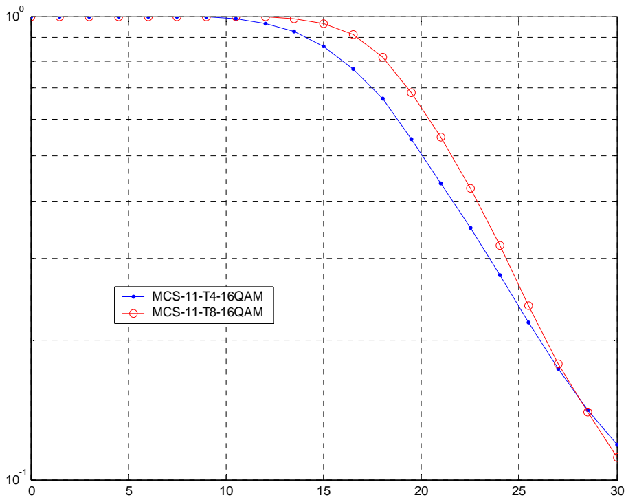
Figure 162: TU3iFH Co-Channel Performance (MCS-11 16-QAM)
