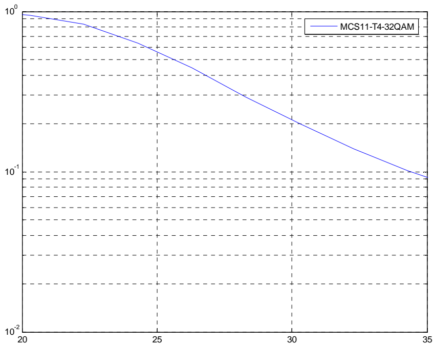
Figure 201: TU3iFH Sensitivity Performance (MCS-11)
