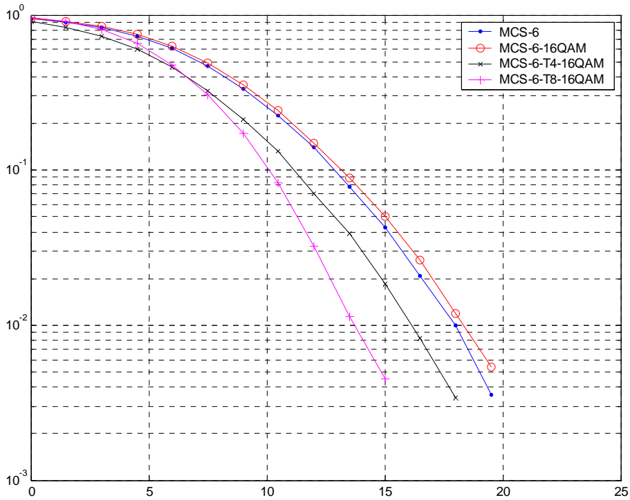
Figure C.2: TU50nH Co-Channel Performance (MCS-6)
