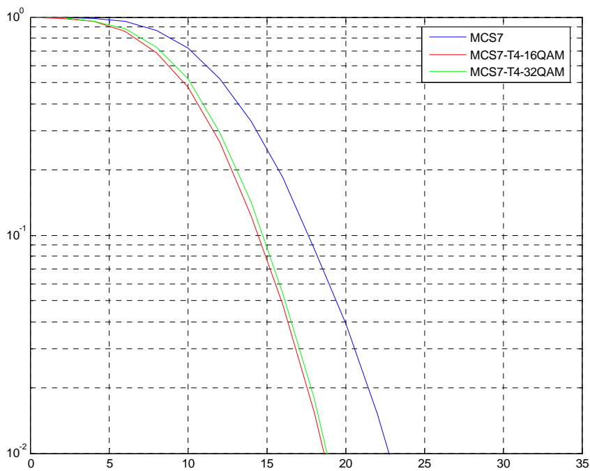
Figure 203: TU3iFH Co-Channel Performance (MCS-7)
