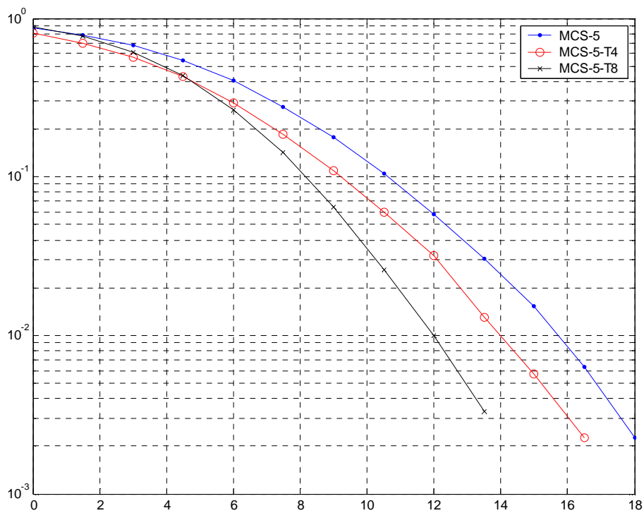
Figure C.1: TU50nH Co-Channel Performance (MCS-5)
