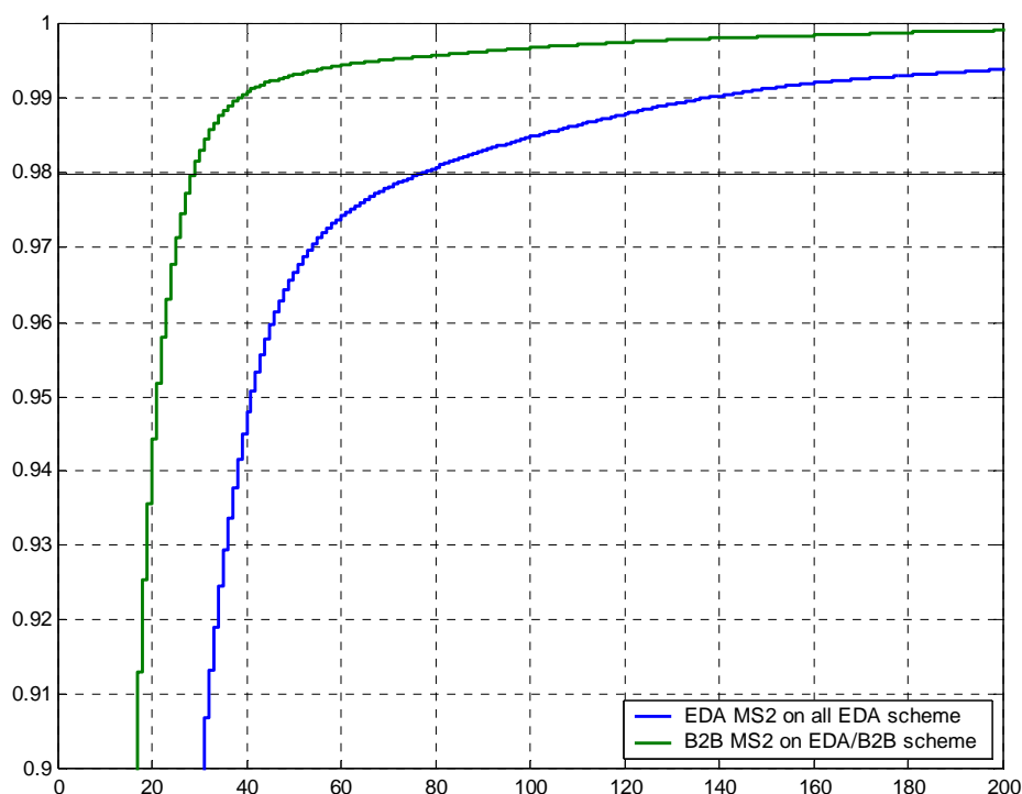
Figure 404: CDF of transmission buffer length for MS2 (MCS-5, CIF 15 FPS)
