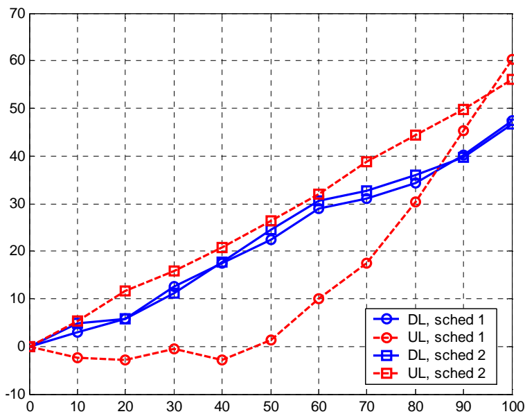
Figure 232i: CIR 15 dB, load factor: 70.0%, DL: 314.9 kbps/cell, UL: 314.9 kbps/cell.
