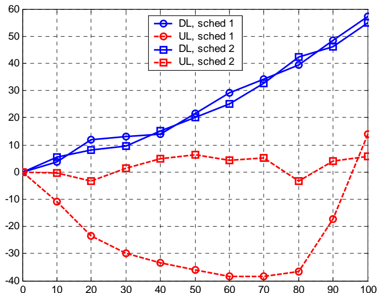
Figure 232g: CIR: 15 dB, load factor: 80.0%, DL: 359.9 kbps/cell, UL: 359.9 kbps/cell.
