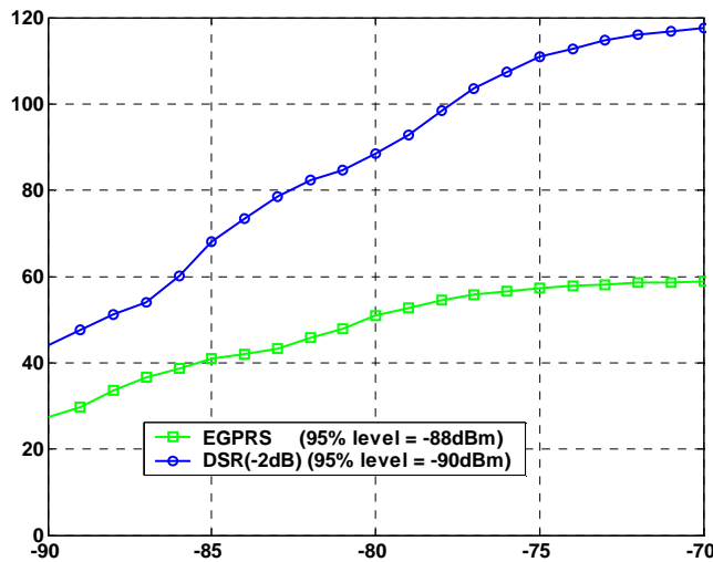
Figure 261: Throughput per TSL for DSR and EGPRS for reuse 1/3
