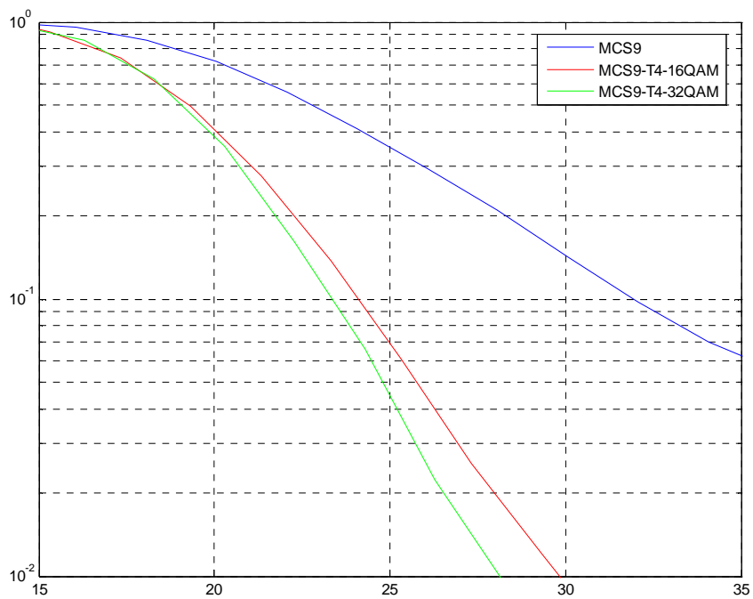
Figure 199: TU3iFH Sensitivity Performance (MCS-9)
