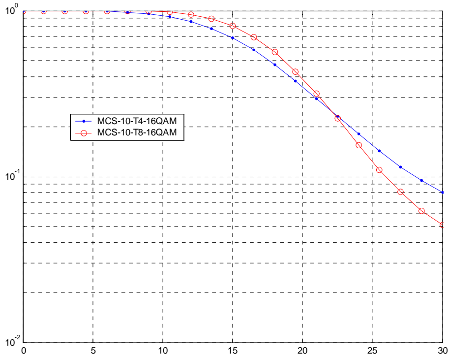
Figure C.6: TU50nH Co-Channel Performance (MCS-10 16-QAM)
