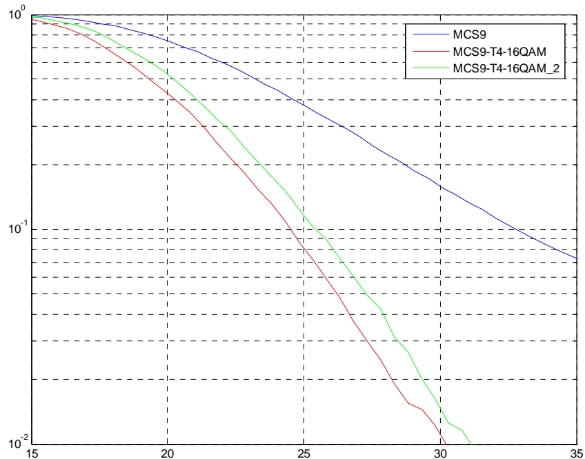
Figure 216: TU3iFH Sensitivity Performance (MCS-9)
