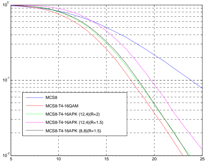
Figure 231: TU3iFH Co-Channel Performance (MCS-8)
