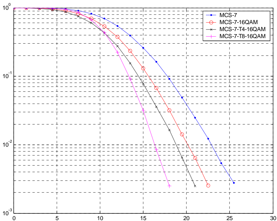
Figure 158: TU3iFH Co-Channel Performance (MCS-7)
