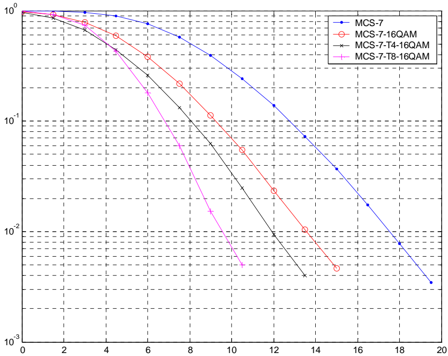
Figure 165: TU3iFH Sensitivity Performance (MCS-7)
