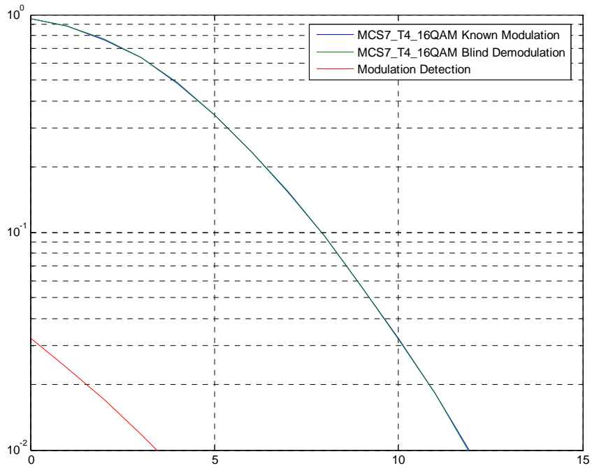
Figure C.18: MCS7-T4-16QAM, Sensitivity, TU50iFH
