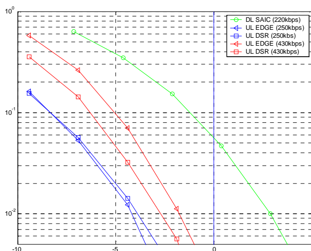
Figure 256: TCH/AFS5.9 FER at re-use 1/1
