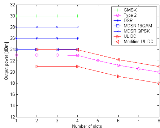
Figure 78: TX power with multislot profile 3
