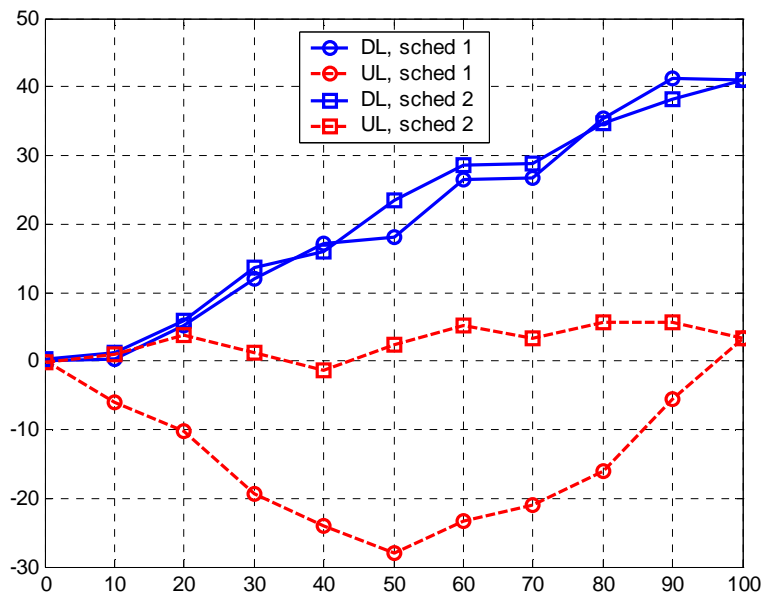
Figure 232e: CIR 15 dB, load factor: 70.0%, DL: 314.9 kbps/cell, UL: 314.9 kbps/cell.
