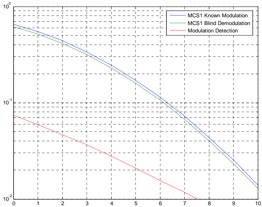
Figure C.12: MCS1, Co-channel, TU50iFH
