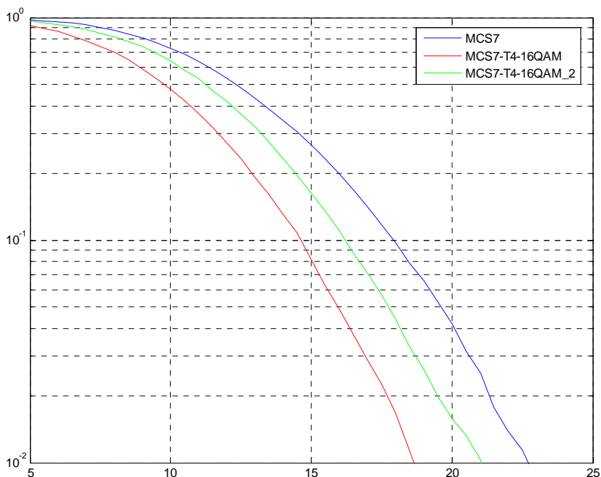
Figure 211: TU3iFH Co-Channel Performance (MCS-7)
