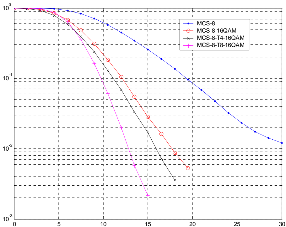
Figure 166: TU3iFH Sensitivity Performance (MCS-8)
