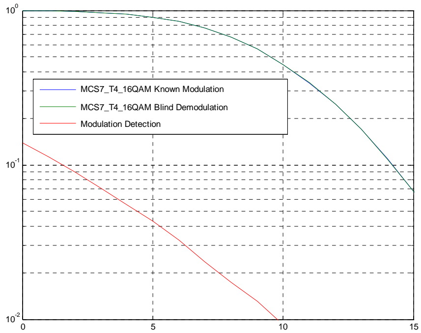
Figure C.10: MCS7-T4-16QAM, Co-channel, TU3iFH
