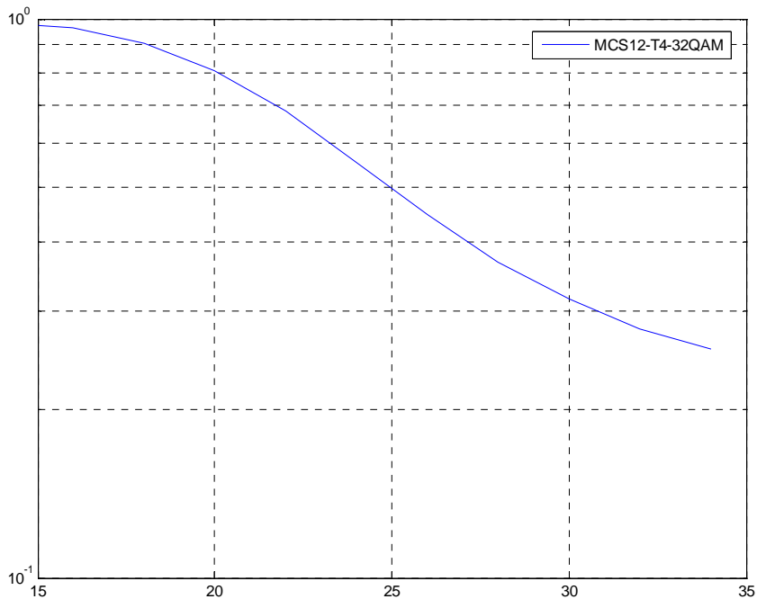
Figure 208: TU3iFH Co-Channel Performance (MCS-12)
