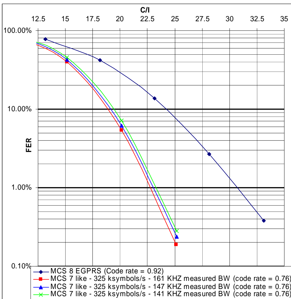
Figure 232.b1: Expected performance of higher symbol rate coding schemes
