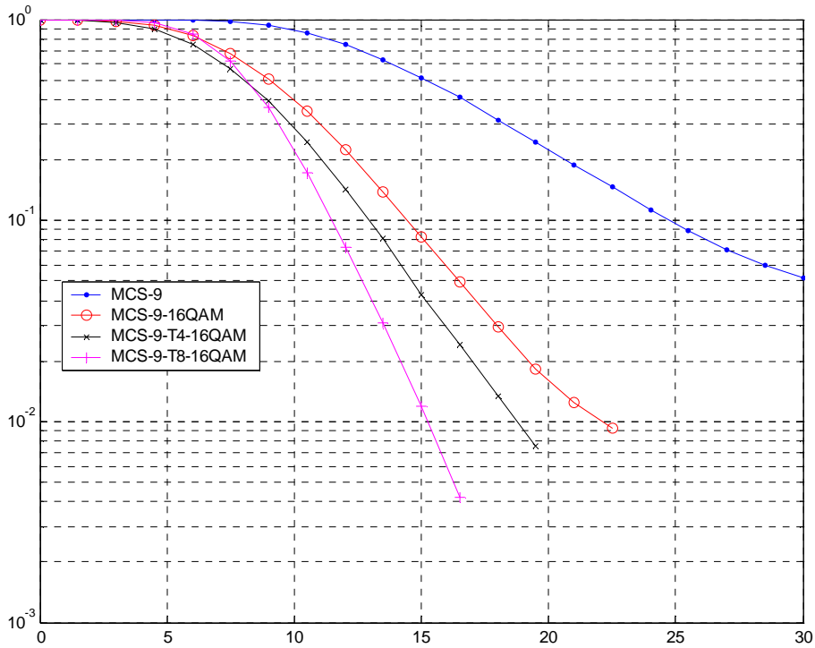
Figure 167: TU3iFH Sensitivity Performance (MCS-9)
