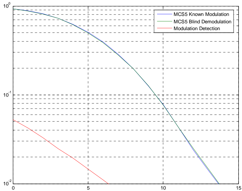
Figure C.9: MCS5, Co-channel, TU3iFH
