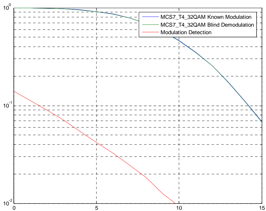
Figure C.15: MCS7-T4-32QAM, Co-channel, TU50iFH
