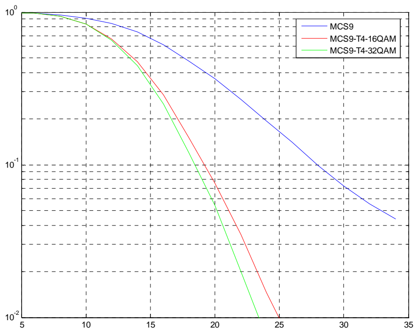
Figure 205: TU3iFH Co-Channel Performance (MCS-9)
