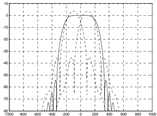
Figure 238: MDSR spectrum
