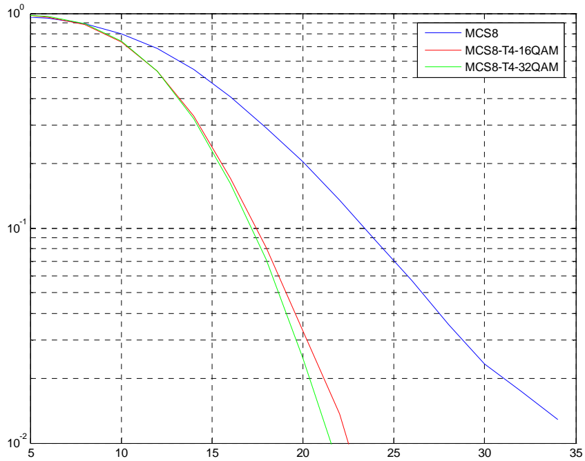
Figure 204: TU3iFH Co-Channel Performance (MCS-8)
