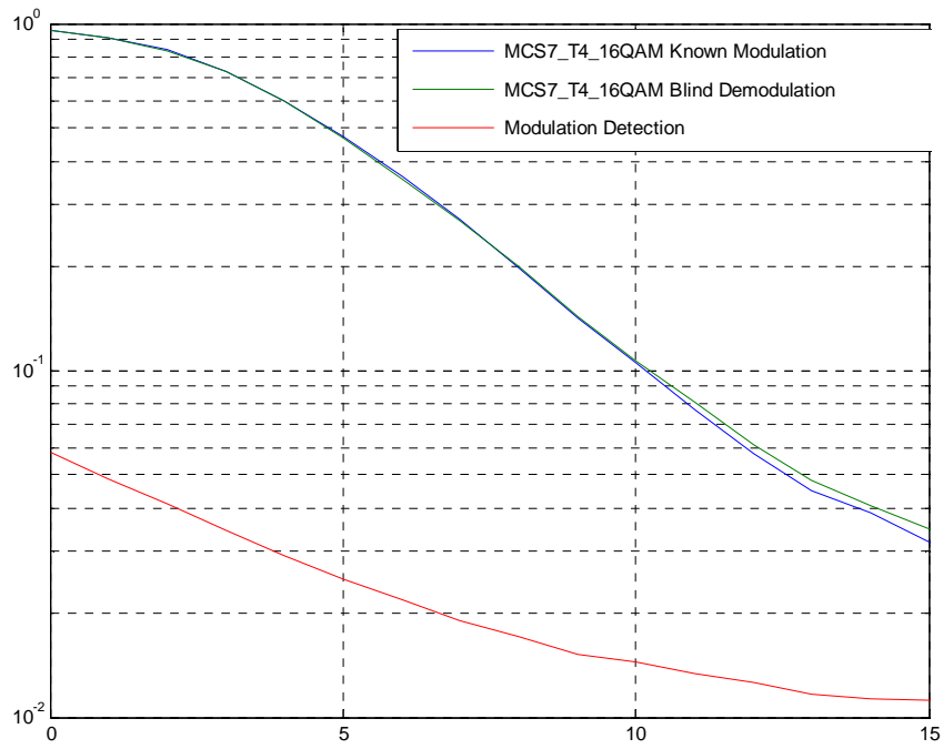
Figure C.22: MCS7-T4-16QAM, Sensitivity, HT100iFH
