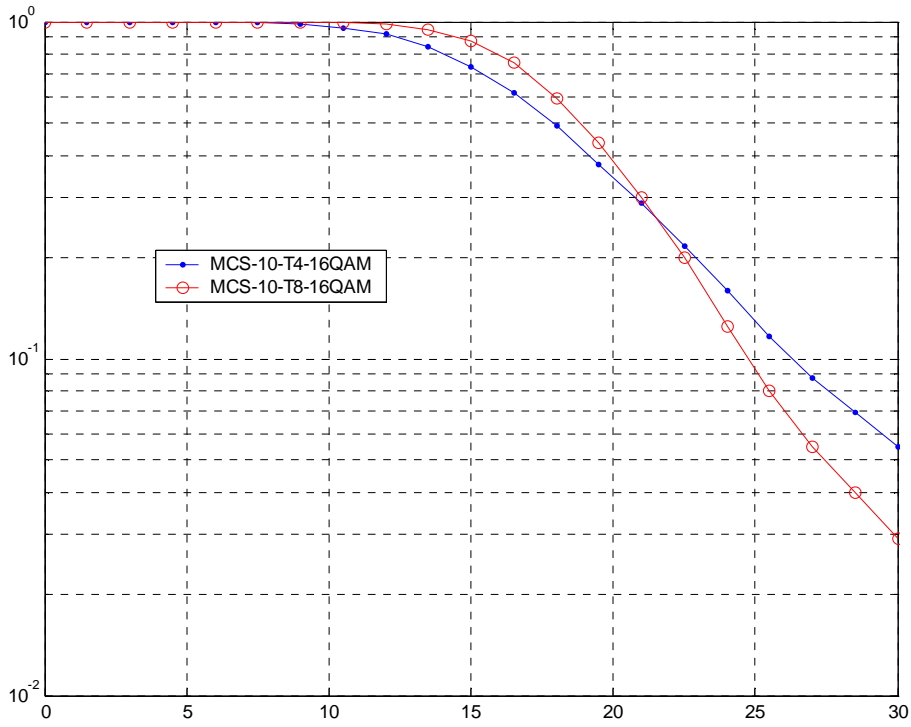
Figure 161: TU3iFH Co-Channel Performance (MCS-10 16-QAM)
