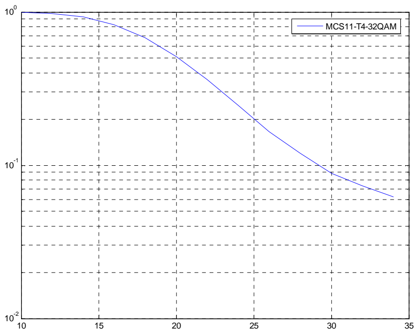
Figure 207: TU3iFH Co-Channel Performance (MCS-11)
