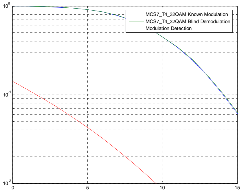
Figure C.11: MCS7-T4-32QAM, Co-channel, TU3iFH
