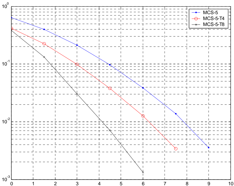
Figure 163: TU3iFH Sensitivity Performance (MCS-5)
