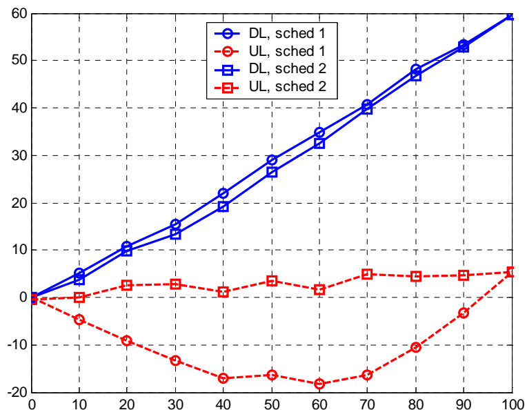
Figure 232f: CIR: 35 dB, load factor: 70.0%, DL: 660.4 kbps/cell, UL: 660.4 kbps/cell.
