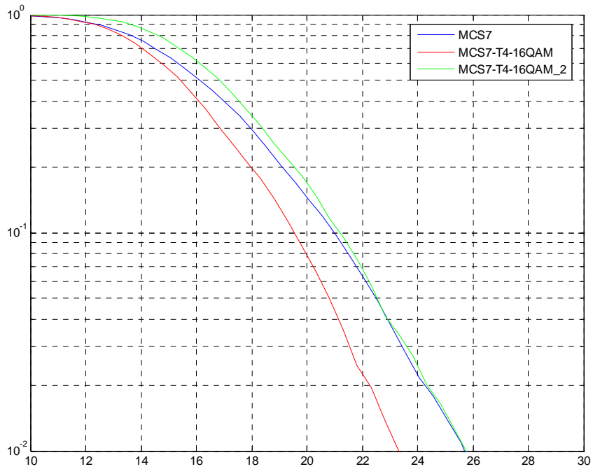
Figure 214: TU3iFH Sensitivity Performance (MCS-7)
