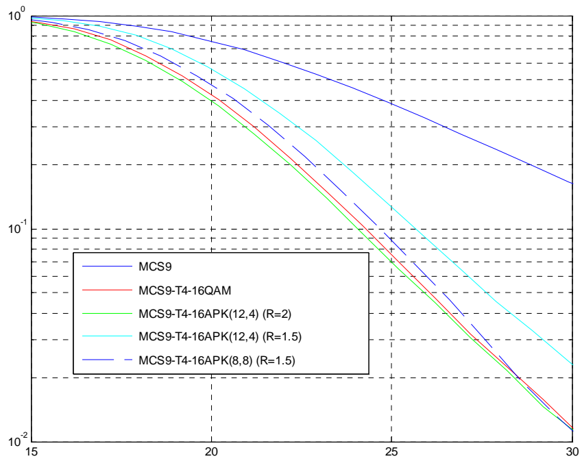
Figure 229: TU3iFH Sensitivity Performance (MCS-9)
