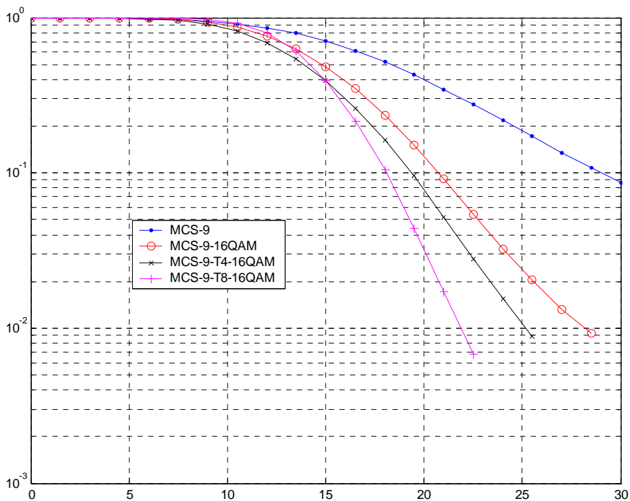
Figure 160: TU3iFH Co-Channel Performance (MCS-9)
