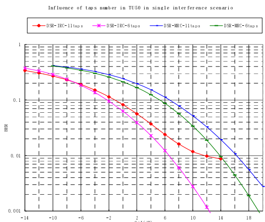
Figure 284: Influence of DSR receiver taps number in TU50 at single interference scenario using two antennas
