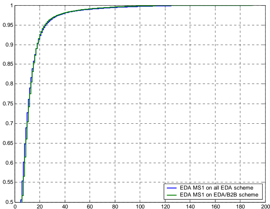
Figure 402: CDF of transmission buffer length for MS1
