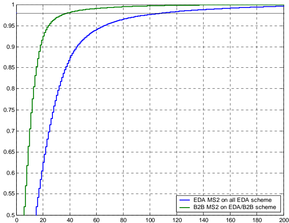
Figure 401: CDF of transmission buffer length for MS2 (QCIF 30 FPS)
