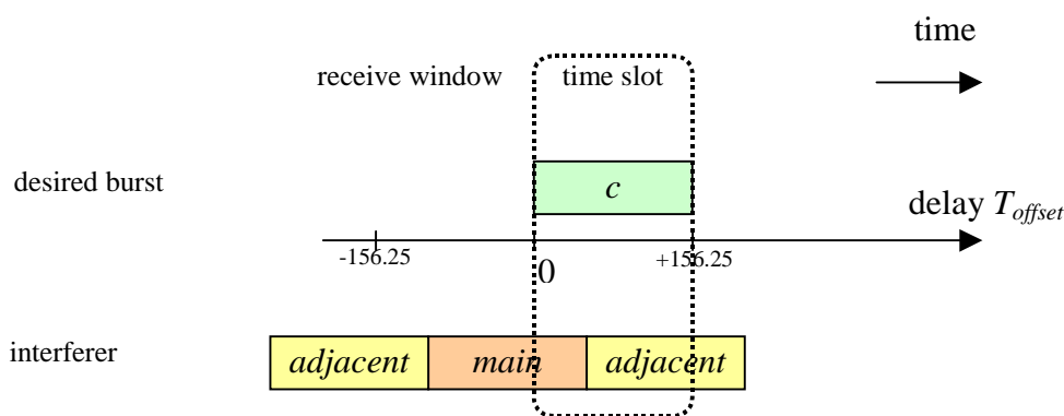
Figure 5-6 Interferer burst structure.
