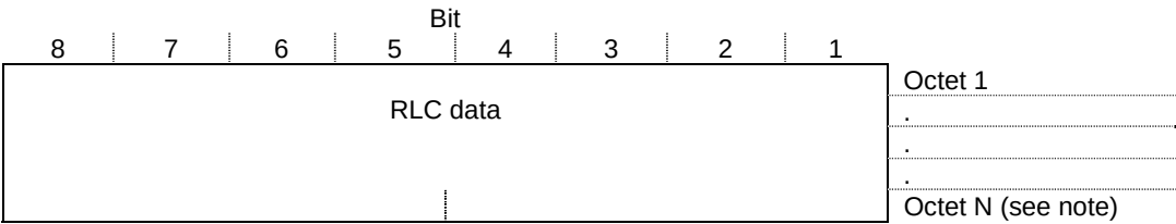
NOTE: the RLC data may contain a non-integer number of octets. N \geq 1 Figure 14: Uplink RLC/MAC block for data transfer in RLC transparent mode
