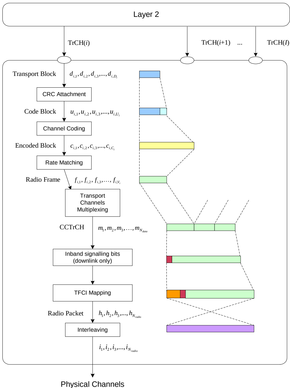
Figure 2: FLO Architecture
