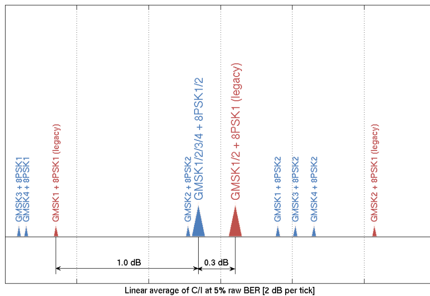
Figure 10. Breakdown of CCI case with C: GMSK, I: 8PSK.
