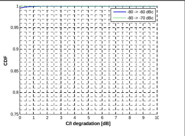
Figure 24. C/I degradation CDF comparing relaxed IM requirement to -60 and -70 dBc.
