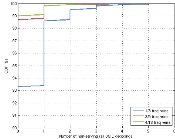
Figure ZF.5.2-4: Likelihood of decoding the BSIC of a neighboring cell
