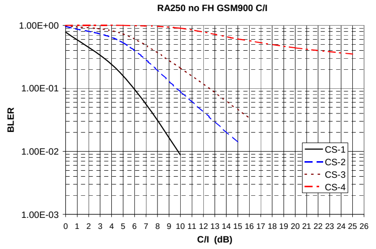
Figure 4: BLER vs. C/I_c , RA250 no FH, GSM900
