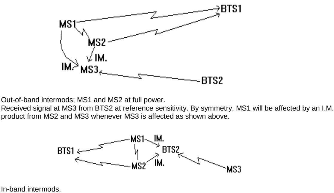
Figure 4.1: Intermodulation between MS
