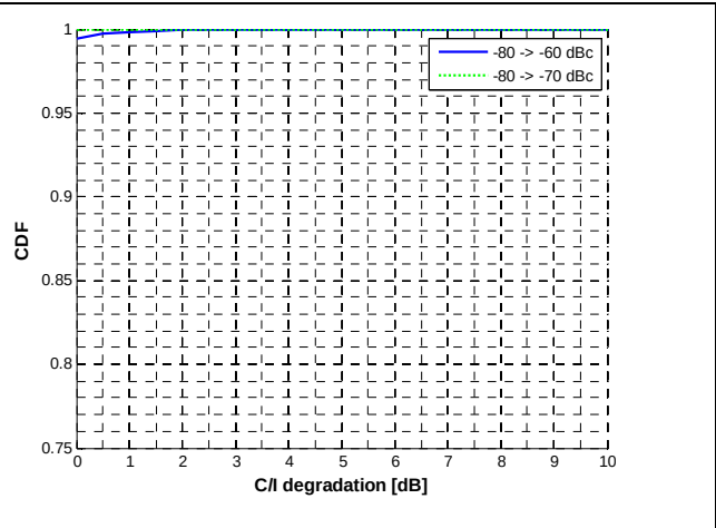
Figure 28. C/I degradation CDF comparing relaxed IM requirement to -60 and -70 dBc.
