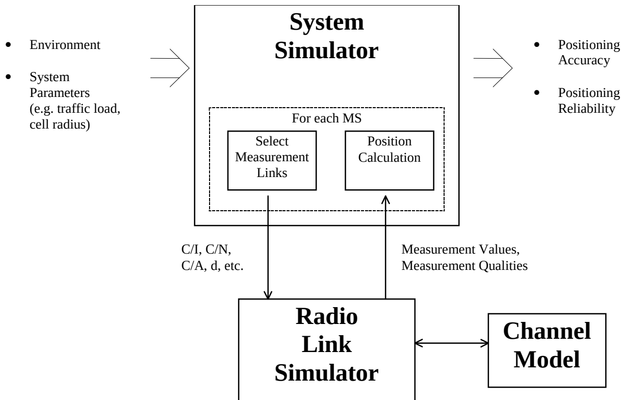
Figure 2.1: Positioning Simulator
