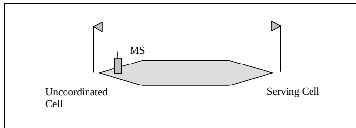
Figure X.10: Relative geometry for inter/intra modulation analysis
