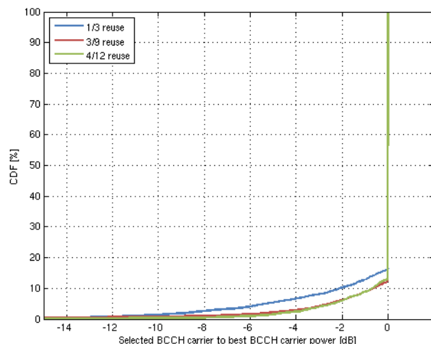
Figure 24.2.2-2: Selected BCCH carrier to best BCCH carrier power ratio
