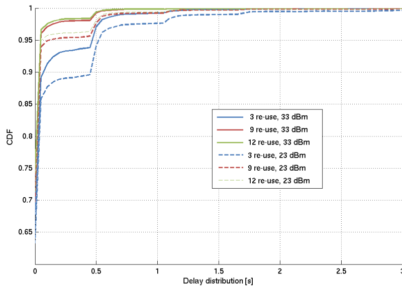
Figure ZF.6.2-1: Common Control Signaling Delay
