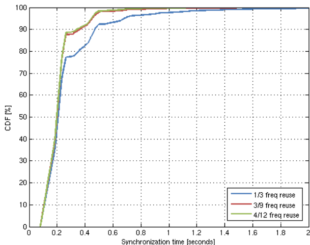
Figure ZF.5.2-1: Total time to synchronization for 1/3, 3/9 and 4/12 frequency reuse
