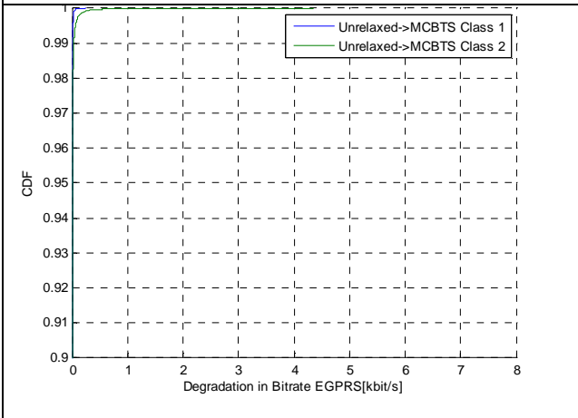
Figure 11 Throughput Degradation CDF of EGPRS comparing different relaxation levels
