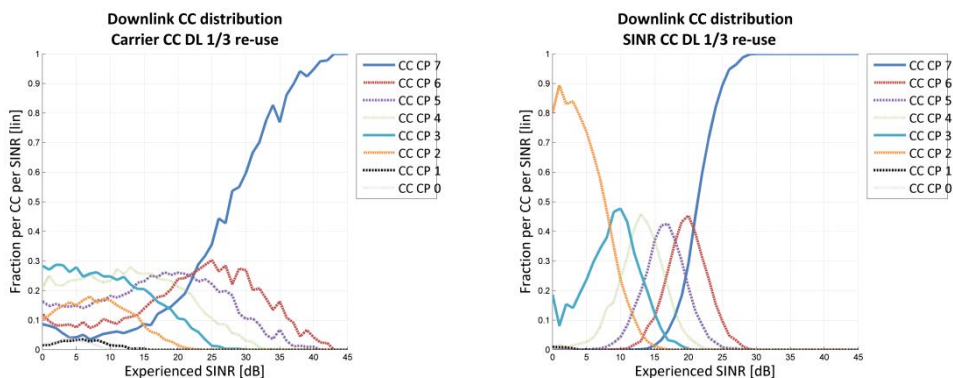
Figure ZF.7.2-4: Downlink Coverage class distribution for 23 dBm. Carrier SS based (left), SINR based (right)
