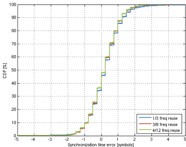
Figure ZF.5.2-2: Synchronization time error after FCCH detection.
