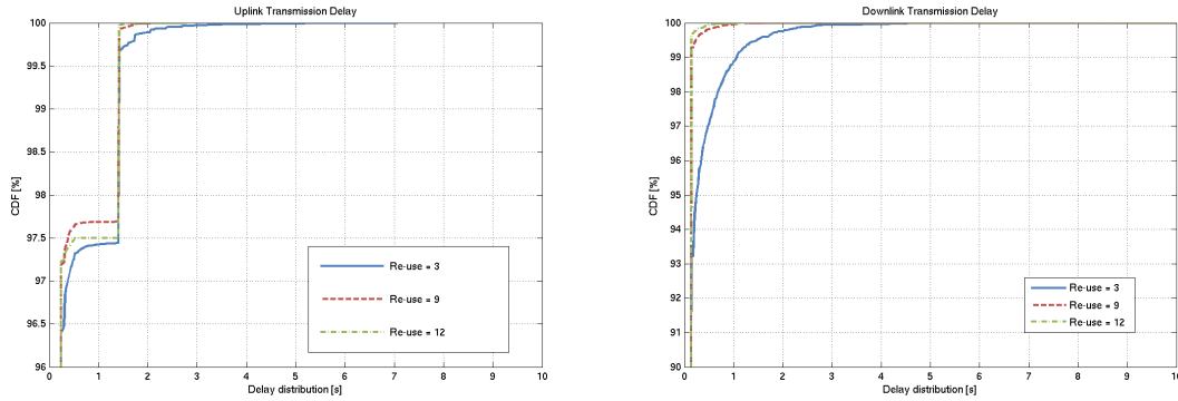
Figure 24.2.4-1: Uplink (left) and downlink (right) transmission delay for 33 dBm
