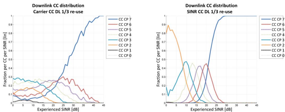
Figure ZF.7.2-4: Downlink Coverage class distribution for 23 dBm.
