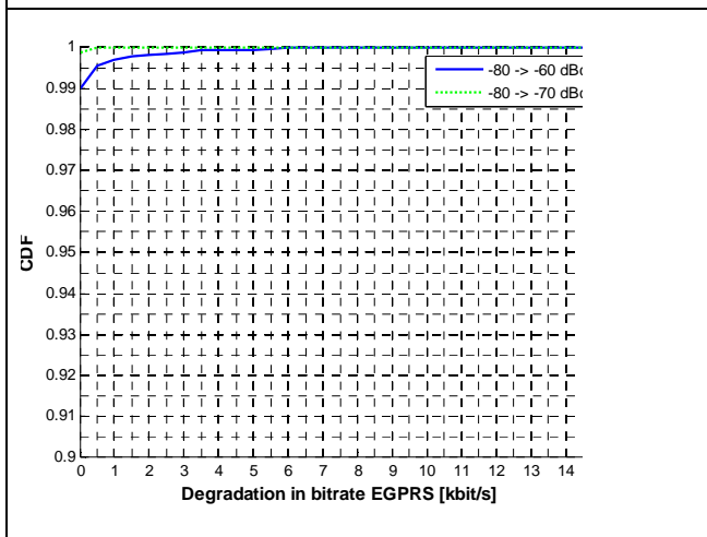
Figure 25. EGRPS bitrate degradation CDF comparing relaxed IM requirement to -60 and -70 dBc.
