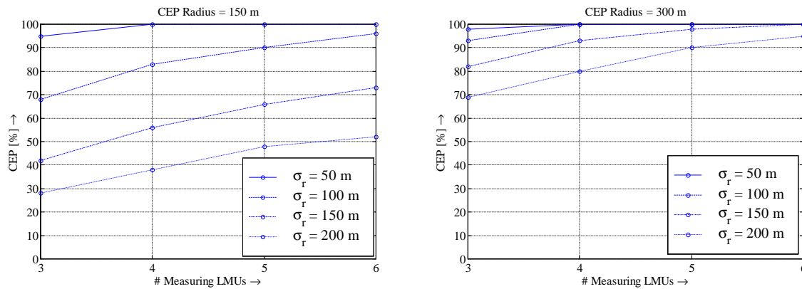
Figure V.4.3: Circular Error probability for various CEP radii
