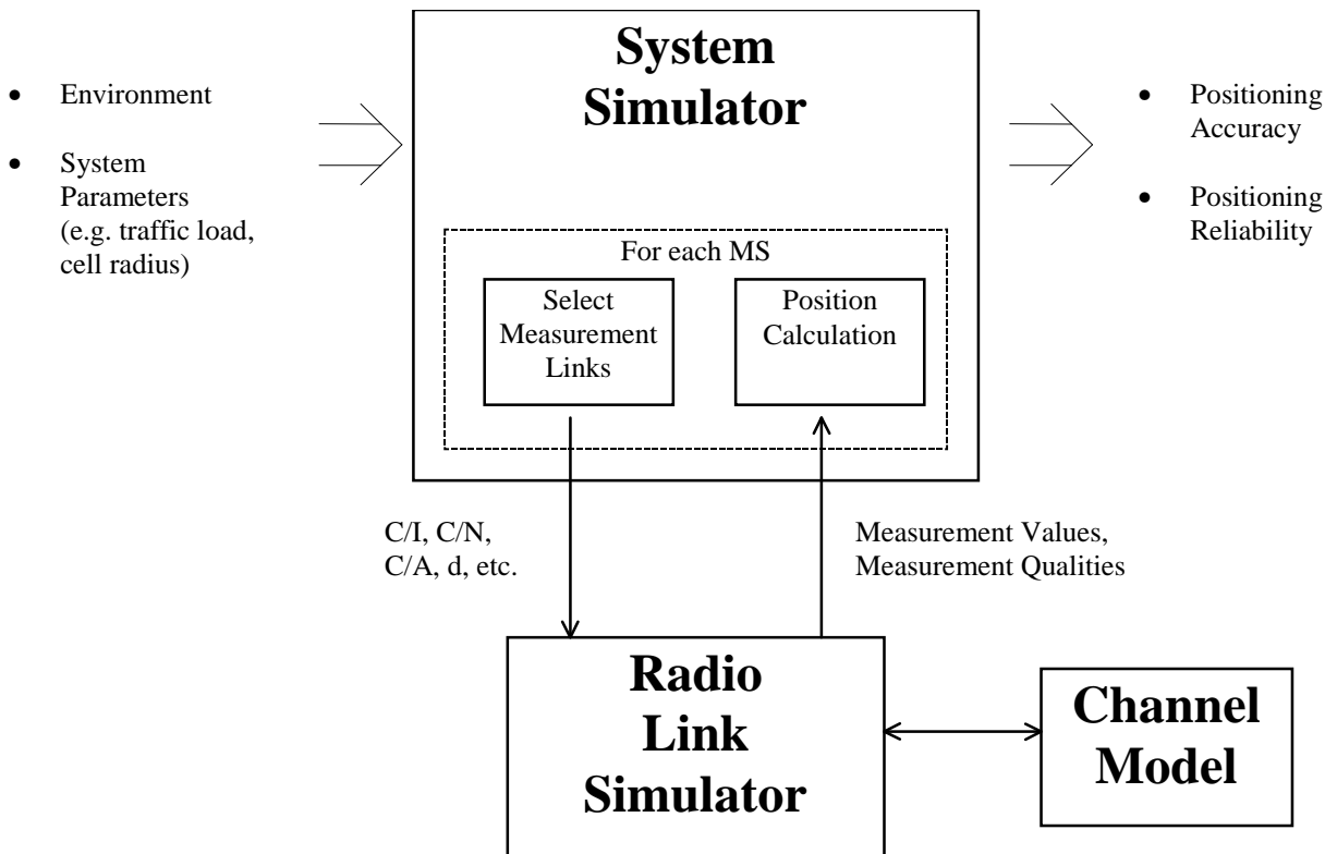
Figure 2.1: Positioning Simulator
