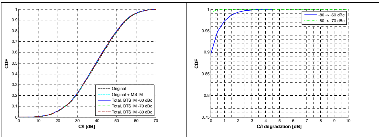
Figure 13. C/I CDF comparing MCPA IM
