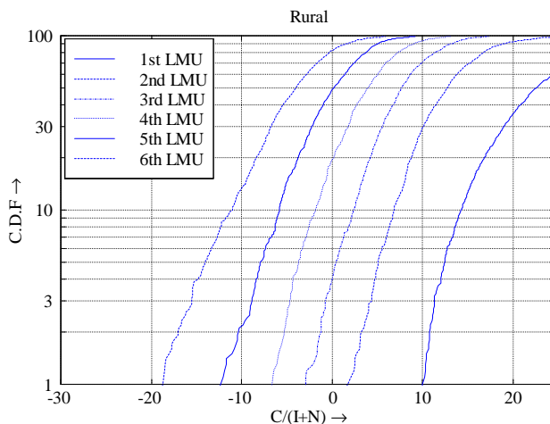
Figure V.4.2: C/(I+N) distribution in Rural environment
