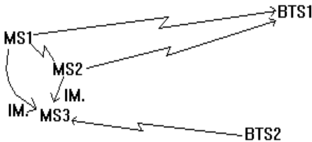
Out-of-band intermods; MS1 and MS2 at full power. Received signal at MS3 from BTS2 at reference sensitivity. By symmetry, MS1 will be affected by an I.M. product from MS2 and MS3 whenever MS3 is affected as shown above.
