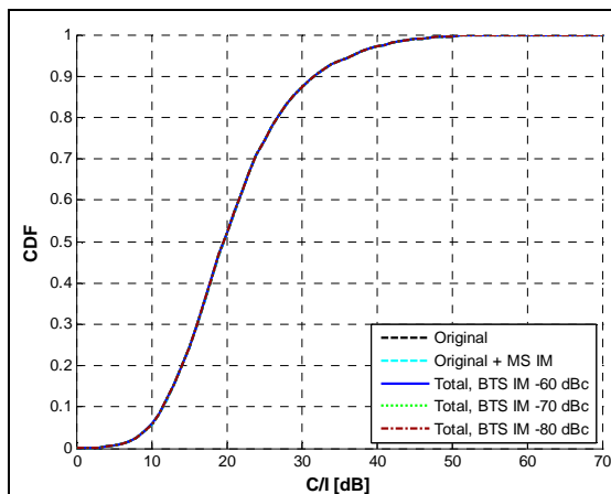
Figure 23. C/I CDF comparing MCPA IM requirements -60, -70 and -80 dBc.
