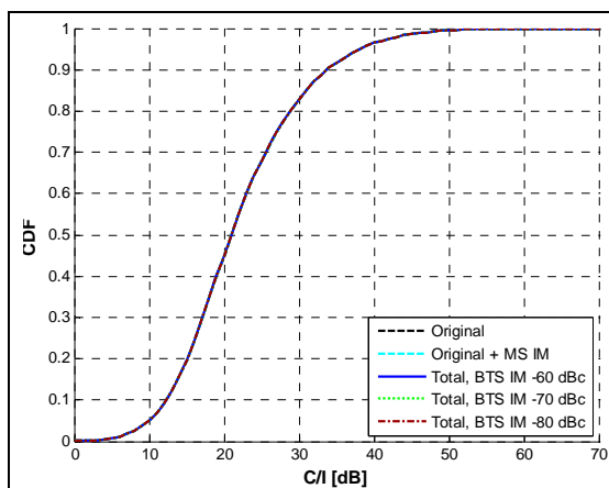
Figure 27. C/I CDF comparing MCPA IM requirements -60, -70 and -80 dBc.
