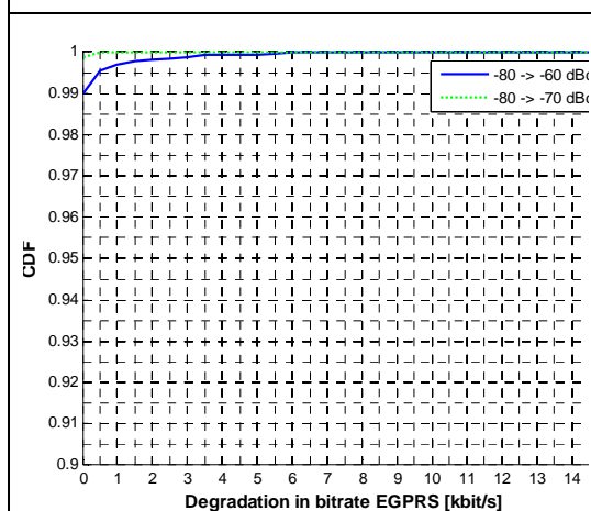
Figure 25. EGRPS bitrate degradation CDF comparing relaxed IM requirement to -60 and -70 dBc.
