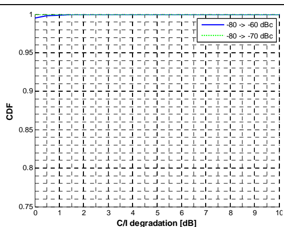
Figure 24. C/I degradation CDF comparing relaxed IM requirement to -60 and -70 dBc.
