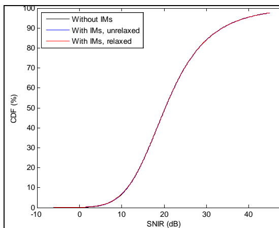
Figure 1: CDF vs. SNIR calculated in the macro cell scenario.
