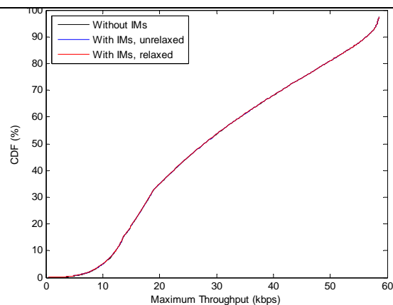
Figure 2: CDF vs. maximum EGPRS throughput calculated in the macro cell scenario.
