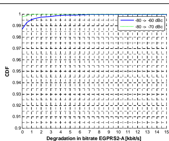
Figure 26. EGRPS2-A bitrate degradation CDF comparing relaxed IM requirement to -60 and -70 dBc.
