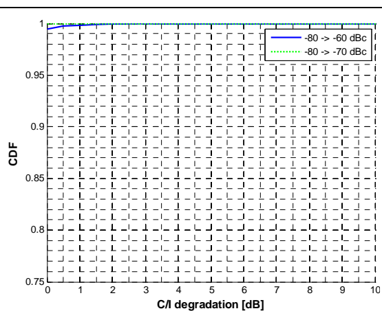
Figure 28. C/I degradation CDF comparing relaxed IM requirement to -60 and -70 dBc.
