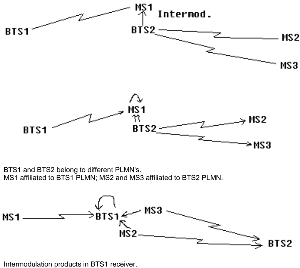
Figure 3.2: Intermodulation
