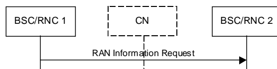
Figure 6.2.2.a: RAN Information Request procedure.
