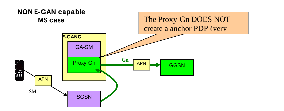
Figure 21: Non EGAN capable terminal
