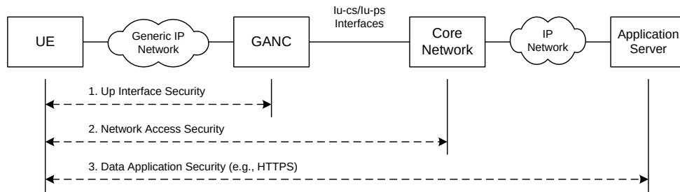
Figure 53: Iu mode GAN Security Mechanisms
