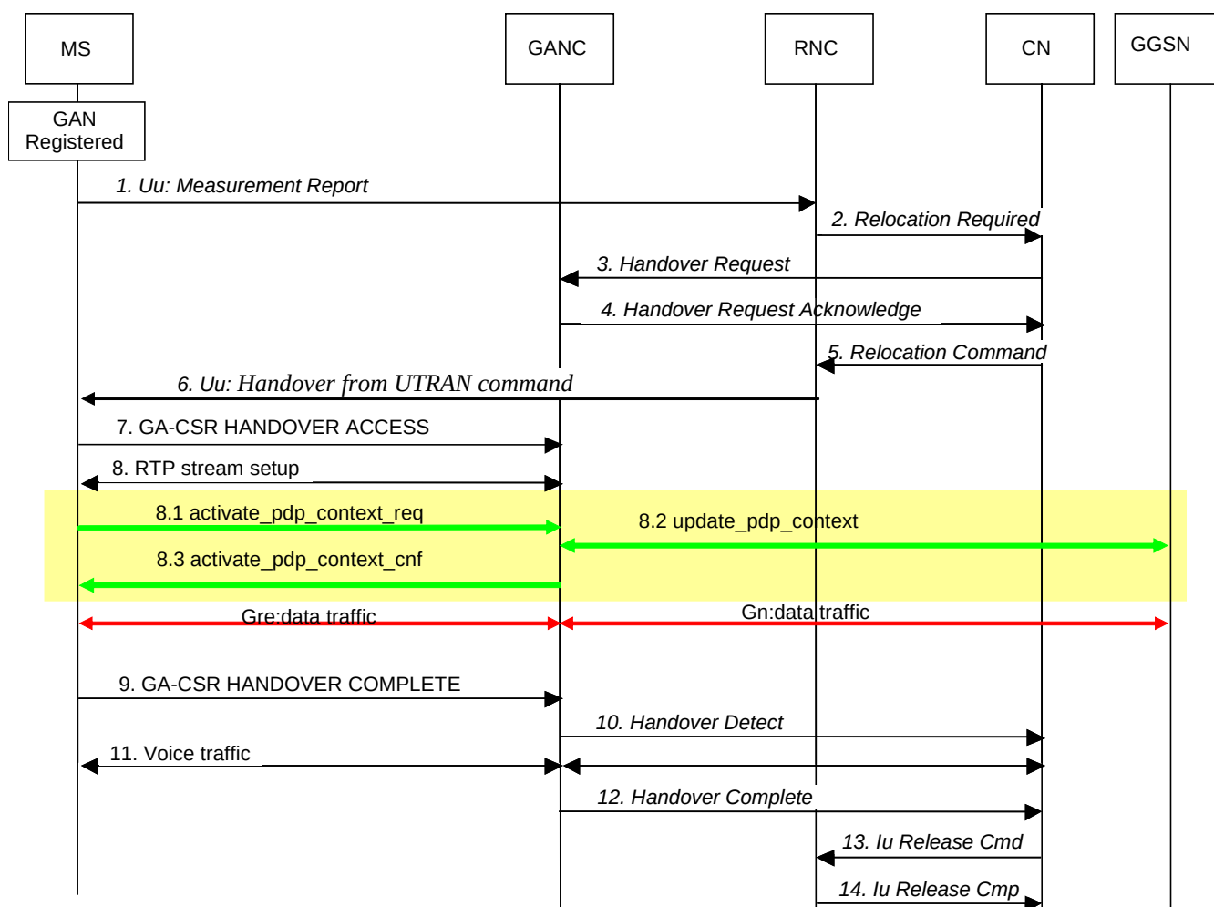
Figure 15: UTRAN to EGAN CS+PS handover procedure
