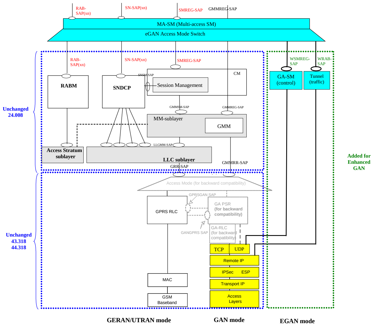
Figure 34: UMTS-GSM-GPRS-GAN terminal
