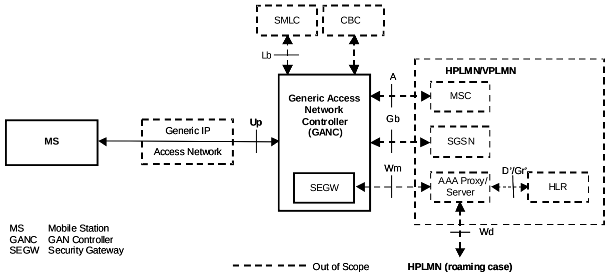
Figure 40: Existing architecture
