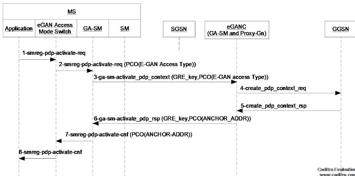
Figure 9: PDP context activation procedure in EGAN mode
