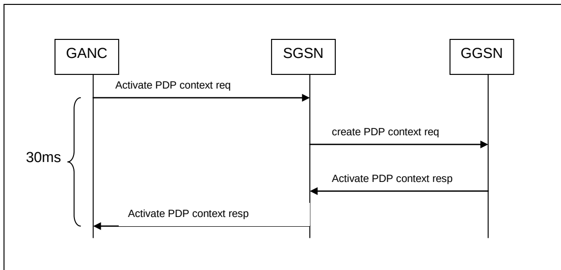
Figure 39: Signalling delay
