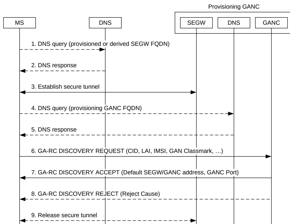
Figure 54: Discovery procedure
