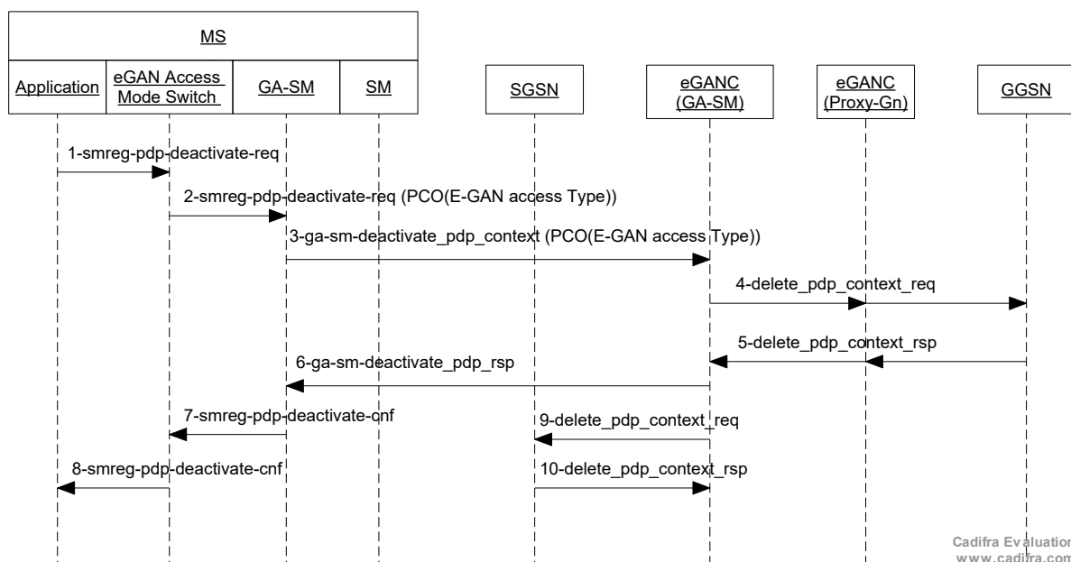
Figure 10: PDP context deactivation procedure on EGAN mode
