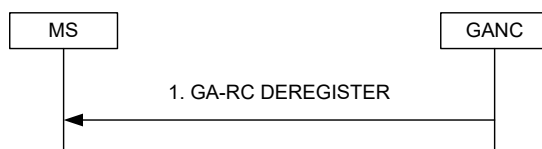
Figure 57: De-Registration initiated by the GANC
