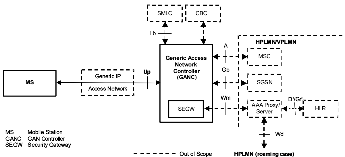
Figure 40: Existing architecture
