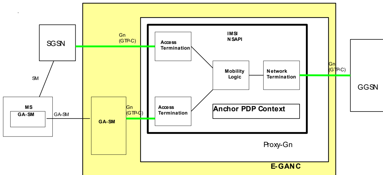
Figure 6: EGANC architecture
