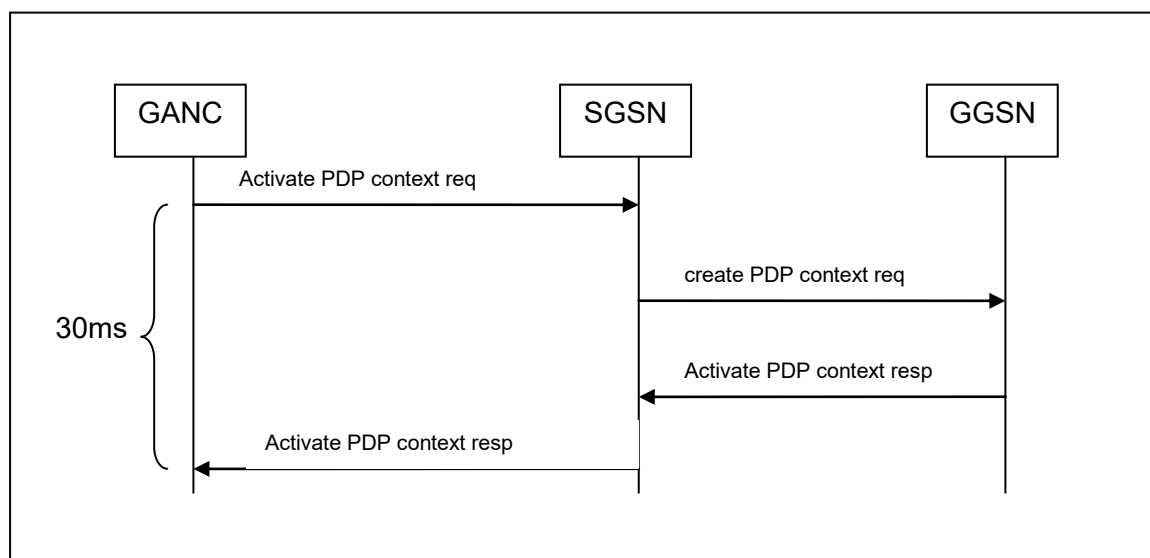
Figure 39: Signalling delay
