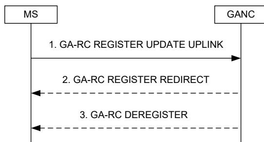
Figure X58: Registration Update Uplink
