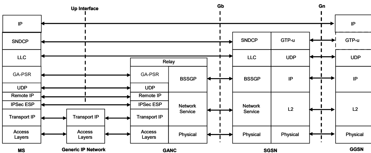
Figure 44: Existing PS user plane architecture
