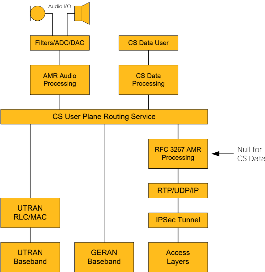
Figure 89: CS User Plane (Before)
