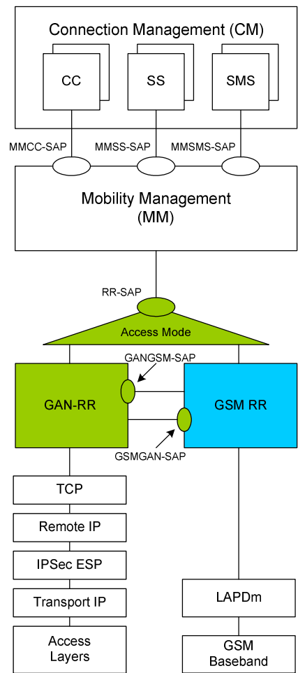
Figure 5.2.1.1.2: MS CS domain signalling architecture
