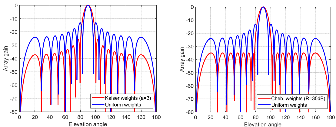
Figure 9.2.2-1: Examples for amplitude weighting/tapering: left: Kaiser ( a=3 ), right: Chebwin ( R=35\text{dB} )
