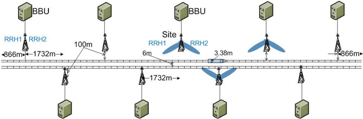
Figure 6.1.5-1: 4 GHz deployment
