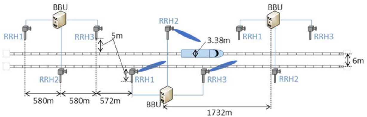
Figure 6.1.5-2: 30 GHz deployment
