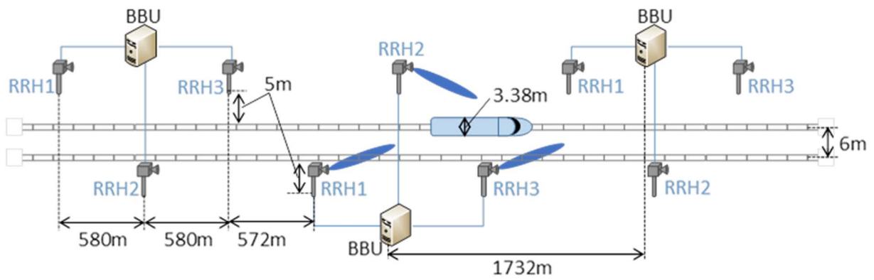
Figure 6.1.5-2: 30 GHz deployment
