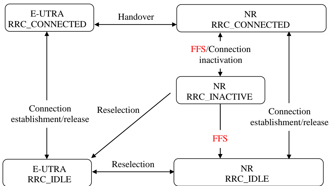
Figure 13.2.2-2: UE state machine and state transitions between NR and E-UTRAN
