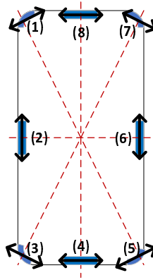
Figure 7.3-7: Handheld UT antenna positions and orientations for one antenna field pattern (top-down view)
