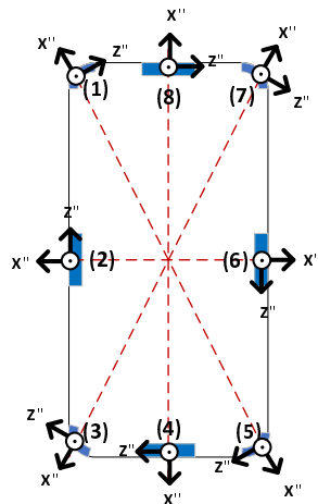
Figure 7.3-9: Handheld UT antenna coordinate systems used for channel model calibration for one antenna field pattern (top-down view)
